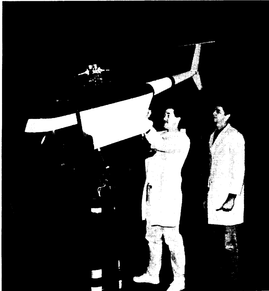
FIGURE 9: The Scaled Research Vehicle (FFRRV) In The NASA 14- by 22-Foot Tunnel.
