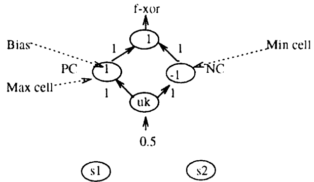
Figure 2: SC-net structure
