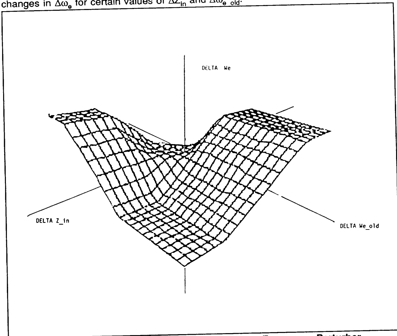
Figure 8. Control Surface for Synchronous Frequency Perturber
