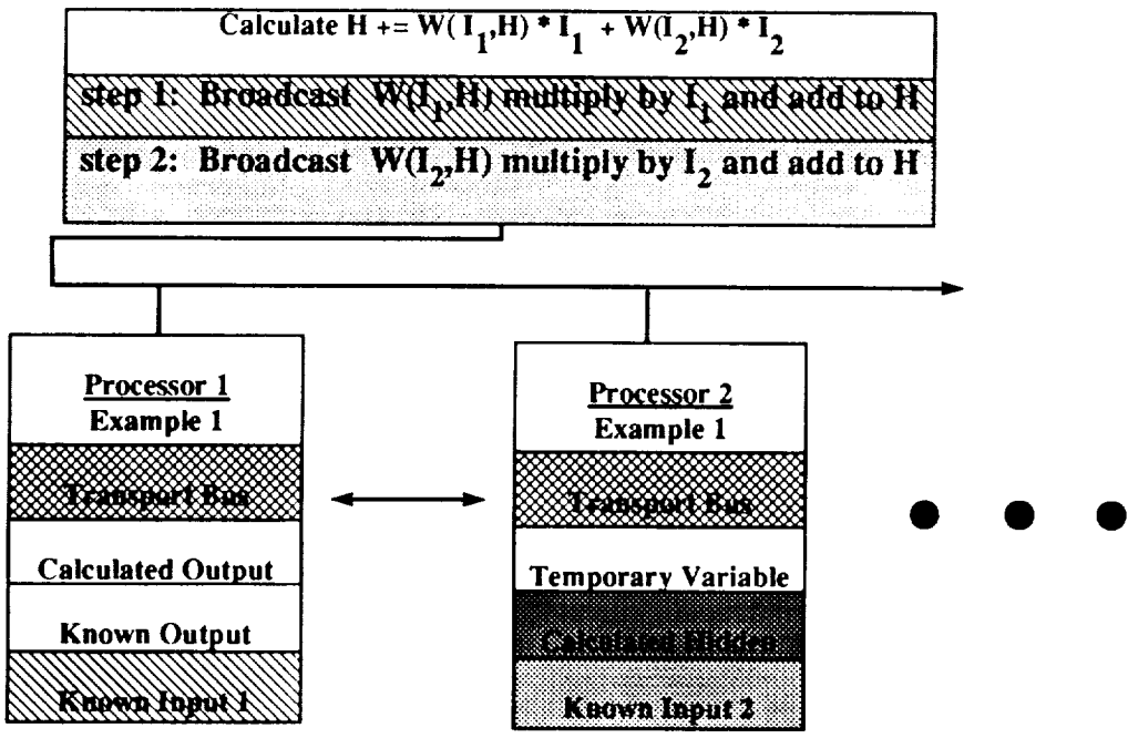
Fig 7: Calculation of Hidden Neuron (eqn 1.2) for XOR Network. All operations are local except for the global broadcast of the connections W(I_1,H) and W(I_2,H) and local inter-processor communications.
