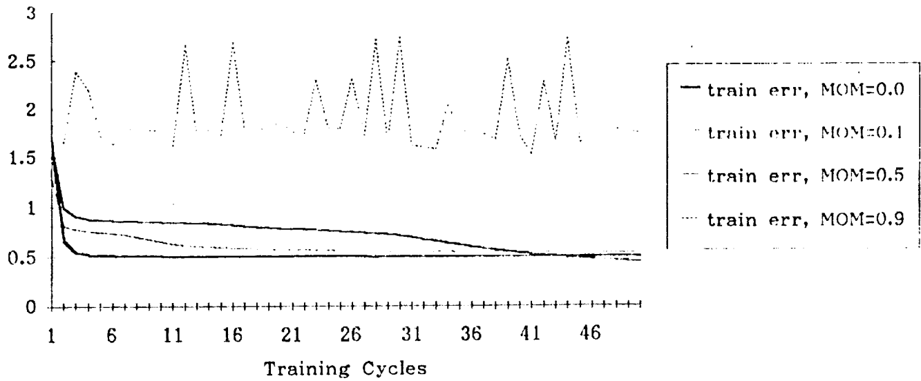
Training Error vs. Momentum Gain
