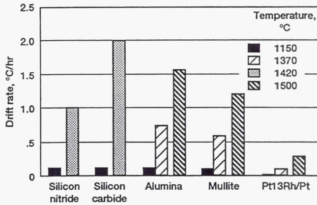
Figure 6.—Drift rates of 5 μm Pt13Rh/Pt thin film thermocouples and 75 μm lead wires at selected temperature levels.
