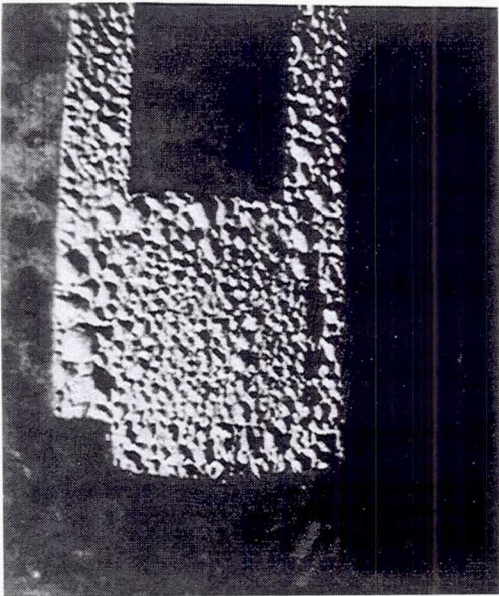
(c) Silicon nitride substrate—test time = 149 hours, maximum test temperature = 1167 °C.
