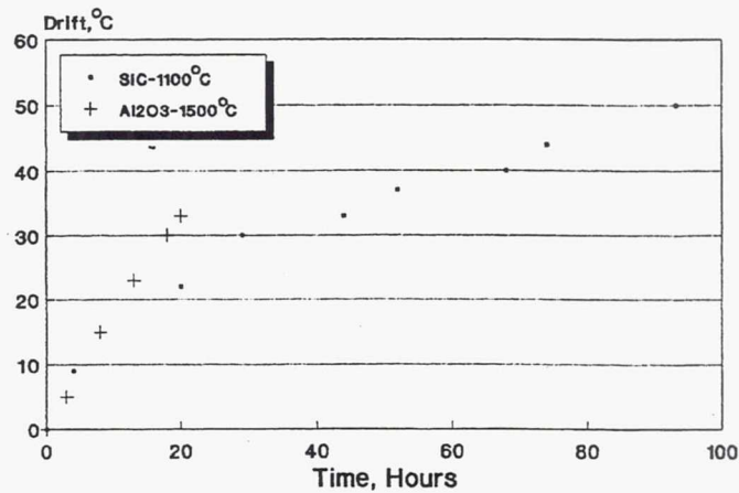
Figure 7.—Comparison of drift rates for Pt13Rh/Pt thin film thermocouples on silicon carbide at 1100 °C and aluminum oxide at 1500 °C.
