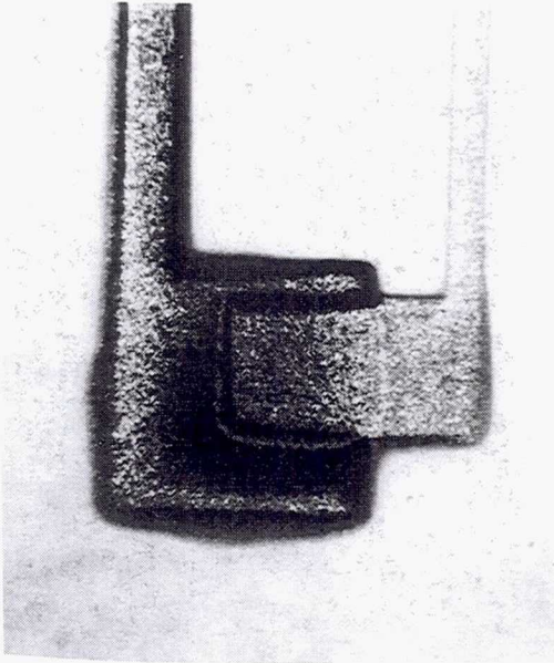
(a) Aluminum oxide substrate—test time = 38 hours, maximum test temperature = 1216 °C.
