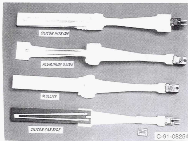
Figure 2.—Thin film Pt13Rh/Pt thermocouples on ceramic materials for high temperature furnace tests.
