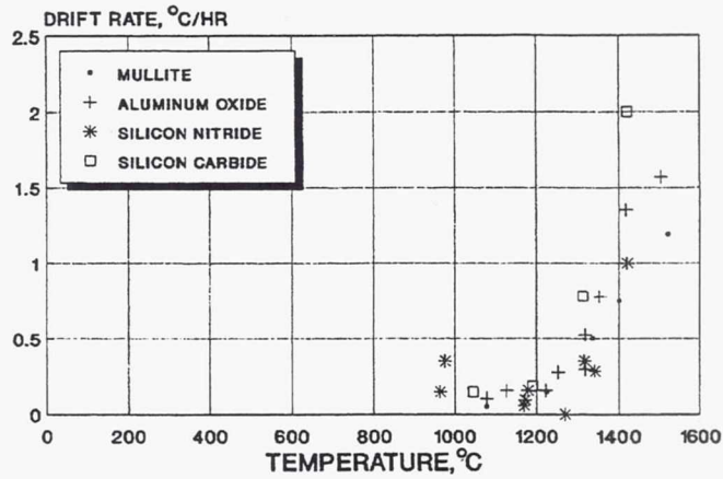
Figure 5.—Drift rates of Pt13Rh/Pt thin film thermocouples on ceramic substrates with 100 °C temperature gradient across thin film portion of thermocouple circuit.
