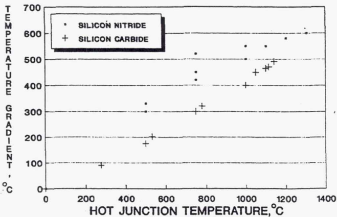
Figure 3.—Measurement of temperature gradient across thin film portion of thermocouple circuit on silicon carbide and silicon nitride substrates-high gradient configuration.
