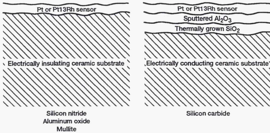
Figure 1.—Schematic diagram of thin film thermocouples on ceramic substrates.
