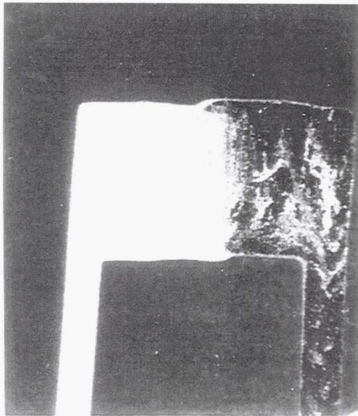
(c) Test time = 119 hours, maximum test temperature = 1246 °C.
