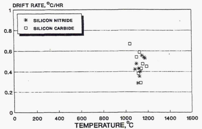
Figure 4.—Drift rates of Pt13Rh/Pt thin film thermocouples on ceramic substrates with 500-600 °C temperature gradient across thin film portion of thermocouple circuit.
