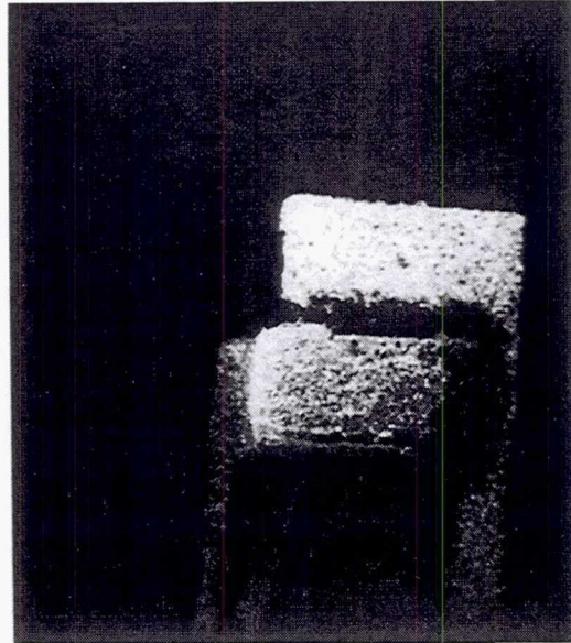
(b) Aluminum oxide substrate—test time = 94 hours, maximum test temperature = 1355 °C.
