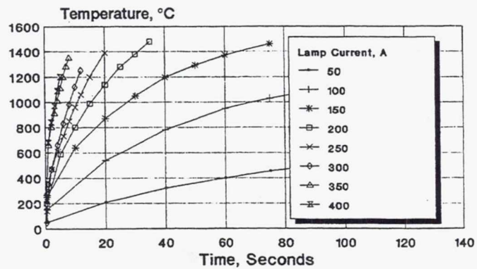
Figure 11.—Heating rate curves for Pt13Rh/Pt thin film thermocouples on silicon nitride substrate in arc lamp heat-flux-calibrator test.
