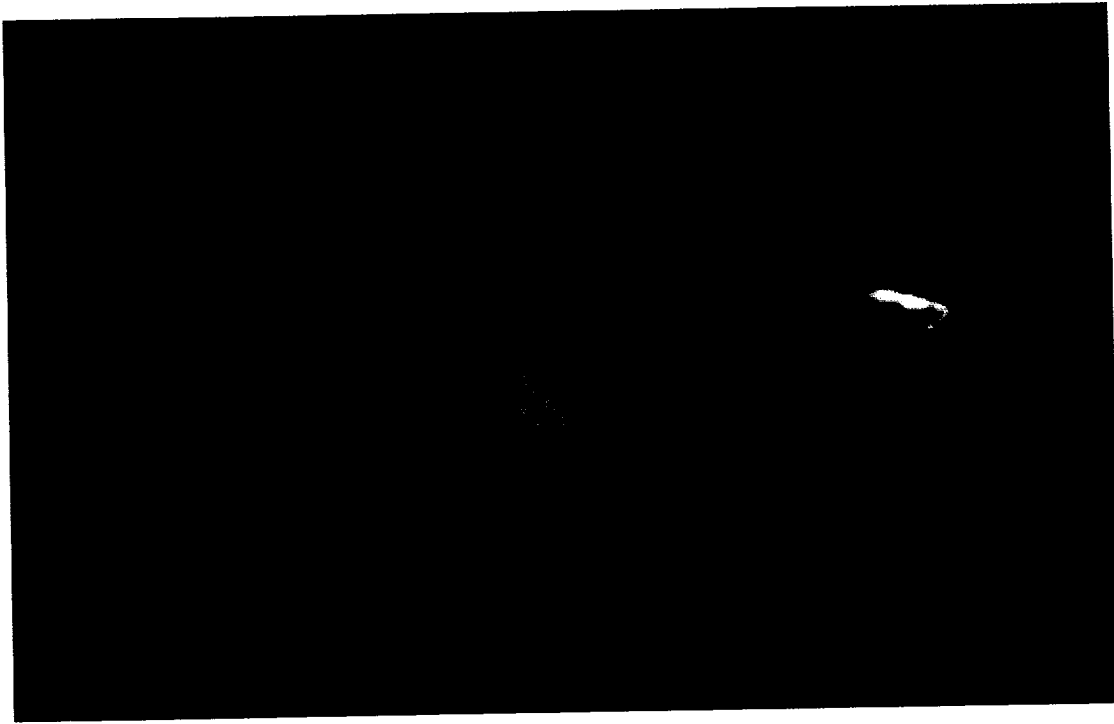
Figure 1. Space Shuttle glows produced during STS-39 by nitric oxide (NO) chemical releases within Discovery's cargo bay. Surface and gas-phase glows are visible in the photograph.
