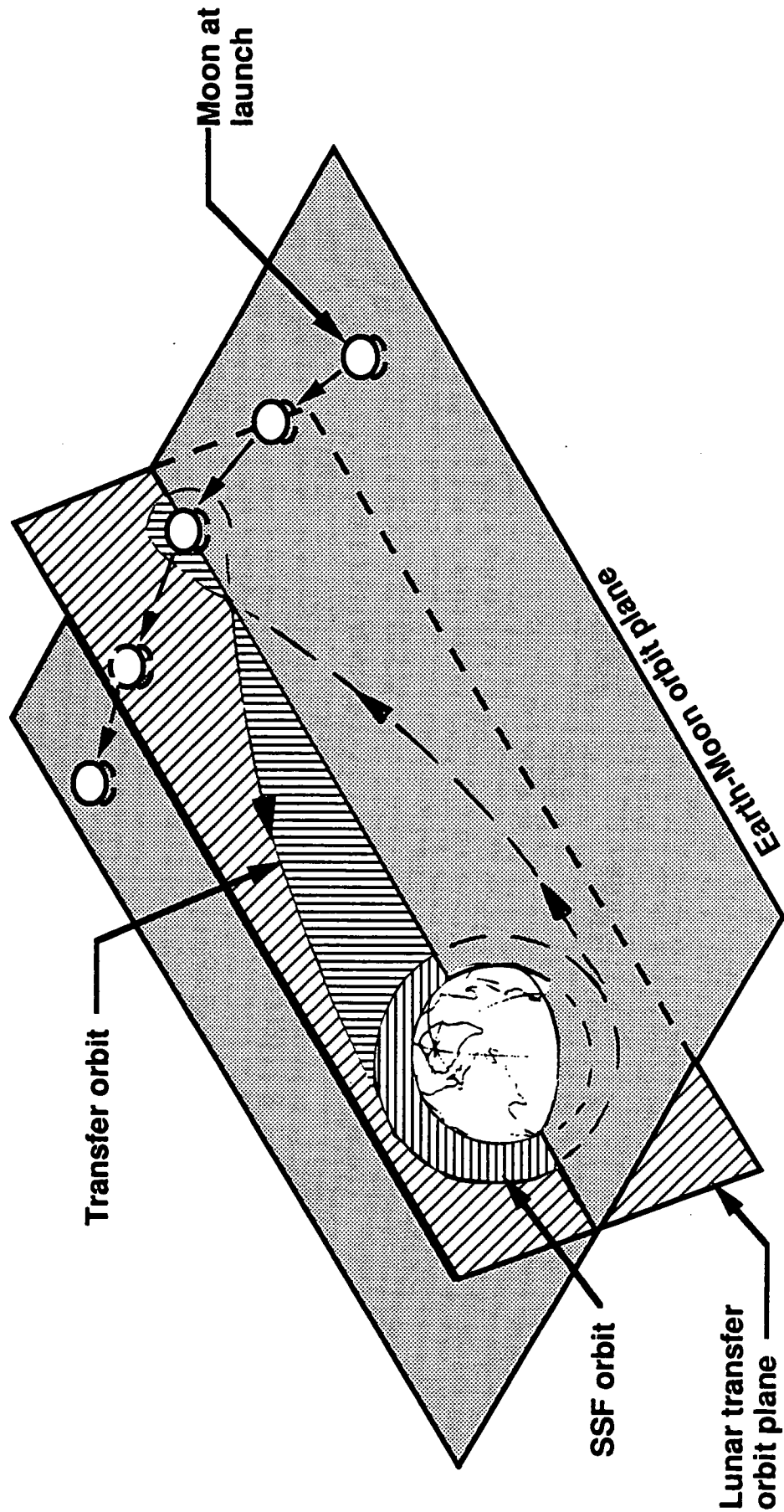
Figure 2-1.3-2. Lunar Transfer Geometry From SSF
