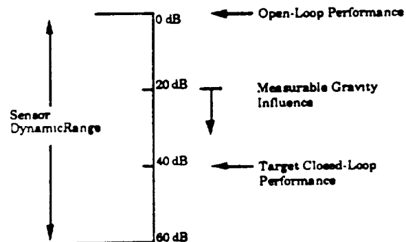
Figure 2 MACE Test Article Requirement
