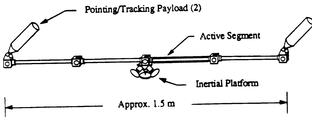
Figure 6: The MACE flexible test article.
