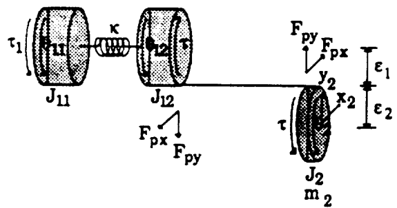
Figure 8 Flexible evaluation model for non-CG mounted payload.
