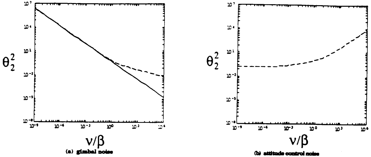
Figure 6 Variance of CG mounted payload under white noise applied at the gimbal and attitude control location for centralized configuration. The values of J_1=1, J_2=0.5 and \mu=1 were used.
