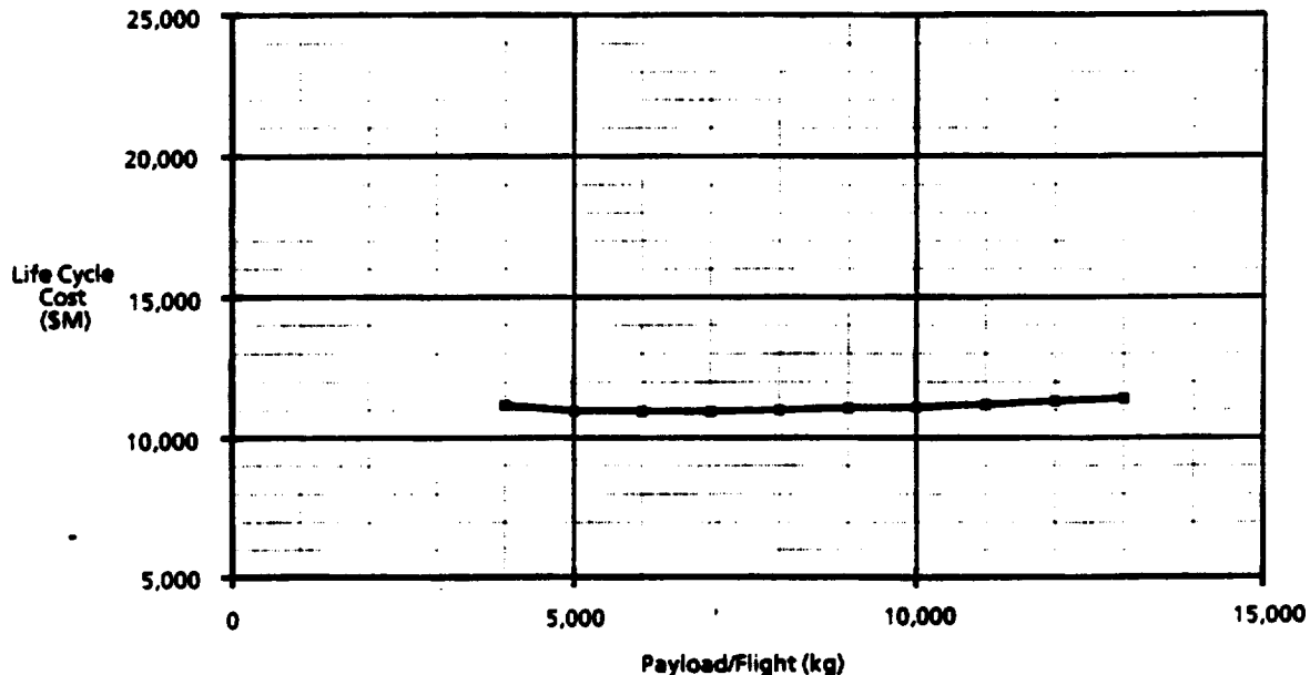
Figure 2.8. Life Cycle Cost vs. Payload Size
