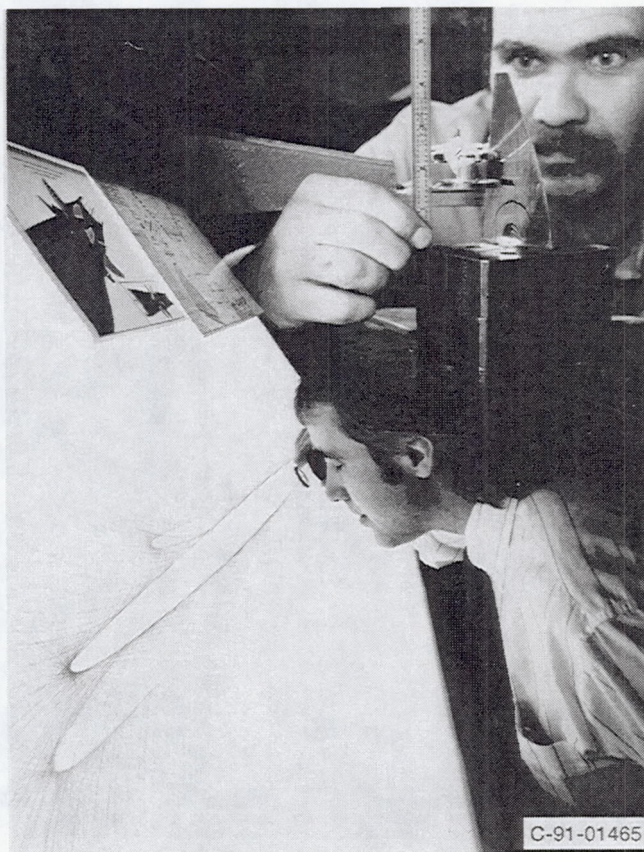
Figure 24.—Blade in inspection machine, upper right. Cross-sectional tracing being compared with Mylar master, lower left.
