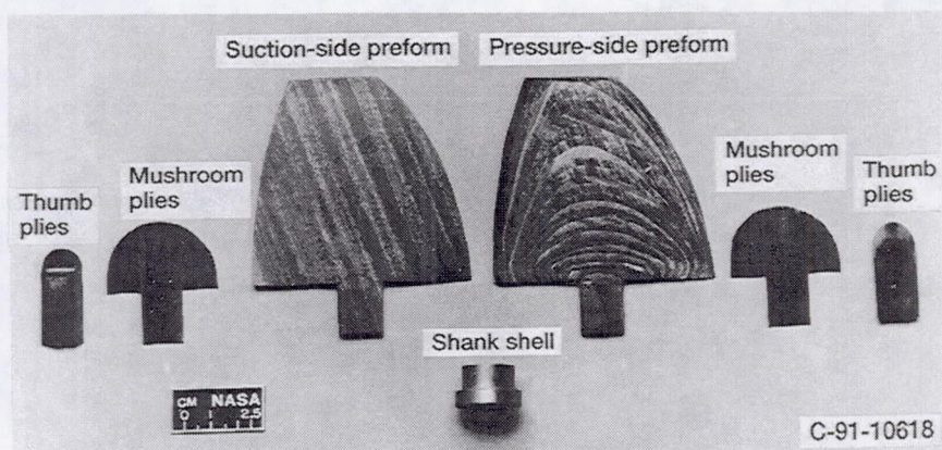
Figure 3.—Components used to assemble a CM-2D blade.
