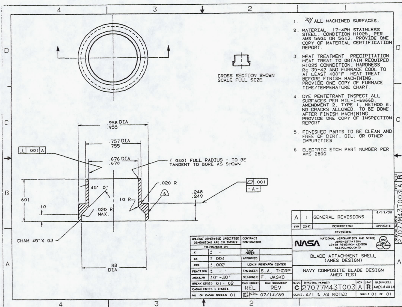
Figure 19.—Drawing for metal shell used at base of composite blade.
