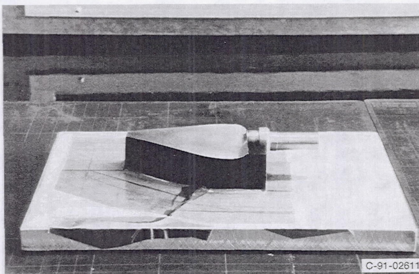
Figure 13.—Completed male half of mold for CM-1D forward blade.
