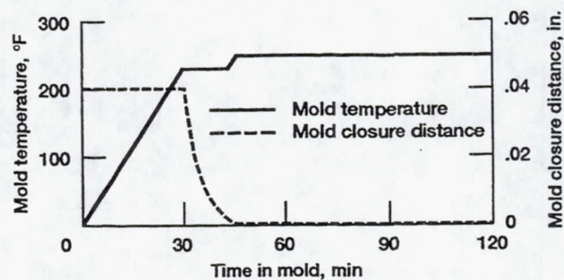
Figure 23.—Chart showing mold parameters used for CM-1D and CM-2D blades.
