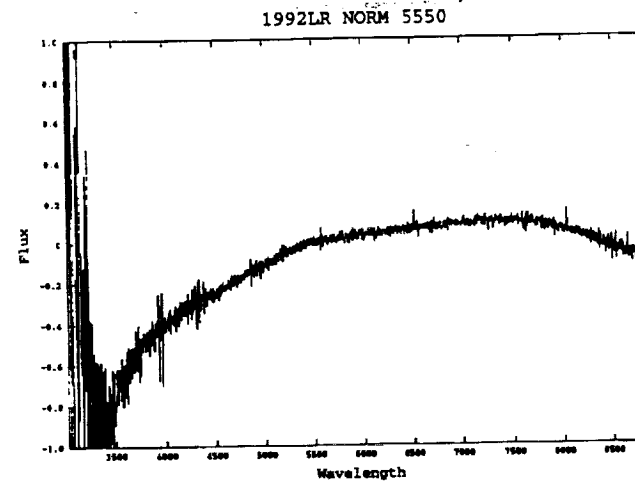
Figure 1. Spectra of 3 NEOs obtained using the 4.2m Herschel telescope on La Palma. As seen in part (a), 1992AC shows the characteristically flat spectra for an EMP type, while 1992JE, part (b), has the slightly more curved signature of the C-type asteroid. 1992LR, part (c), shows the flattening toward the red end of the spectrum characteristic of an S-type asteroid.
