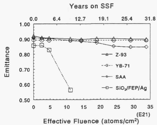
Figure 3b: Thermal emittance of RF plasma ashed coatings.
