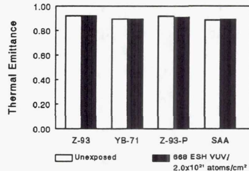
Figure 6b: Thermal emittance of ECR beam/VUV lamp exposed coatings.
