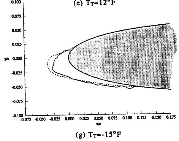
Fig. 9. Effect of Total Air Temperature on Ice Shape.
