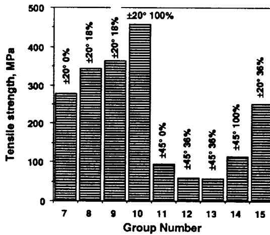
Fig. 31. Strength of Flight Specimens
