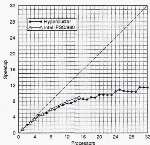
Figure 5: ISTAGE speedup
