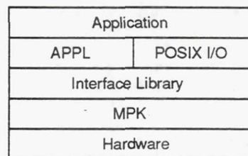
Figure 4: Software layers
