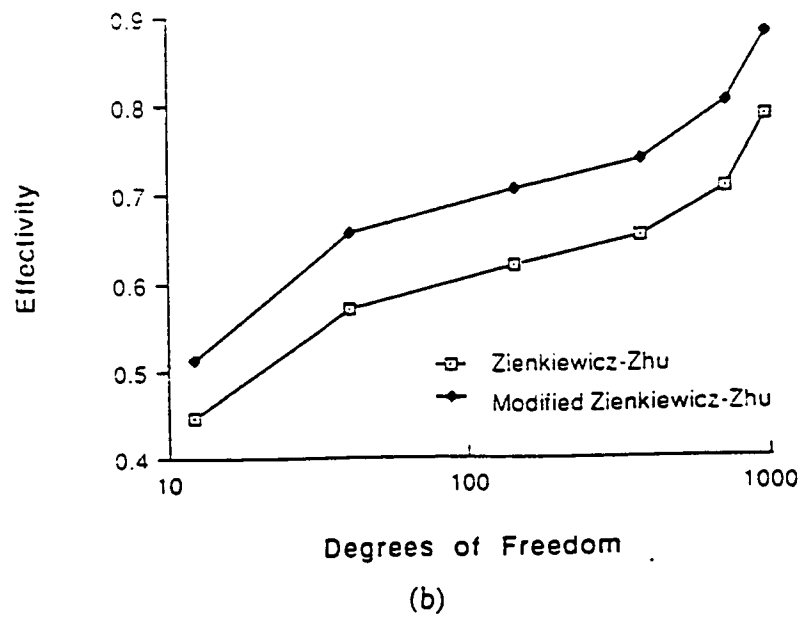
Figure 3.67: (a) Exact error and two error estimates for the six meshes of the cantilever beam problem. (b) Effectivity indices of the two estimates.
