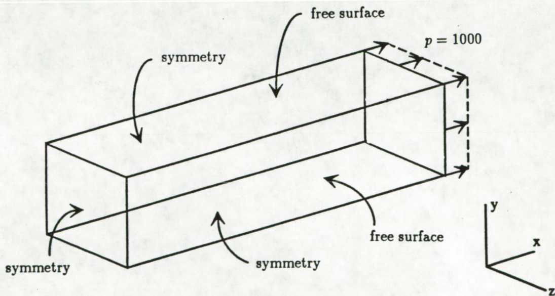
Figure 5.14: Geometry and boundary conditions for isotropic bar under simple tension
