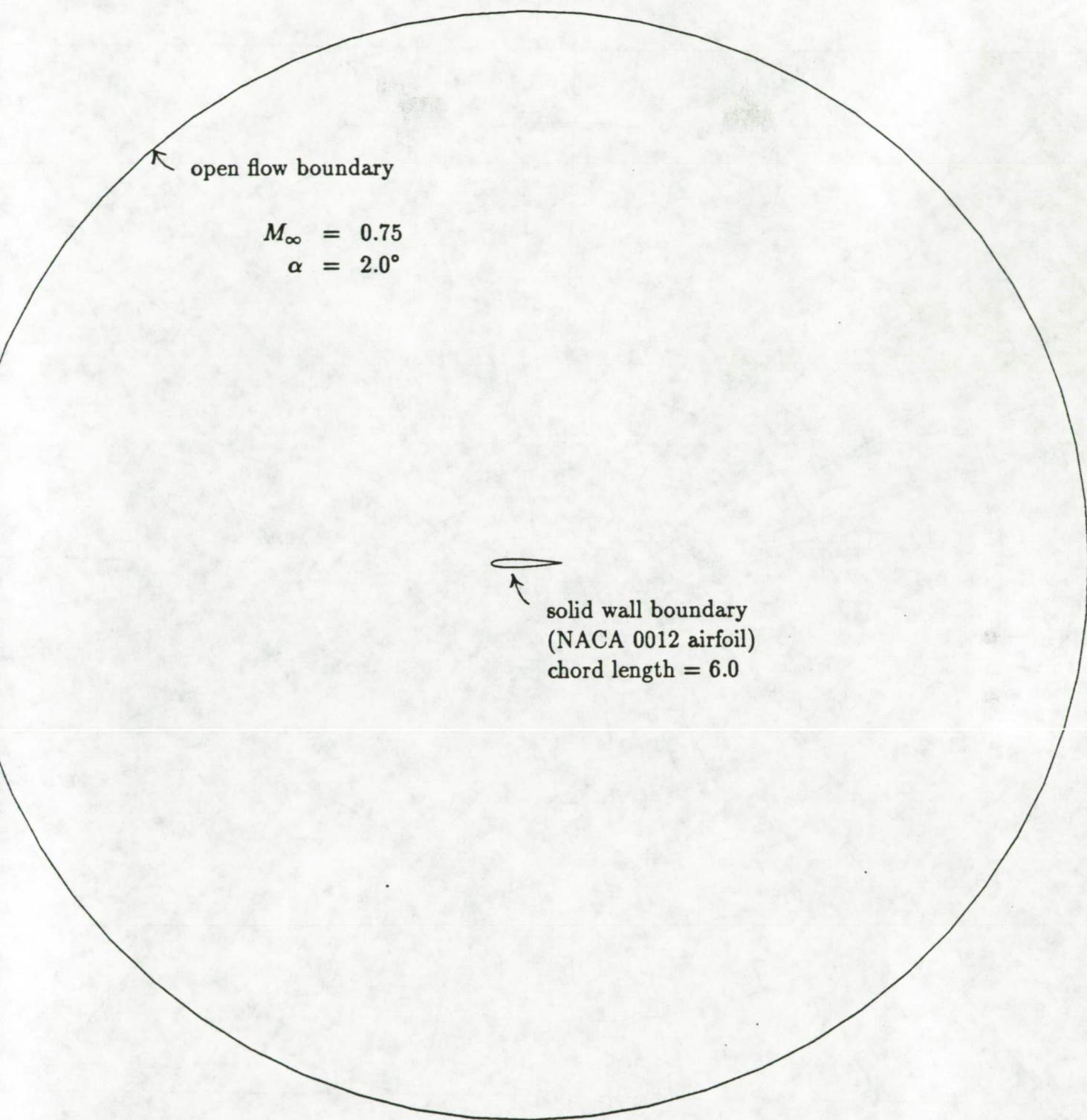
Figure 5.40: Geometry and boundary conditions for inviscid flow over a two-dimensional airfoil
