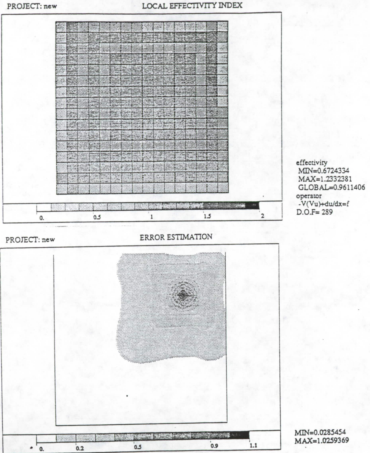
Figure 3.58: Local effectivity indices and estimated error for example with polynomial solution using the governing equation:
