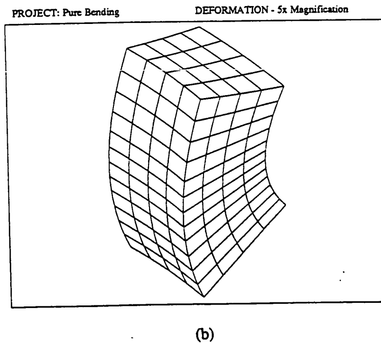
Figure 3.50: Pure bending of a prismatic beam. (a) Beam with applied moment, (b) deformed shape of beam (magnified five times).
