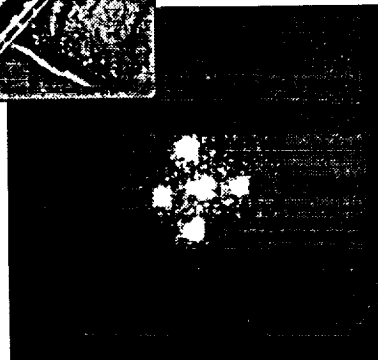
Einstein's Cross
