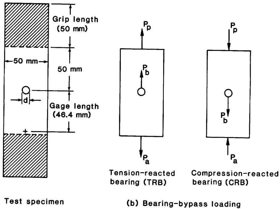
Figure 1. Specimen configuration and bearing-bypass loading.
