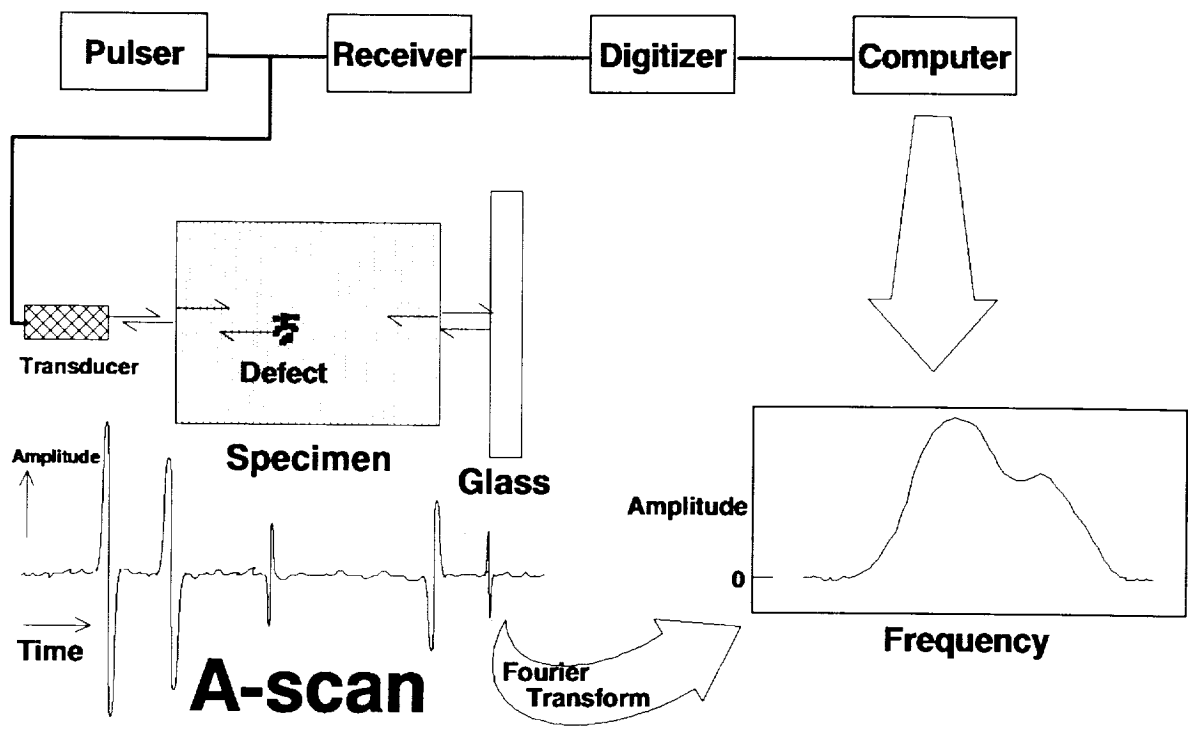
Figure 4 - Diagram of ultrasonic data acquisition system.
