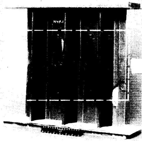
Failed panel specimen NYP1
