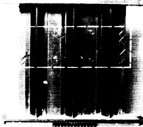
Failed panel specimen NYP2
