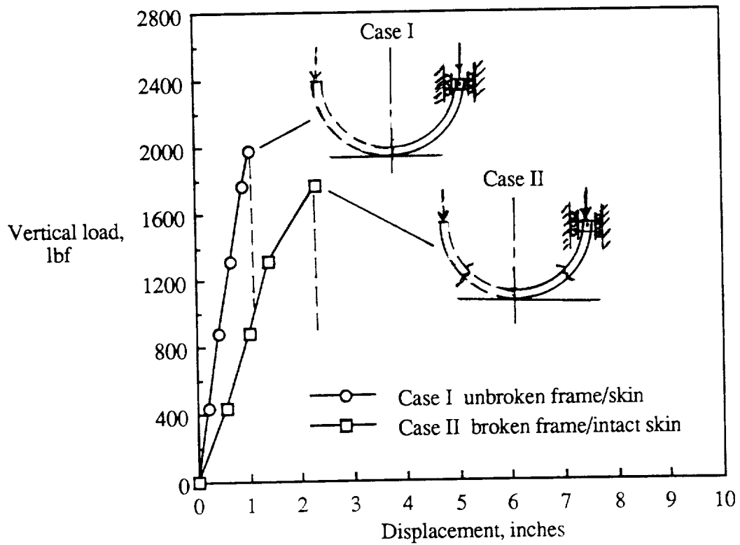
(a) Load-displacement.
