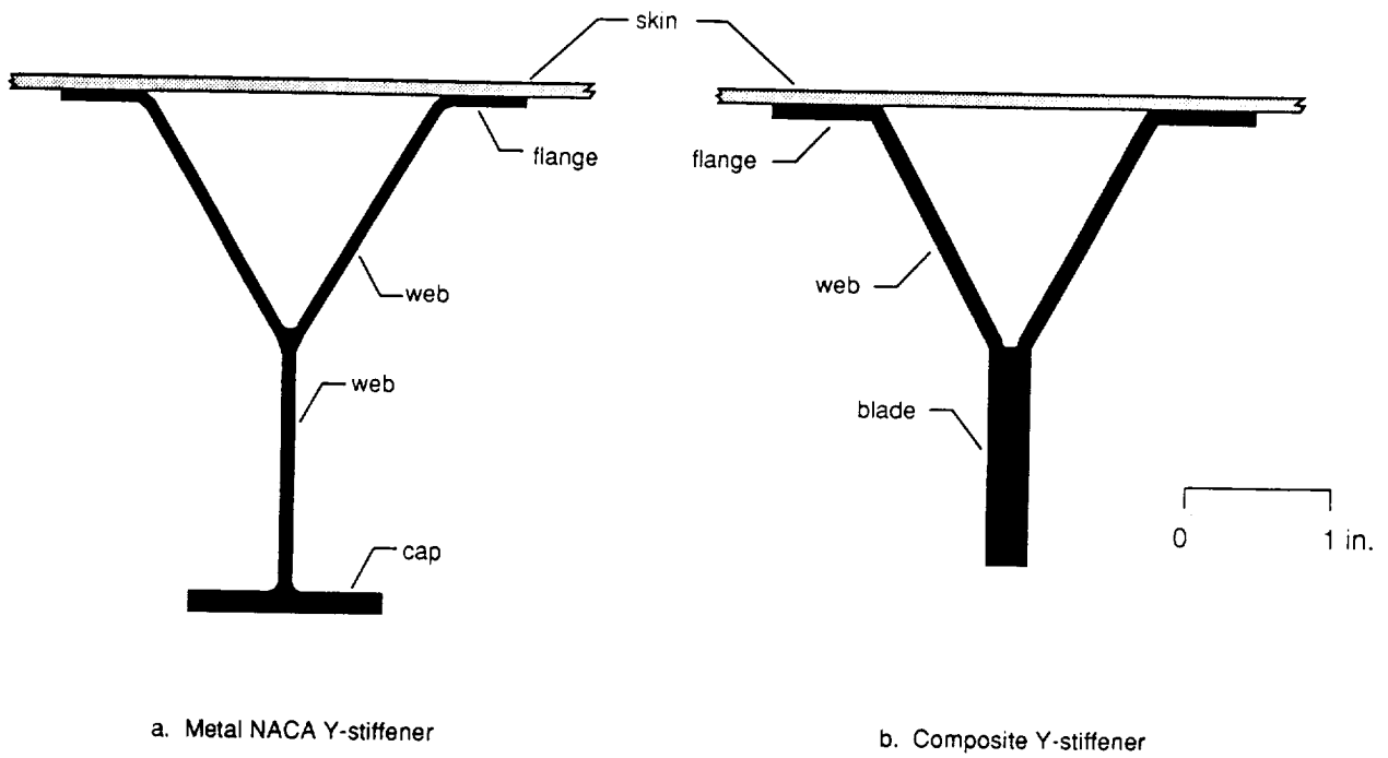
Figure 1. Y-Stiffener Configurations.
