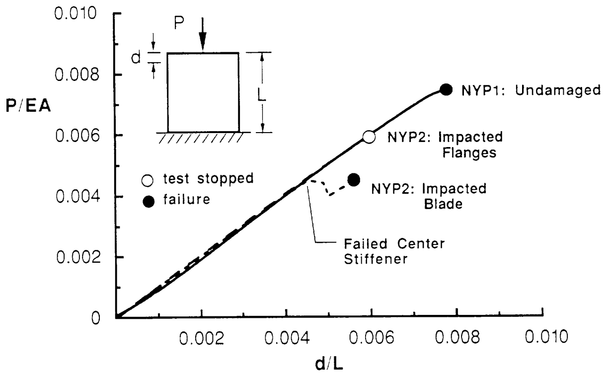
Figure 10. Normalized load versus end-shortening for Y-stiffened panel specimens.
