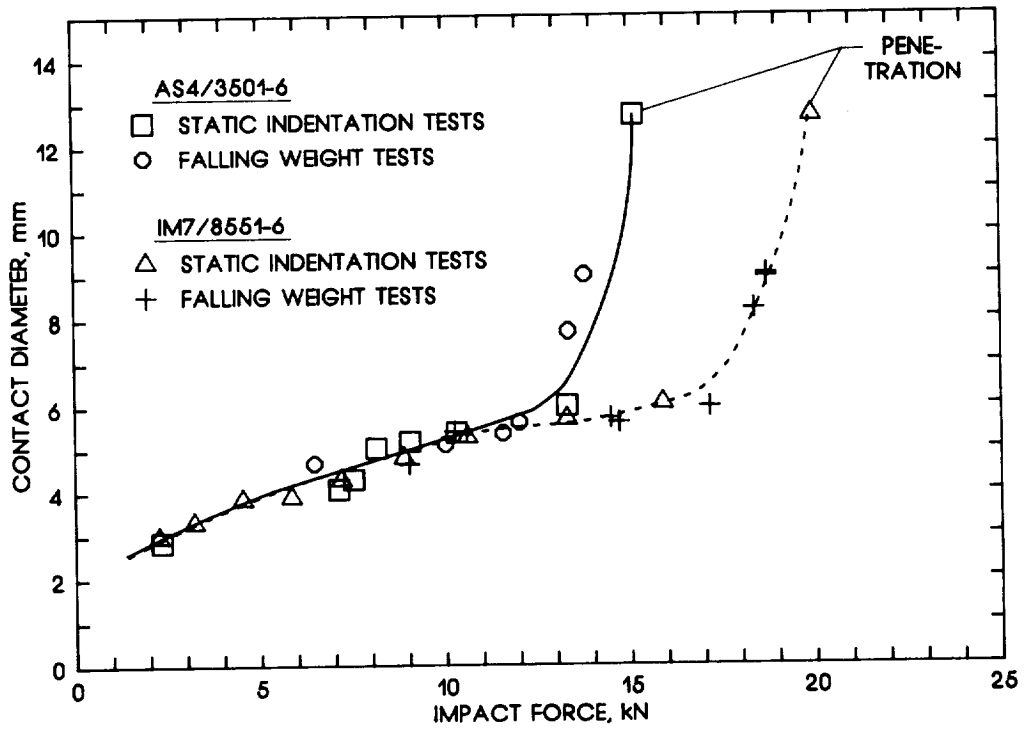
Figure 16.- Contact diameter versus impact force for [45/0/-45/0/90]_{6S} tape laminates.
