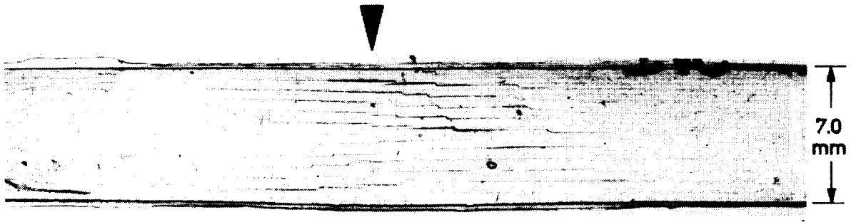
Figure 7.- Photograph of edge replica of IM7/8551-7 specimen (D051R) impacted by falling weight with kinetic energy of 27.1 J.
