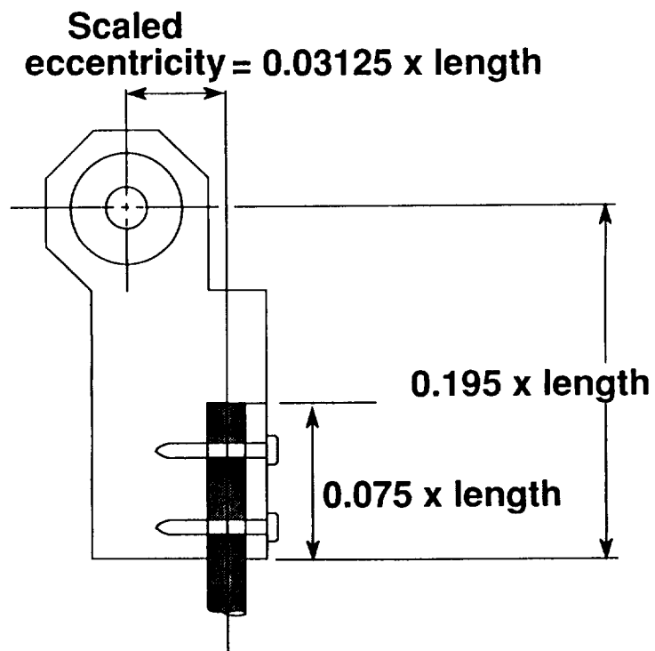
FIGURE 2. Detailed drawing of the hinge-beam attachment.
