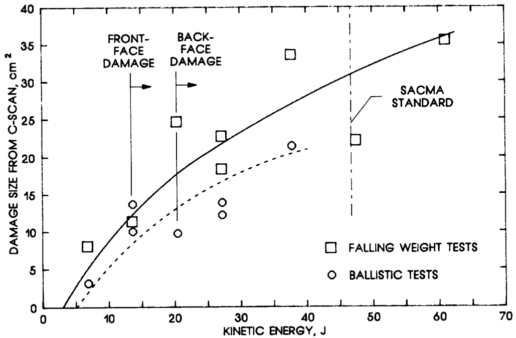
(a) [45/0/-45/90] 66 AS4/3501-6 laminate.
