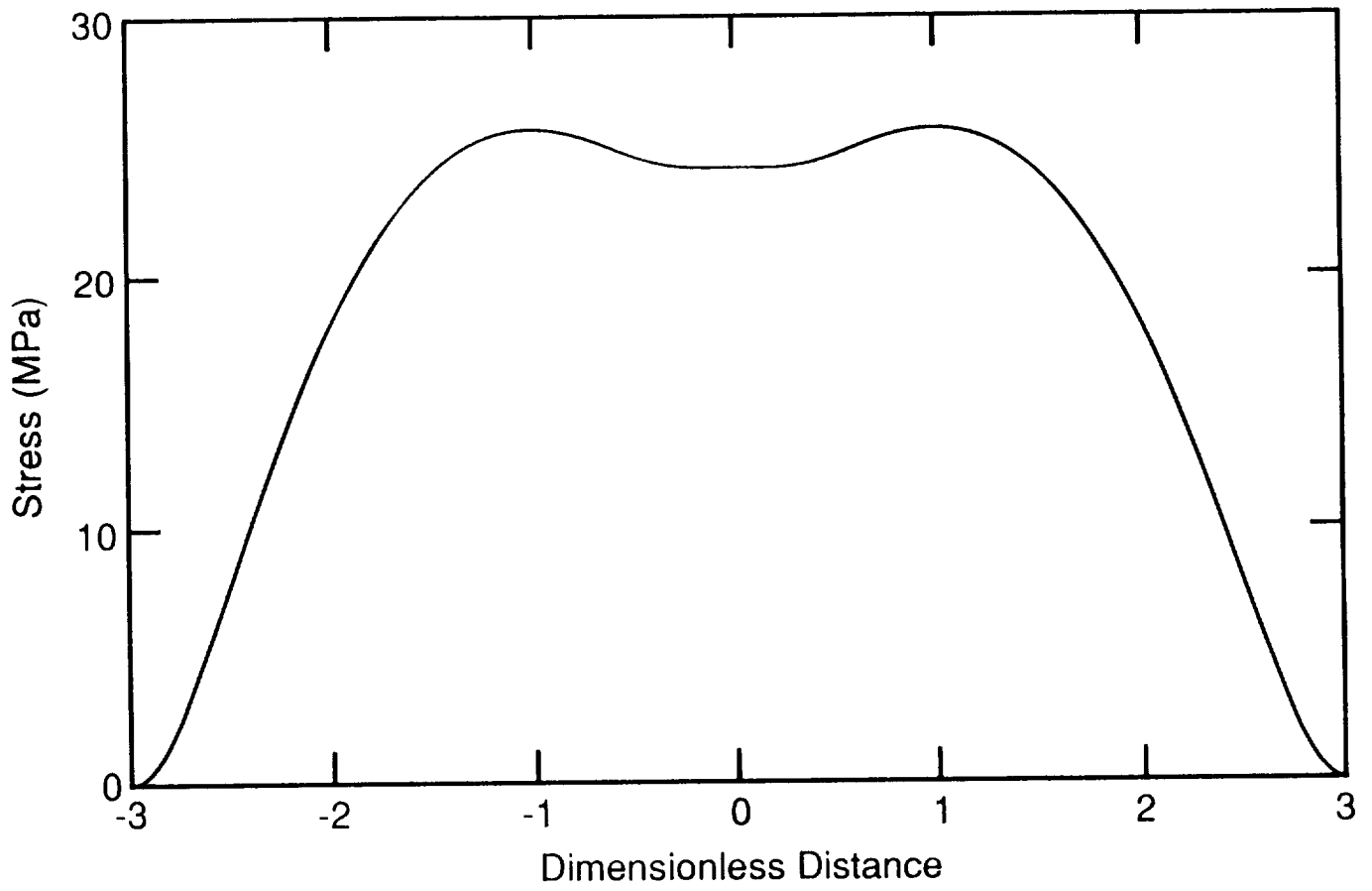
Figure 4: The x direction tensile stress in the 90^\circ ply in a [90_2/0] , carbon fiber/epoxy laminate ( \sigma_{xx}^{(1)} ). This ply has microcracks located at \rho = \pm 3 .
