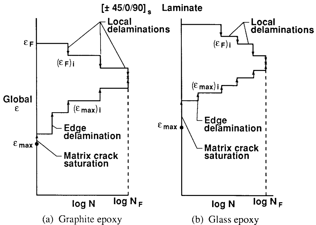
Figure 8. Damage-threshold/fail-safety analysis.
