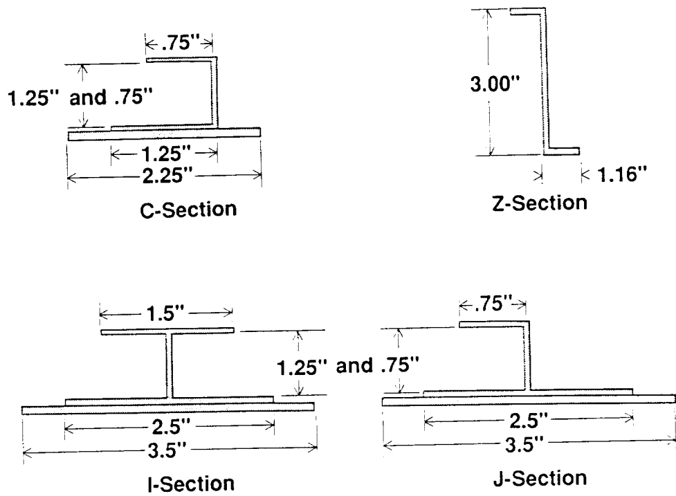
(a) Cross-sectional dimensions.
