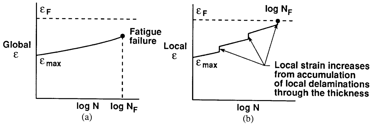
Figure 3. Increase in global versus local strain in 0^\circ plies.
