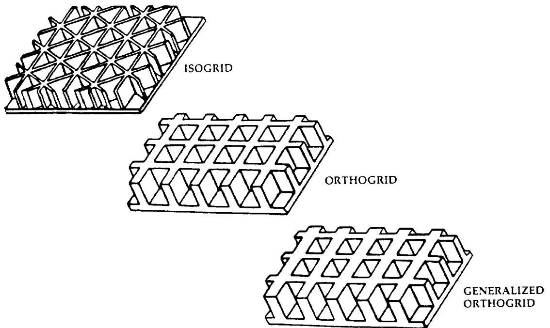
FIGURE 3. - GRID CONFIGURATIONS
