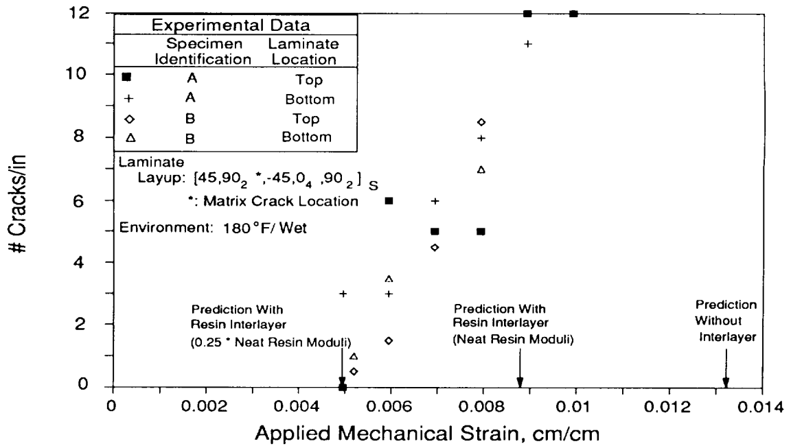
Figure 5. Matrix Crack Onset Predictions and Test Data for a Laminate Exposed to 180^\circ\text{F/Wet} .
