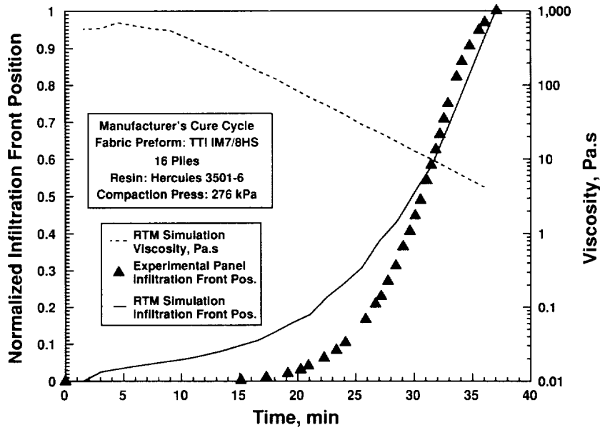
Figure 9. Normalized infiltration front as a function of time.
