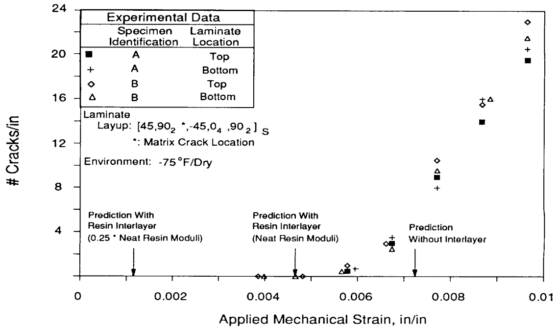
Figure 4. Matrix Crack Onset Predictions and Test Data for a Laminate Exposed to -75^\circ\text{F/Dry} .
