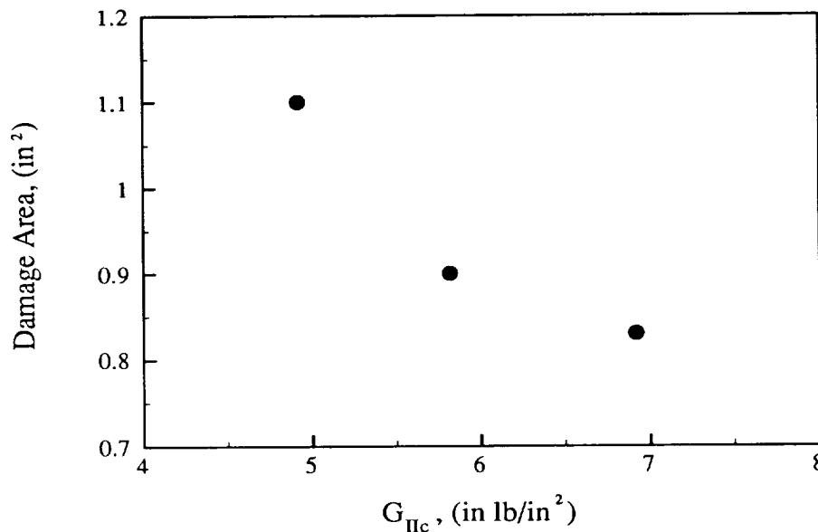
Figure 8. Relationship Between Impact Damage Area and G_{IIc} for IM7/8551-7
