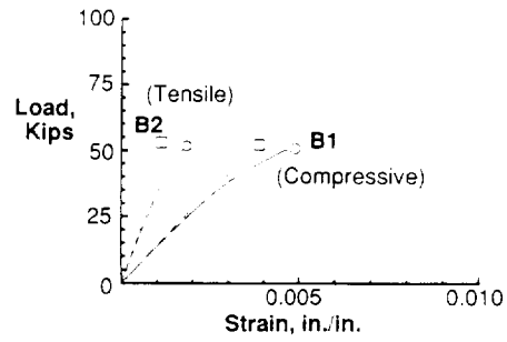
c. strain in web
