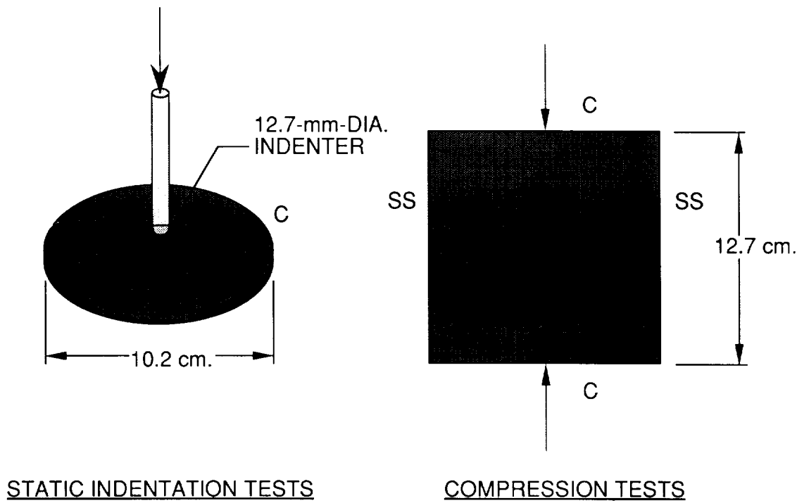
Figure 1. - Static indentation and compression tests.
