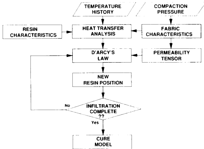
Figure 5. RTM simulation model.
