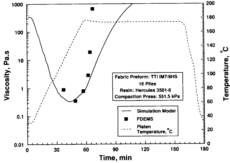
Figure 13. Resin viscosity as a function of time at the bottom of the fabric preform. Comparison between FDEMS measured and model calculated values of resin viscosity.
