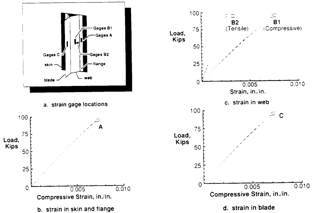
Figure 6. Strain gage results for undamaged element specimen NY1 (square and circular symbols used to distinguish between individual gages).
