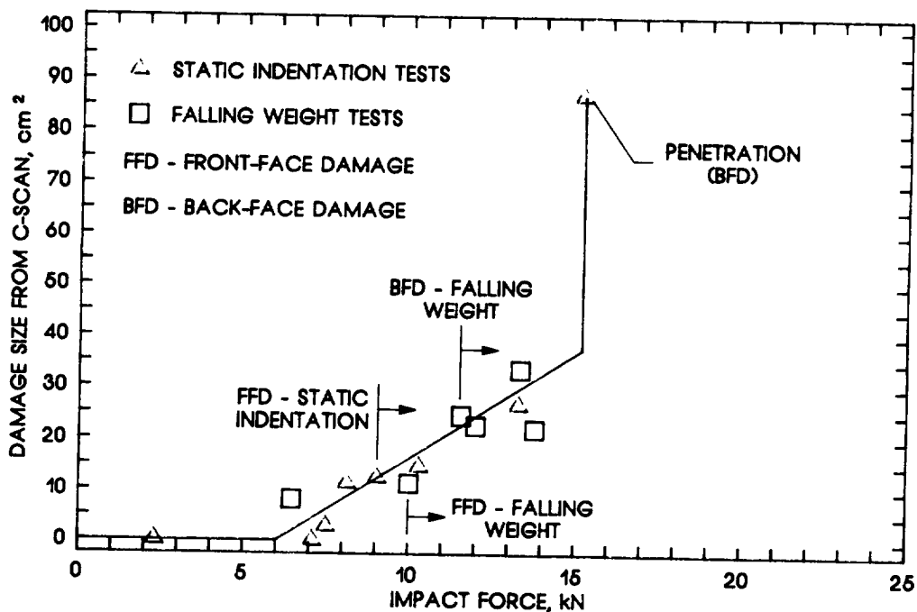
(a) [45/0/-45/90] ss AS4/3501-6 laminate.
