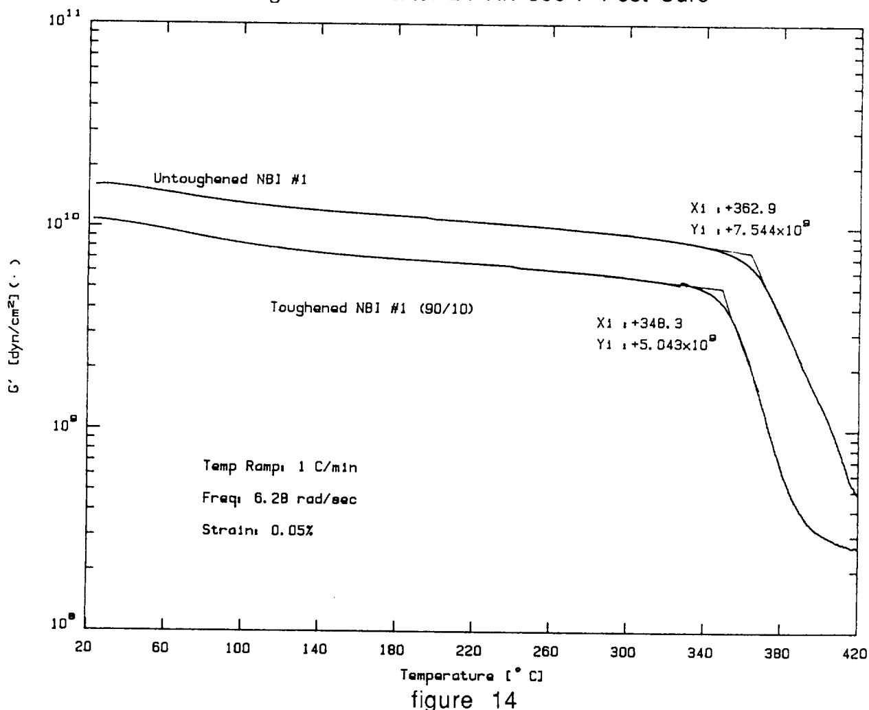
Thermal Profile of Untoughened vs. Toughened PI after 24 Hr. 600°F Post Cure
