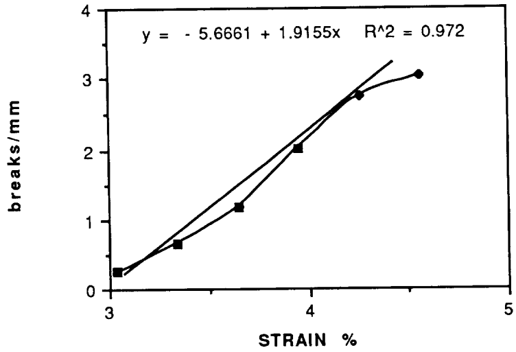
Figure 5 - Fragmentation of the AS4G fiber in tension.
