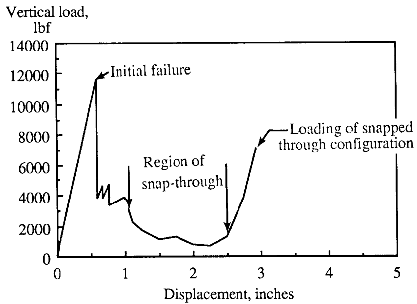
(a) Load-displacement.
