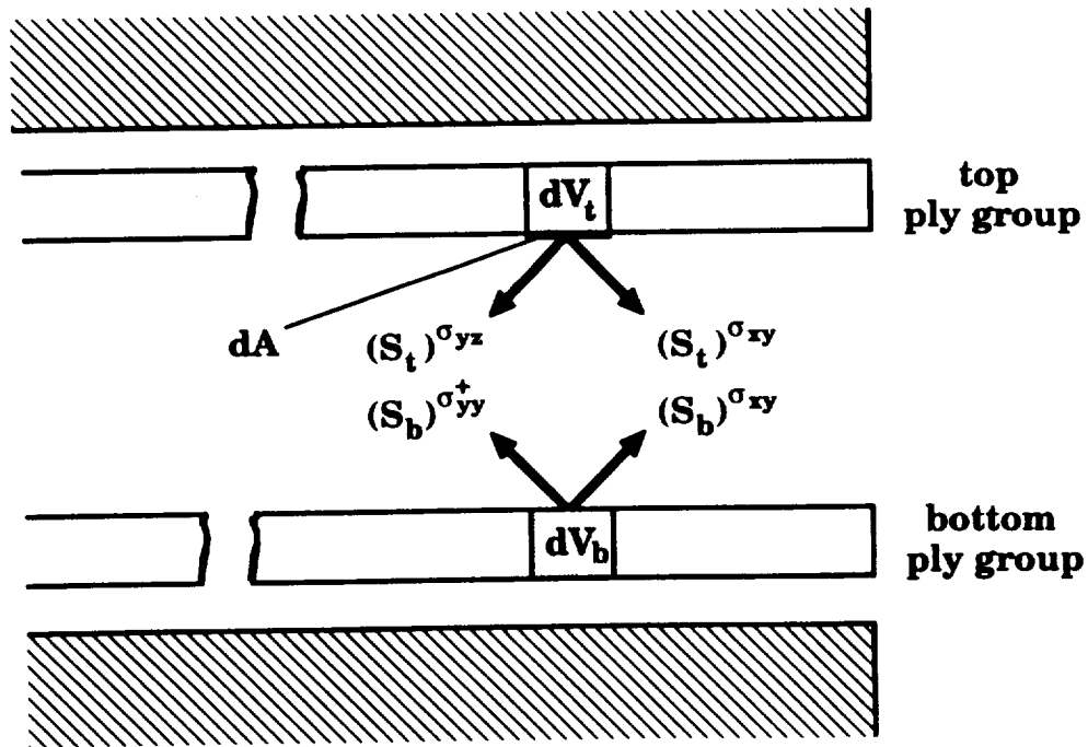
Figure 11 Stresses from the top and bottom cracked ply groups contributing to the strain energy available to form a delamination
