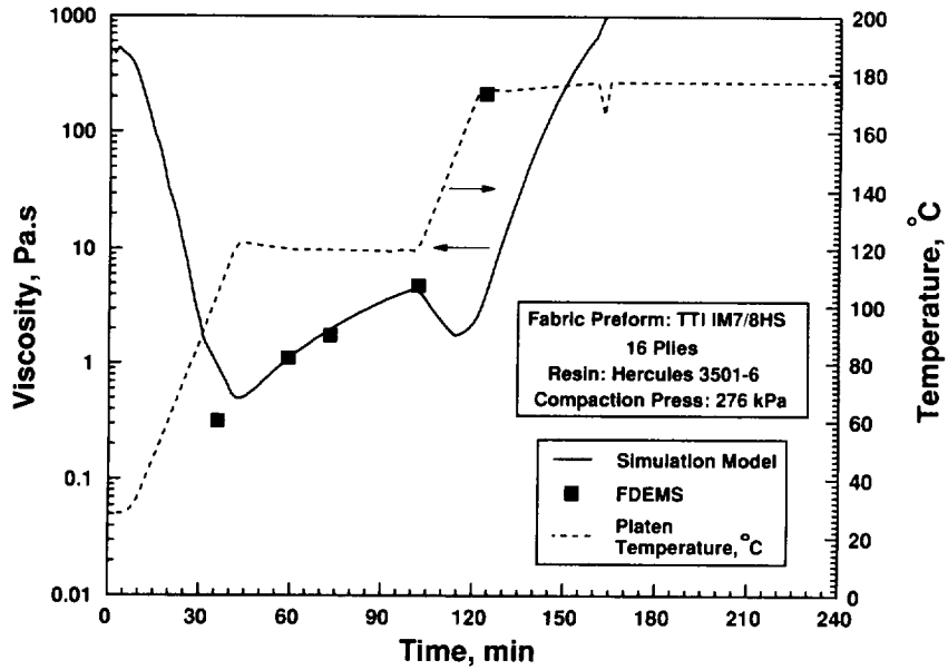
Figure 11. Resin viscosity as a function of time at the bottom of the fabric preform. Comparison between FDEMS measured and model calculated values of resin viscosity.
