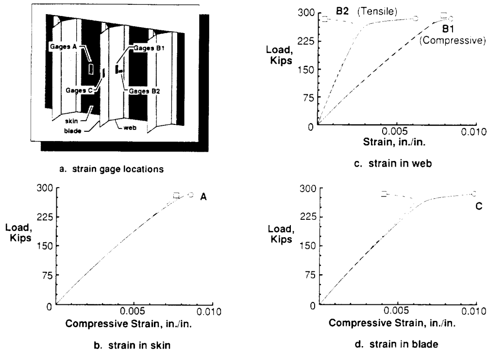
Figure 12. Strain gage results for undamaged panel specimen NYP1 (square and circular symbols used to distinguish between individual gages).
