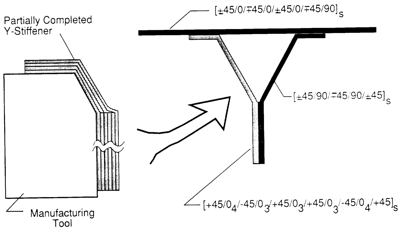
Figure 2. Fabrication of Composite Y-Stiffened Element.
