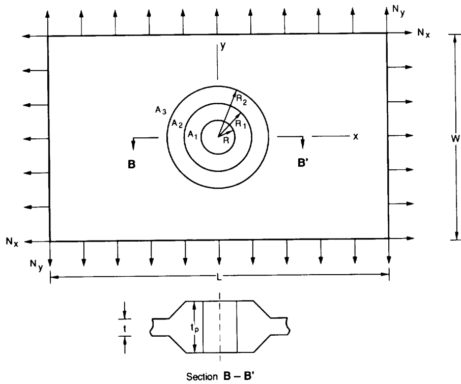
Figure 2. Symmetric integral padup around a circular hole.
