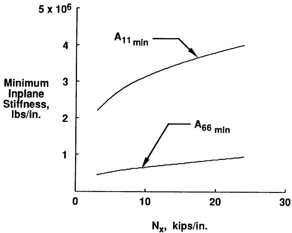
Figure 3. Minimum required inplane stiffnesses for cover panels [11]
