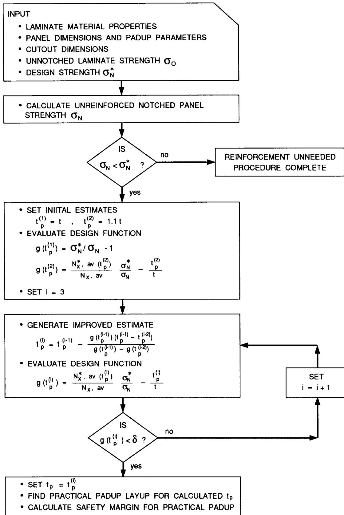
Figure 8. Flowchart for Padup Design Procedure.
