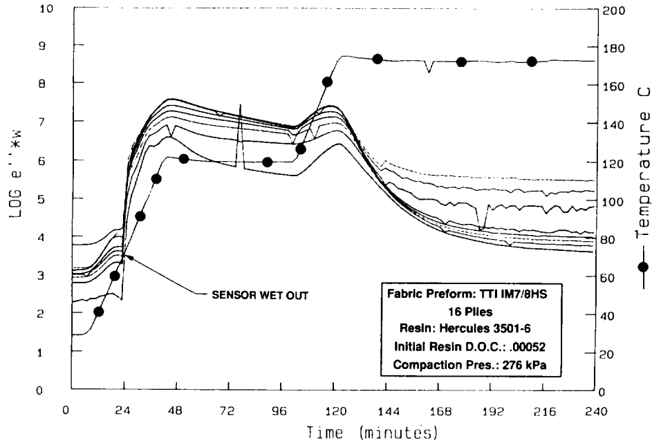
Figure 7. Values of \epsilon'' multiplied by frequency ( \epsilon'' \cdot \omega ) for the bottom sensor. Constant frequency lines plotted from bottom to top are 50 Hz, 125 Hz, 250 Hz, 500 Hz, 5 kHz, 25 kHz, 50 kHz, 0.25 MHz, and 0.50 MHz. Wet out of sensor occurs at 26 minutes.
