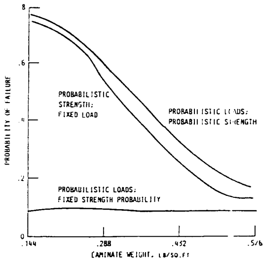
Figure 10. Laminate Optimum Weight For Specified Reliability.
