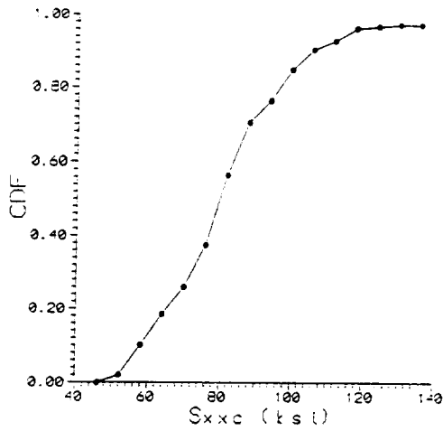
Figure 7. Longitudinal Compressive Strength of a Quasi-Isotropic Laminate (Graphite Fiber-Epoxy)
