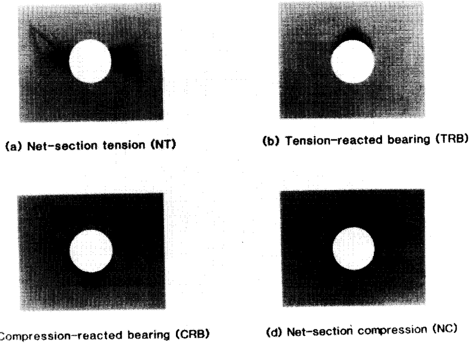
Figure 3. Radiographs of damage at fastener hole.
