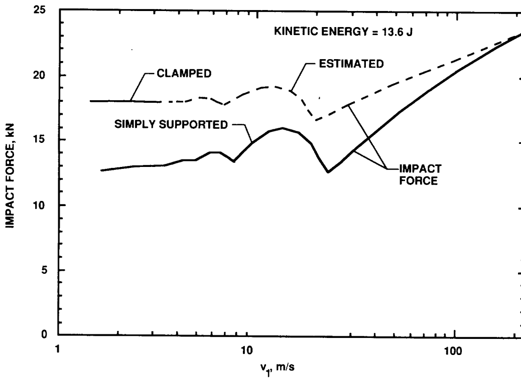
Figure 23.- Predicted impact force versus impactor velocity.
