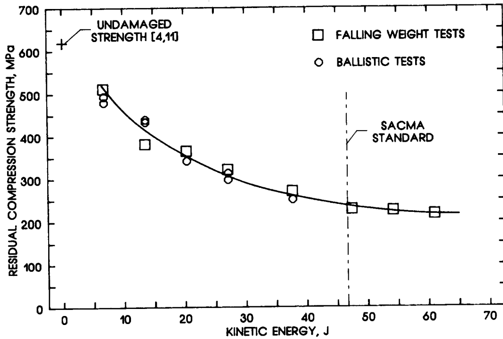
(b) [45/0/-45/90] 68 IM7/8554-7 laminate.
