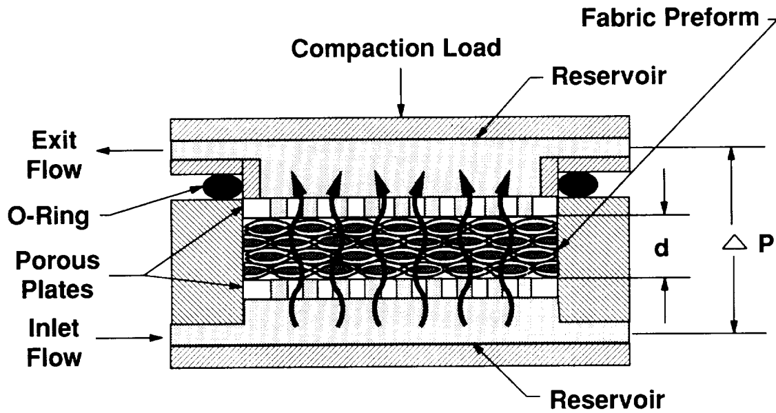
Figure 2. Schematic of the permeability test fixture.
