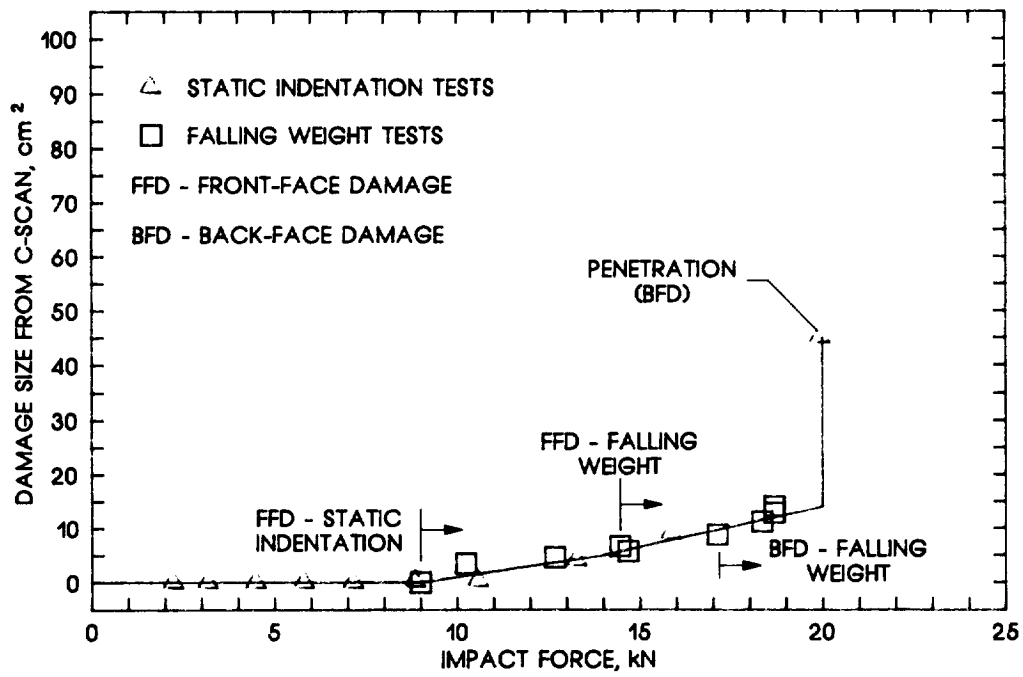
(b) [45/0/-45/90] 68 IM7/8554-7 laminate.
