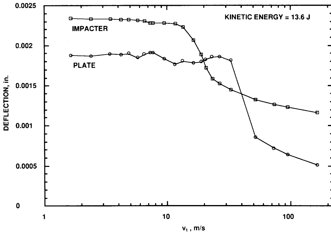
Figure 21. Predicted maximum deflection at center of plate versus impact velocity.
