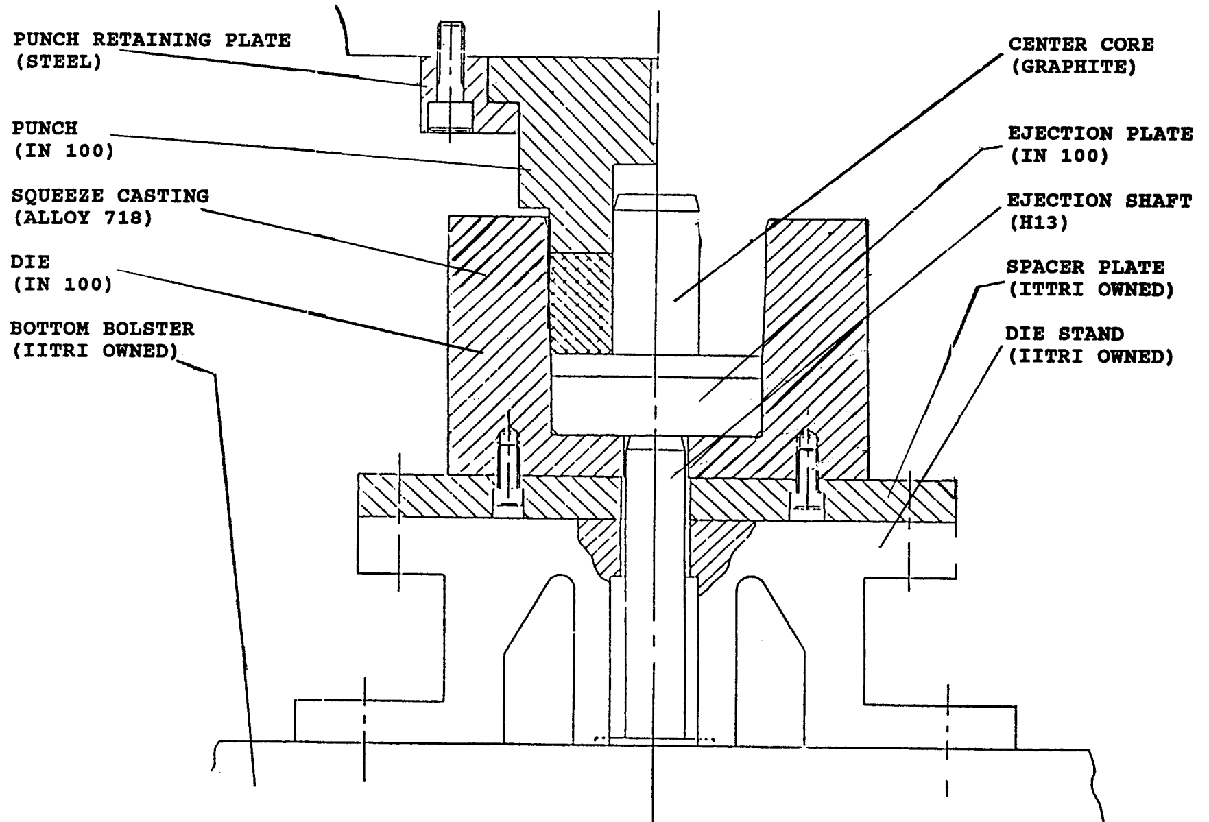
Figure 2. Die system components and materials.
