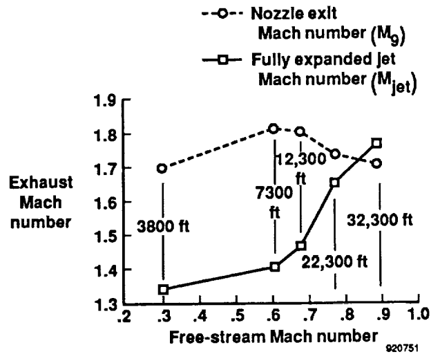
Figure 7. Climb-to-cruise exhaust Mach number test points for an F-18 aircraft at intermediate power.
