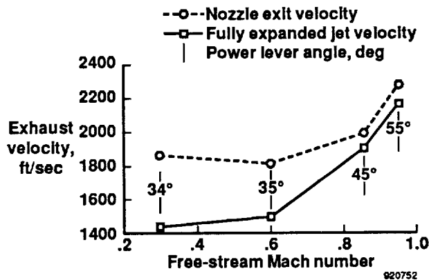
Figure 8. Aircraft Noise Prediction Program validation exhaust velocity test points for an F-16XL, ship 2, aircraft.
