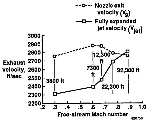
Figure 6. Climb-to-cruise exhaust velocity test points for an F-18 aircraft at intermediate power.
