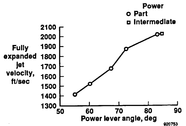
Figure 9. Fully expanded jet velocity for ground test points of an F-16XL, ship 2, aircraft at an altitude of 2300 ft and at Mach 0.
