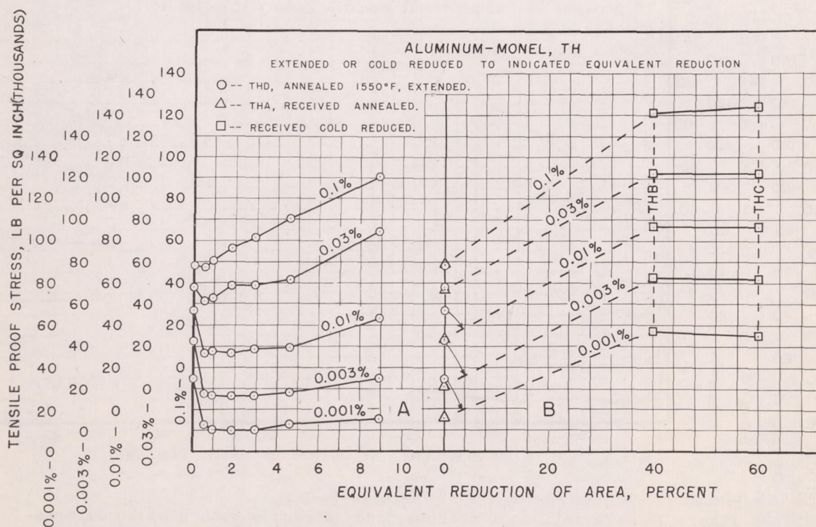
Figure 11.- Variation of tensile proof stress with plastic deformation for aluminum-monel tubing TH. A-Aluminum-monel THD, annealed and extended. B-Cold-reduced aluminum-monel.
