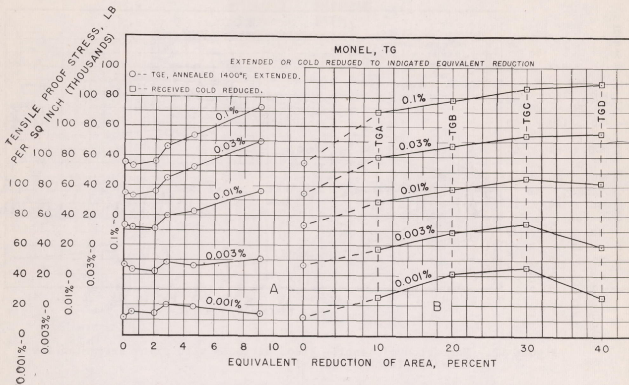
Figure 10.- Variation of tensile proof stresses with prior deformation for monel tubing TG. A-Monel TGE, annealed and extended. B-Cold-reduced monel.
