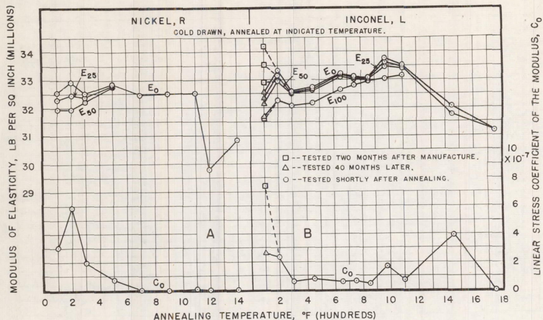
Figure 50.- Variation of tensile modulus of elasticity and of its linear stress coefficient with annealing temperature. A-Gold-drawn nickel rod R. B-Cold-drawn Inconel rod L.
