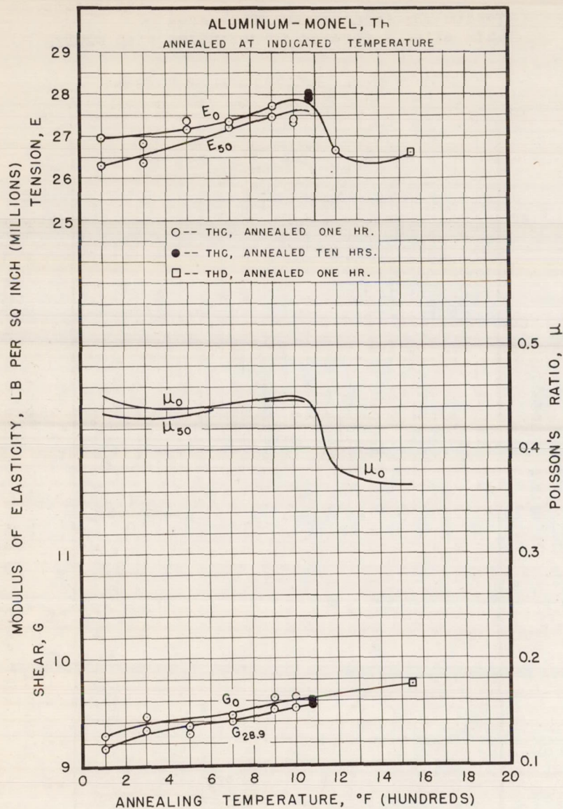
Figure 66.- Variation of Poisson's ratio with annealing temperature for aluminum-monel tubing TH.
