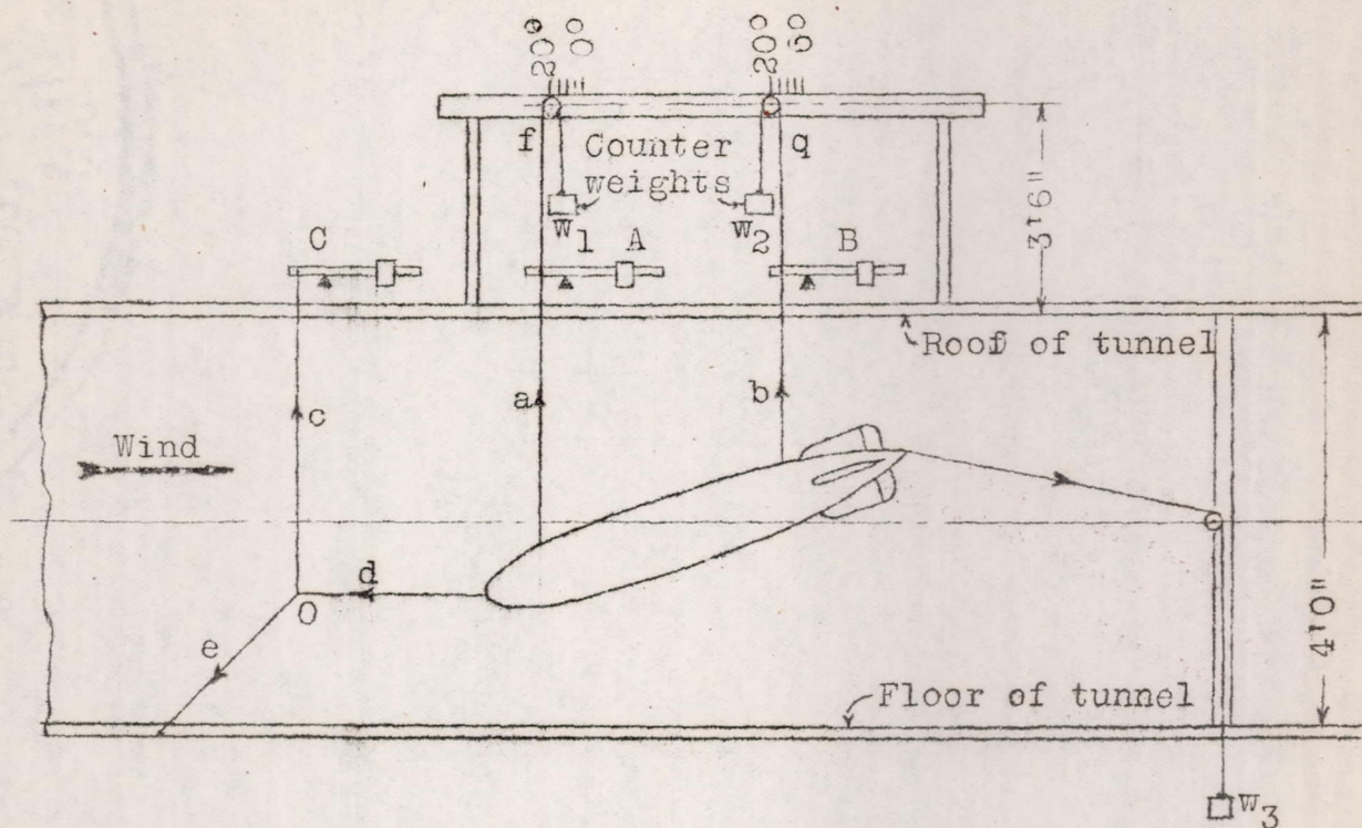
Fig. 4 General arrangement of apparatus
