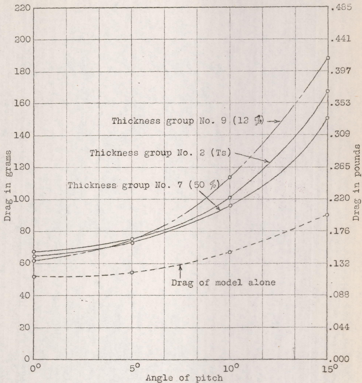
Drag curves for elevator angle 10°
