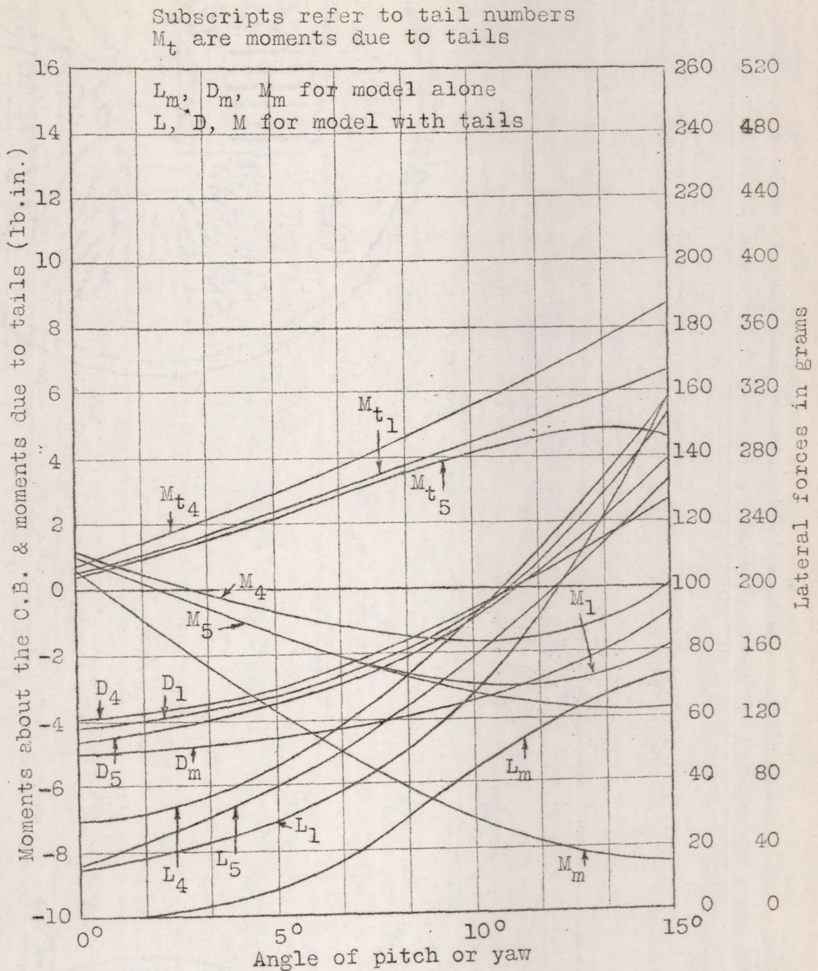
Fig. 17 Performance curves of an L-33 model fitted with aspect ratio tail surfaces. Elevators 10°
