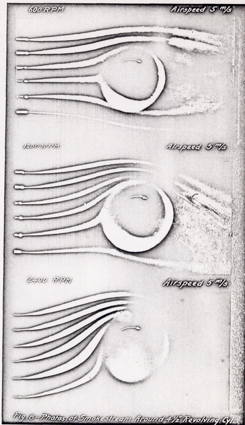
Fig.8 Photographs of smokestream around 4 1/2" revolving cylinder.
