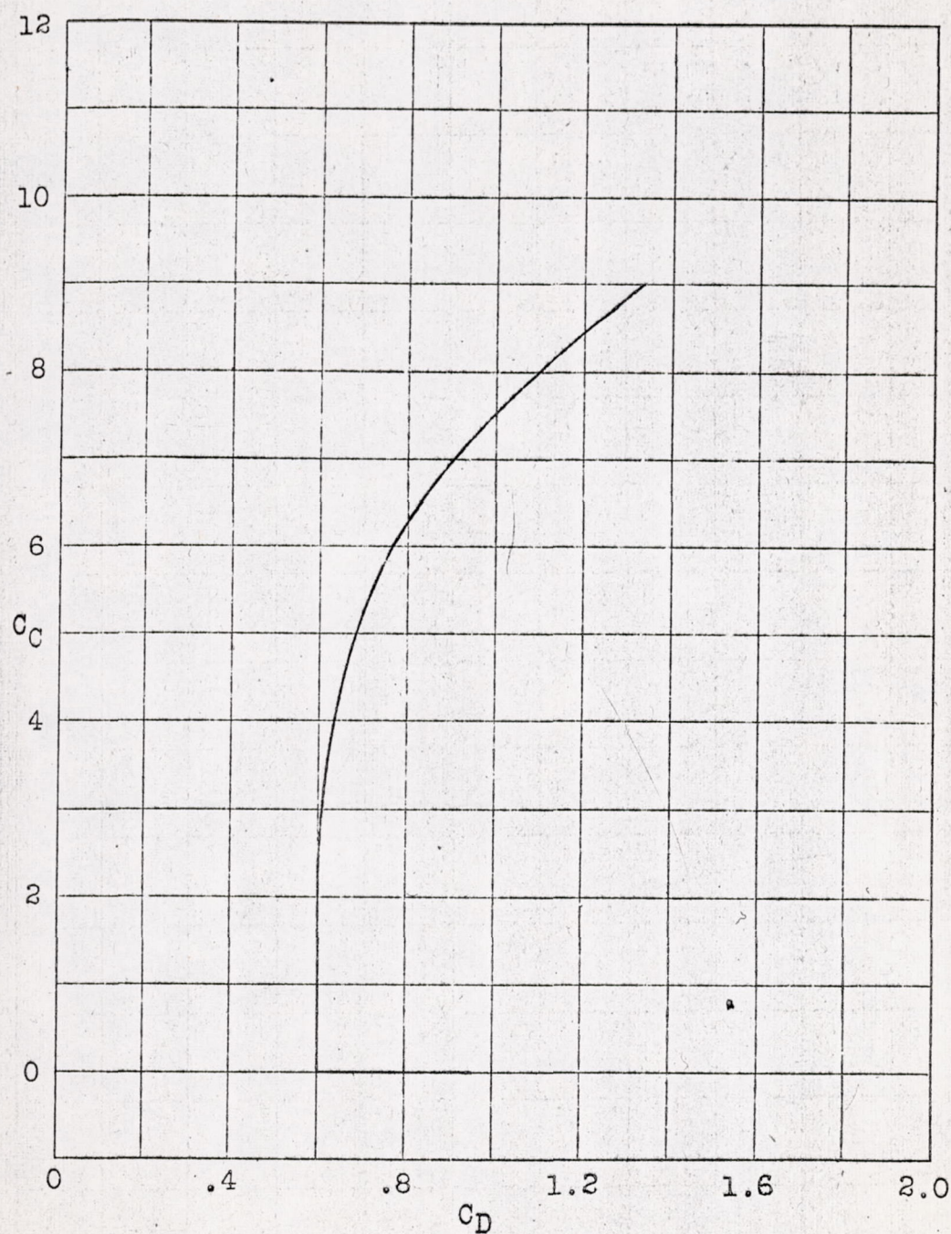
Fig.5 Cross wind & drag coeffs. for rotating circular cylinder.
