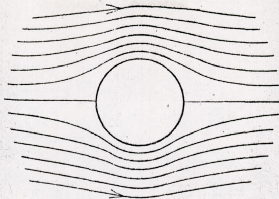
Fig.1 Uniplanar uniform flow around circular cylinder.
