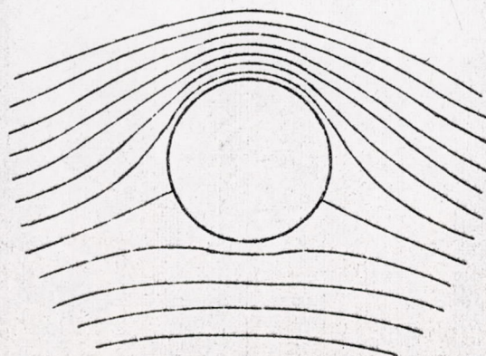
Fig.2 Uniplanar flow around circular cylinder considered as a columnar vortex of strength \Gamma .
