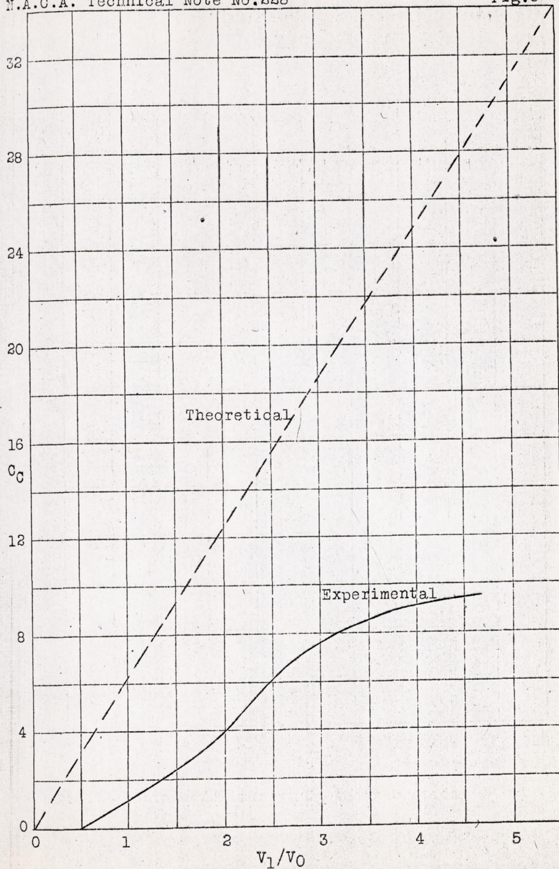
Fig. 6 Cross wind force coeff. vs. V_1/V_0 for rotating cylinder.
