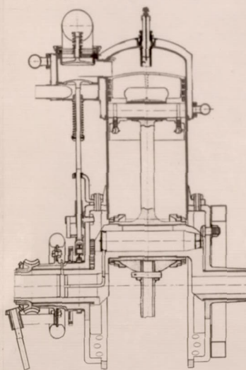
Fig. 25 Manly 5-cylinder, water-cooled engine. 2.35 lb./HP., dry weight. 52.4 HP. at 950 R.P.M.
