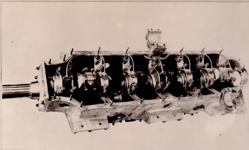
Fig. 20 Wright T-3 crankcase with crankshaft.
