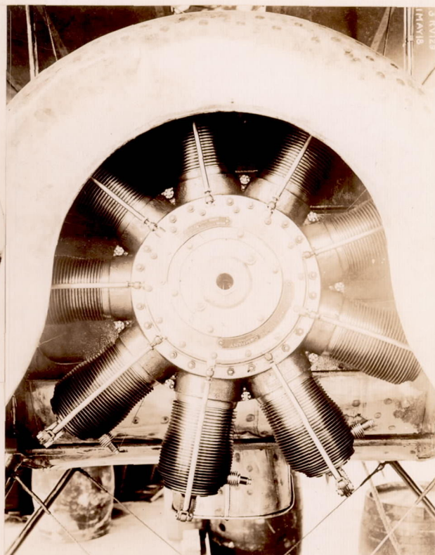
Fig.2 Gnome rotary 9-cylinder air-cooled engine 3-1/2 lb./HP. 90-100 HP. steel cylinder barrel and fins.
