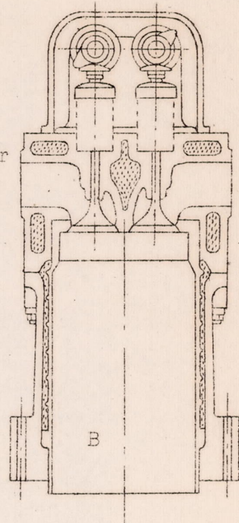
B - Curtiss D-12 cylinder construction - wet cylinder barrel and cast aluminum jacket.
