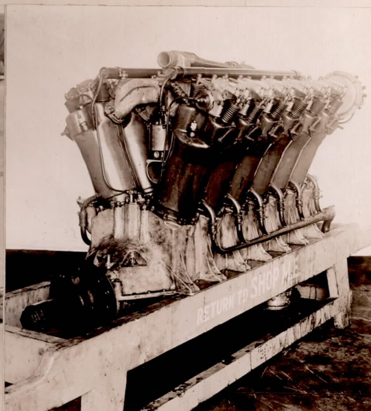
Fig.6 Liberty 12-cylinder 45° vee water-cooled engine 2.2 lb./HP. 400 HP. individual cylinders - wet sleeves.
