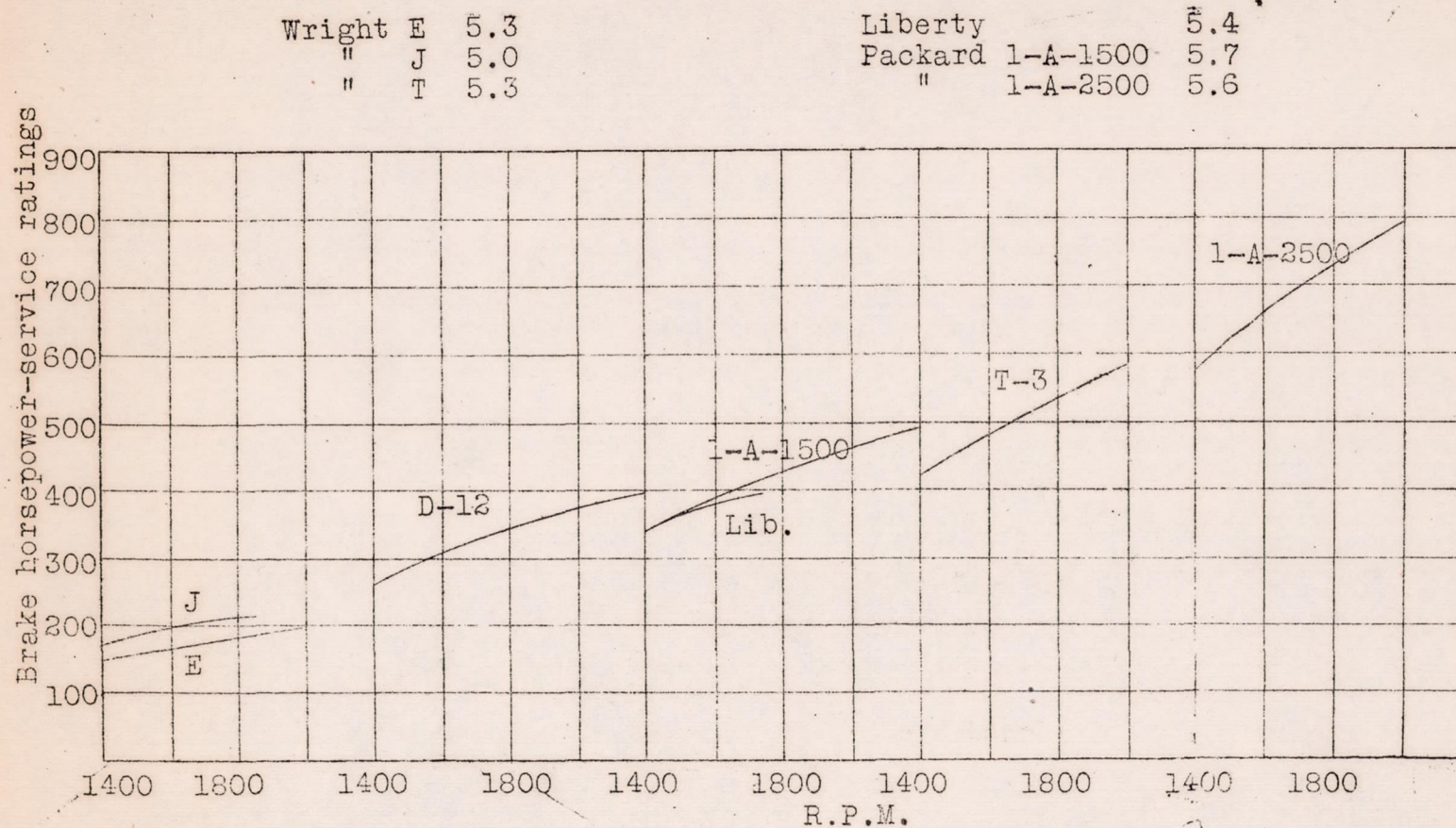
Fig.12. Service ratings of existing aircraft engines (1924).
