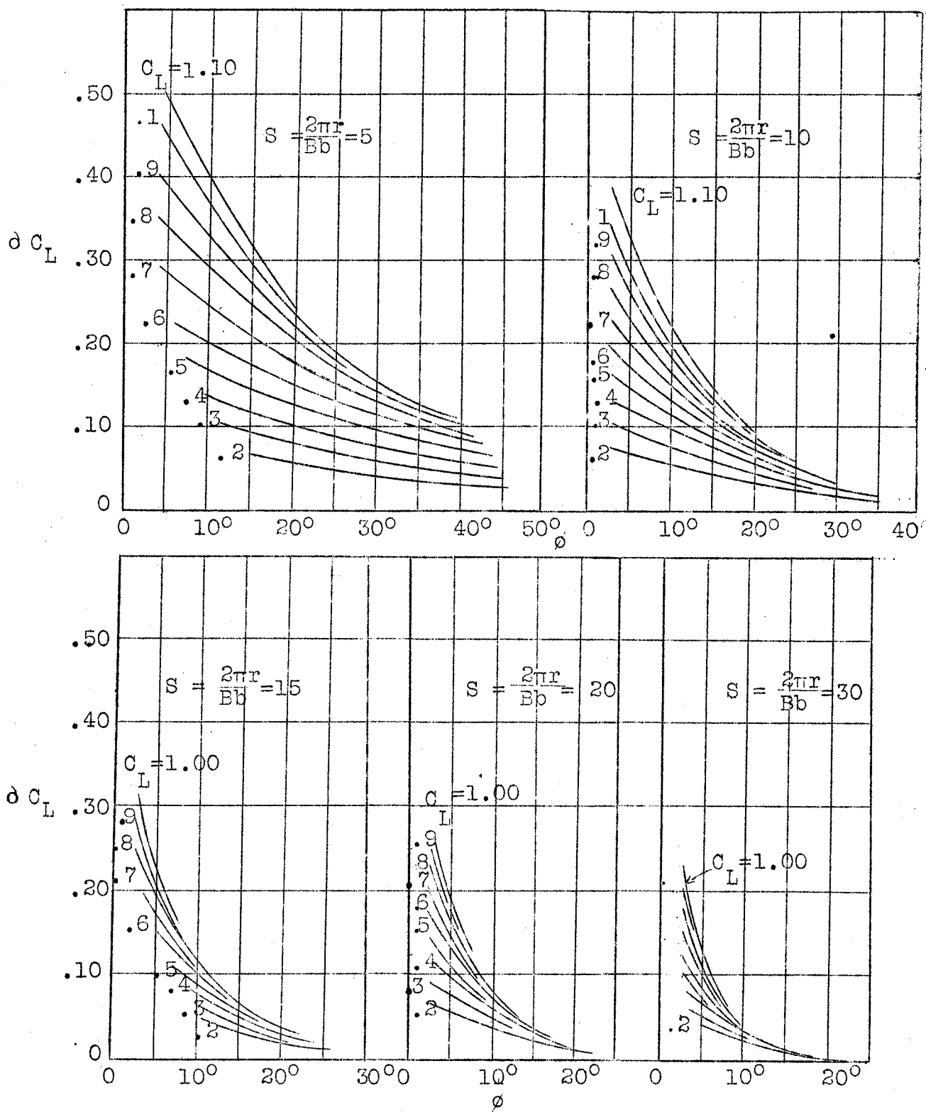
Fig.7 Lift correction, \Delta C_L .
