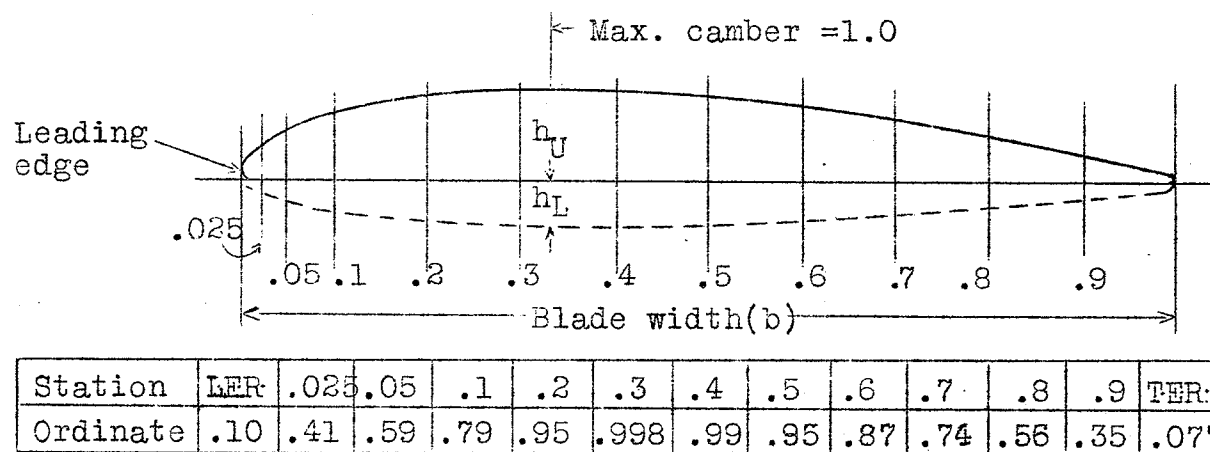
Fig.9 Navy standard blade section.R.A.F.No.6 Modified, flat face.
