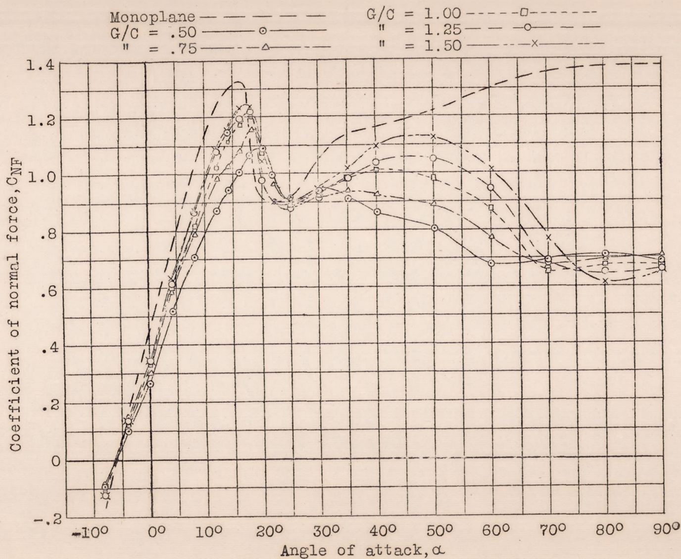
Fig.16 Effect of gap on cellule normal force coefficient.
