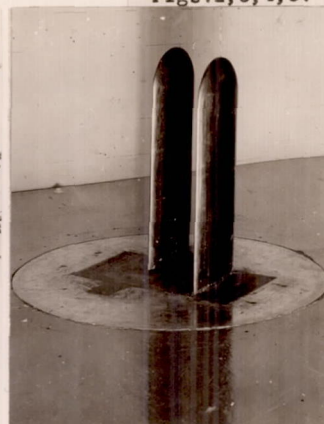
Fig.3 Biplane wings and separation plane in wind tunnel.
