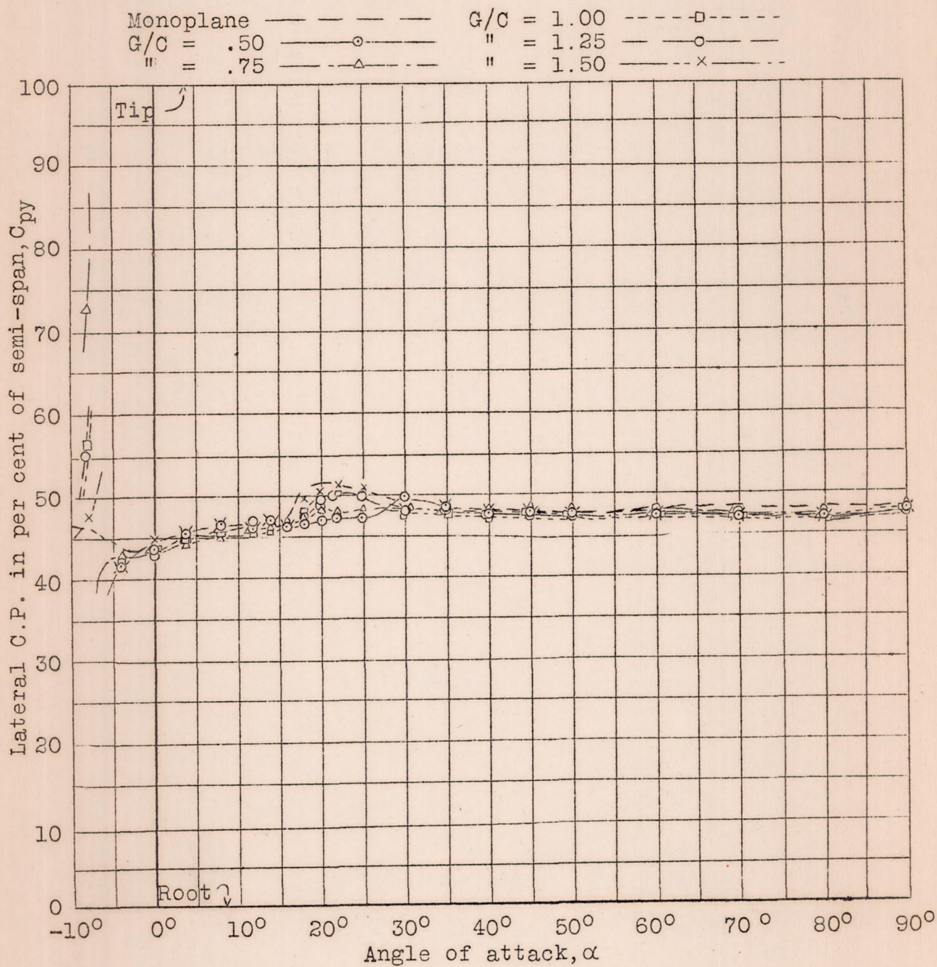
Fig.23 Effect of gap on lower wing lateral center of pressure.
