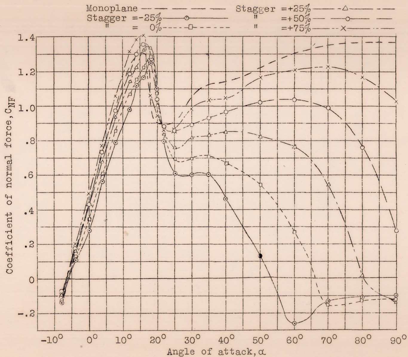
Fig.8 Effect of stagger on upper wing normal force coefficient.
