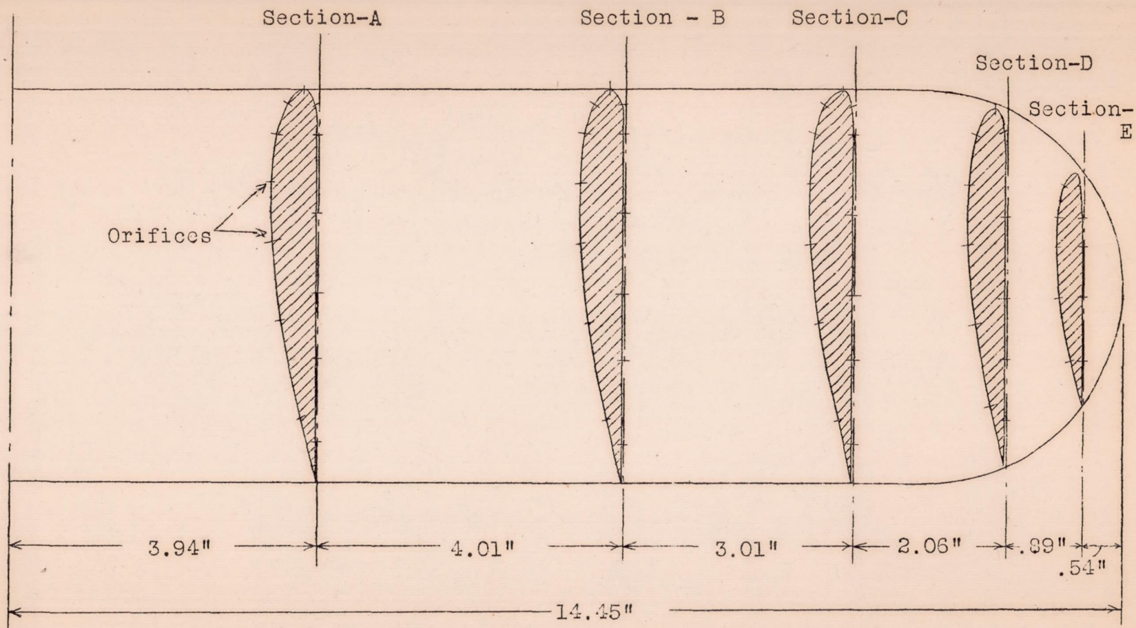
Fig.2 Wing showing orifice locations.
