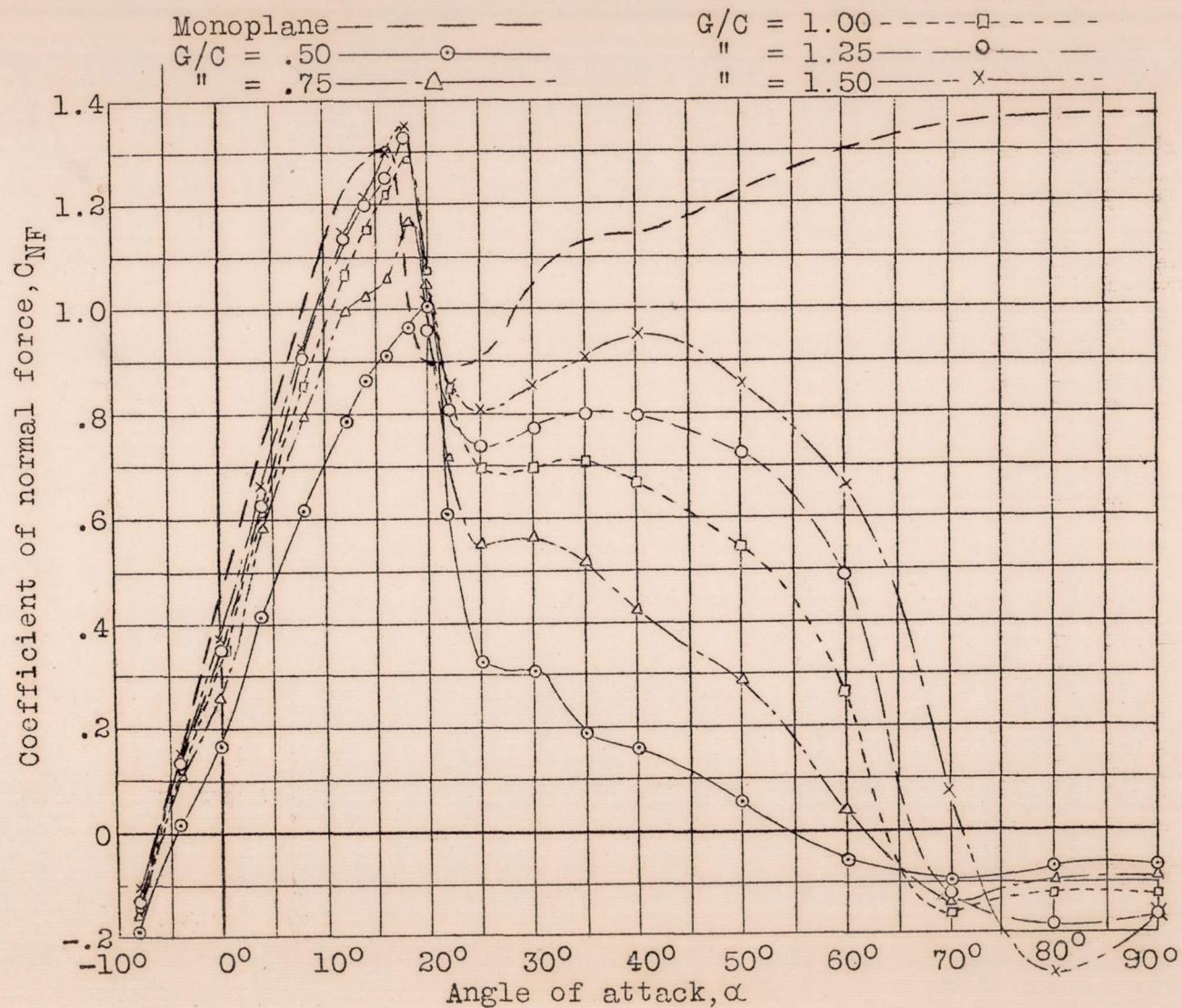
Fig 17 Effect of gap on upper wing normal force coefficient.
