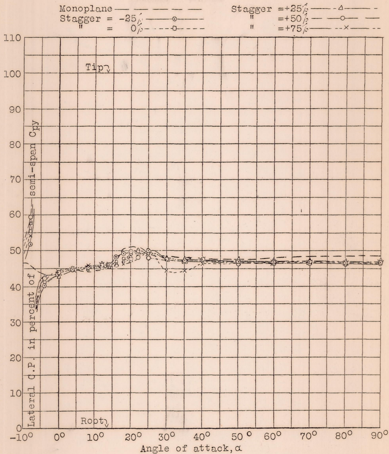
Fig.14 Effect of stagger on lower wing lateral center of pressure.
