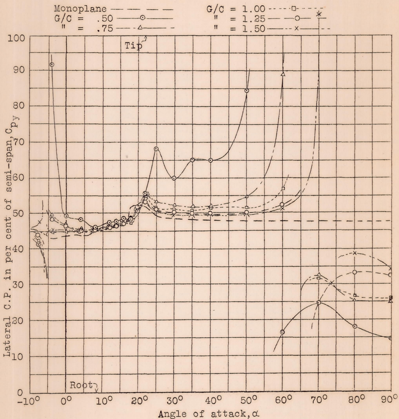
Fig.22 Effect of gap on upper wing lateral center of pressure.
