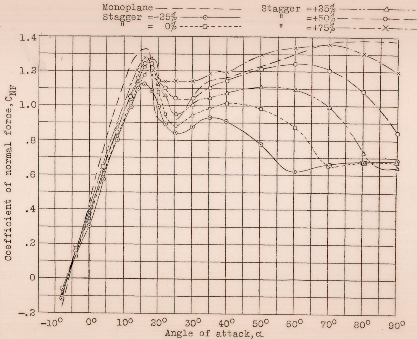
Fig.7 Effect of stagger on cellule normal force coefficient.
