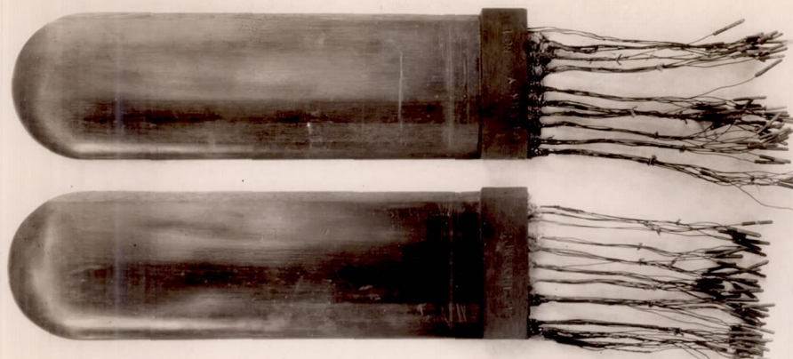
Fig.1 Half-span pressure distribution wing models.
