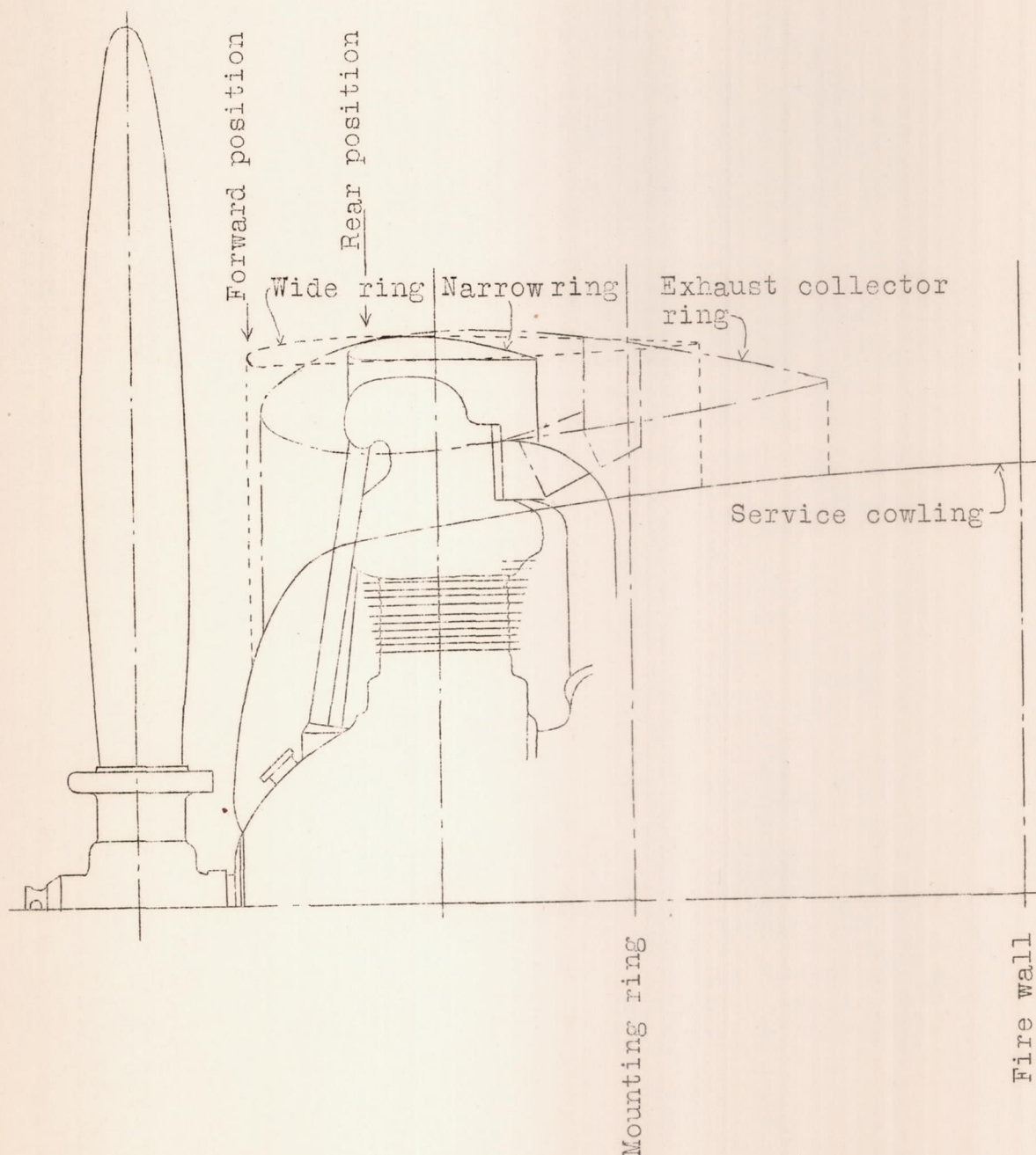
Fig.3 Scale drawing showing cowling sections and location of cowling with respect to center line of cylinders.
