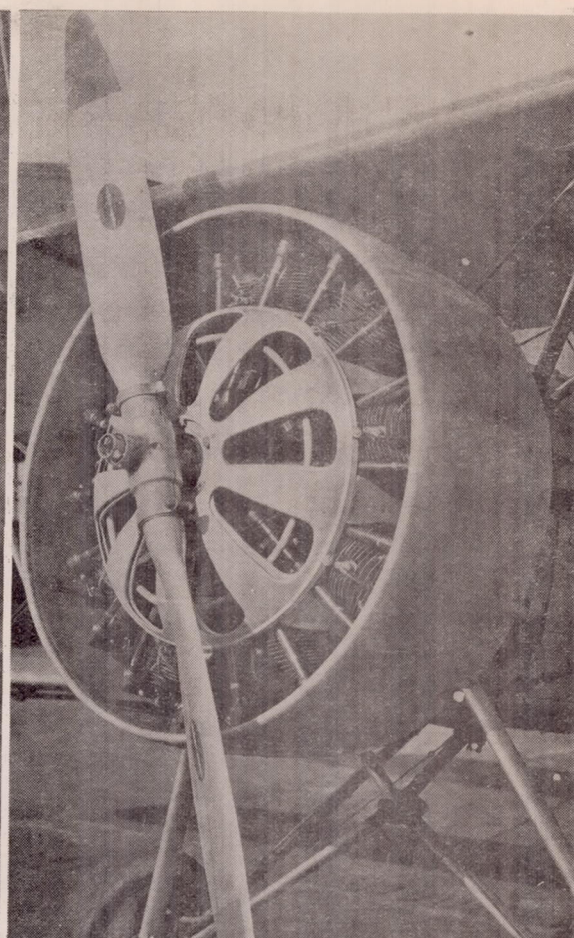
Fig. 5 Three-quarter front view of wide ring cowl- ing as used on XF7C-1 airplane over service type cowlings.
