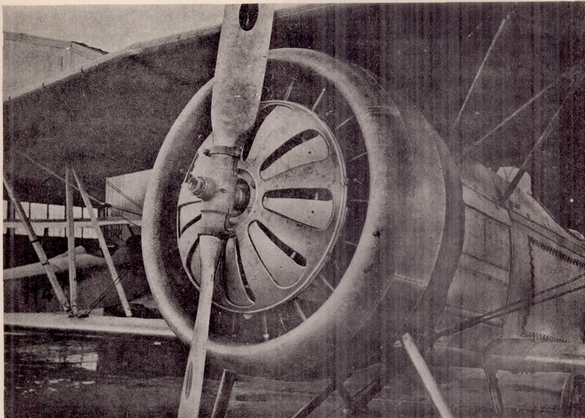
Fig. 11 Three-quarter front view of exhaust collector ring cowl as used on XF7C-1 airplane over service type cowl.
