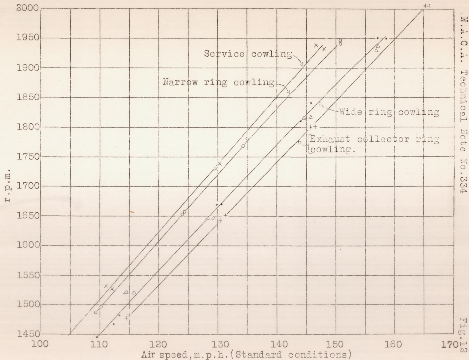
Fig.12 Relation of airspeed to engine speed with service type cowling and with each of three ring cowlings as used over service type cowling in tests on XF7C-1 airplane.
