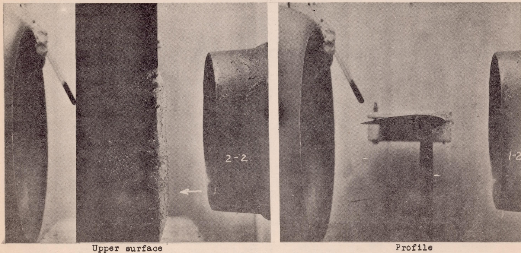
Test on heavy oil coating. Heavy spray. Temperature -1^{\circ}\text{C} . Air speed 70 m.p.h.
