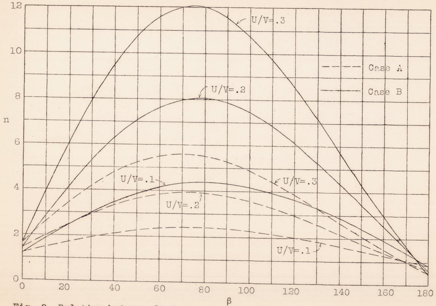
Fig. 2 Relation between load factor and angle \beta
