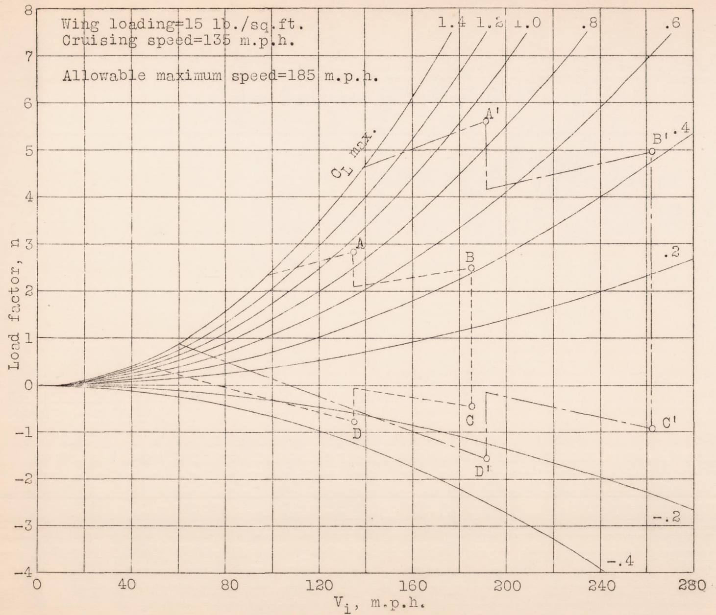
Fig. 6 Load factor chart for a transport airplane.
