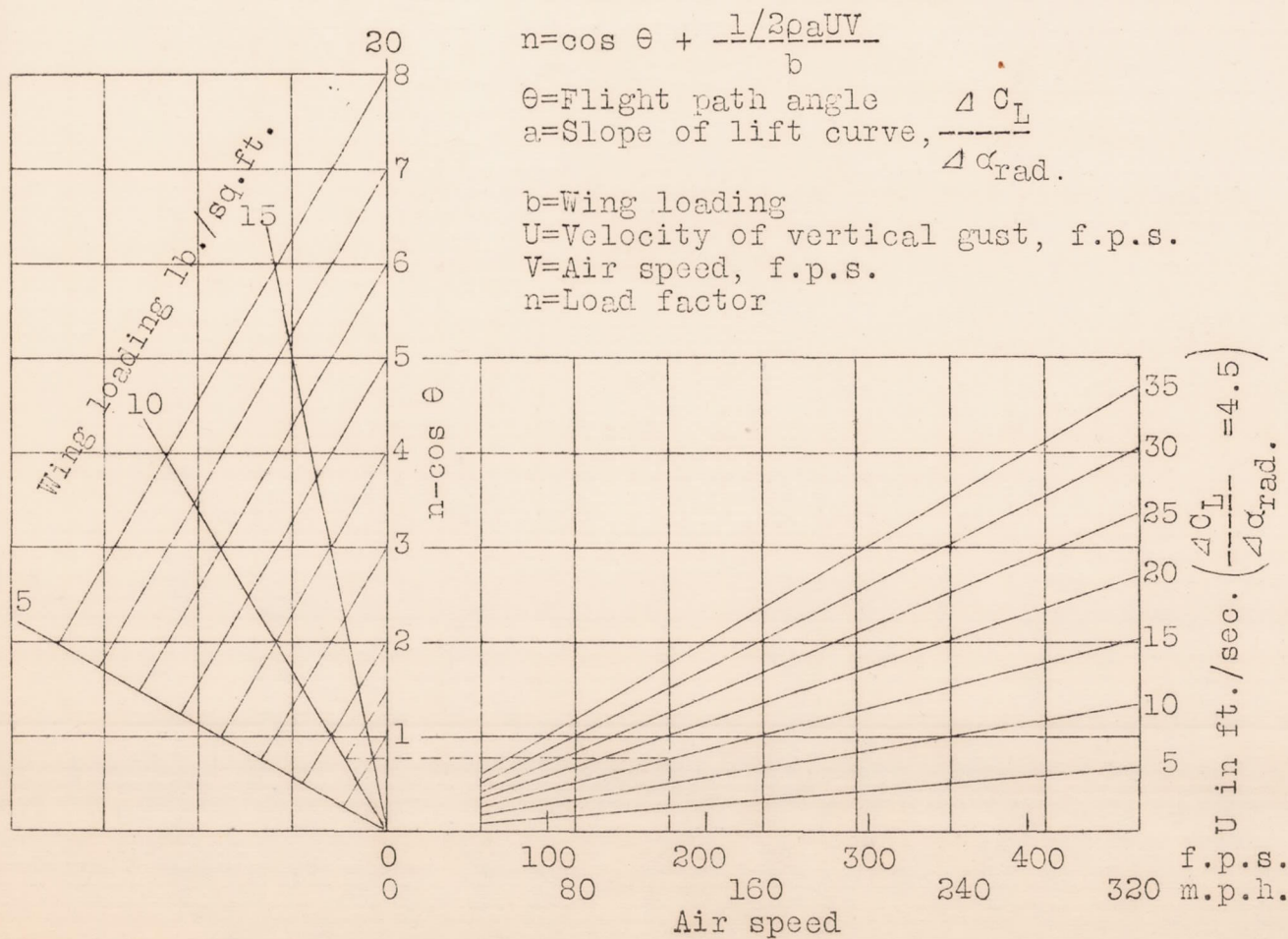
Fig. 5 Applied load factors in bumpy air. Monoplane
