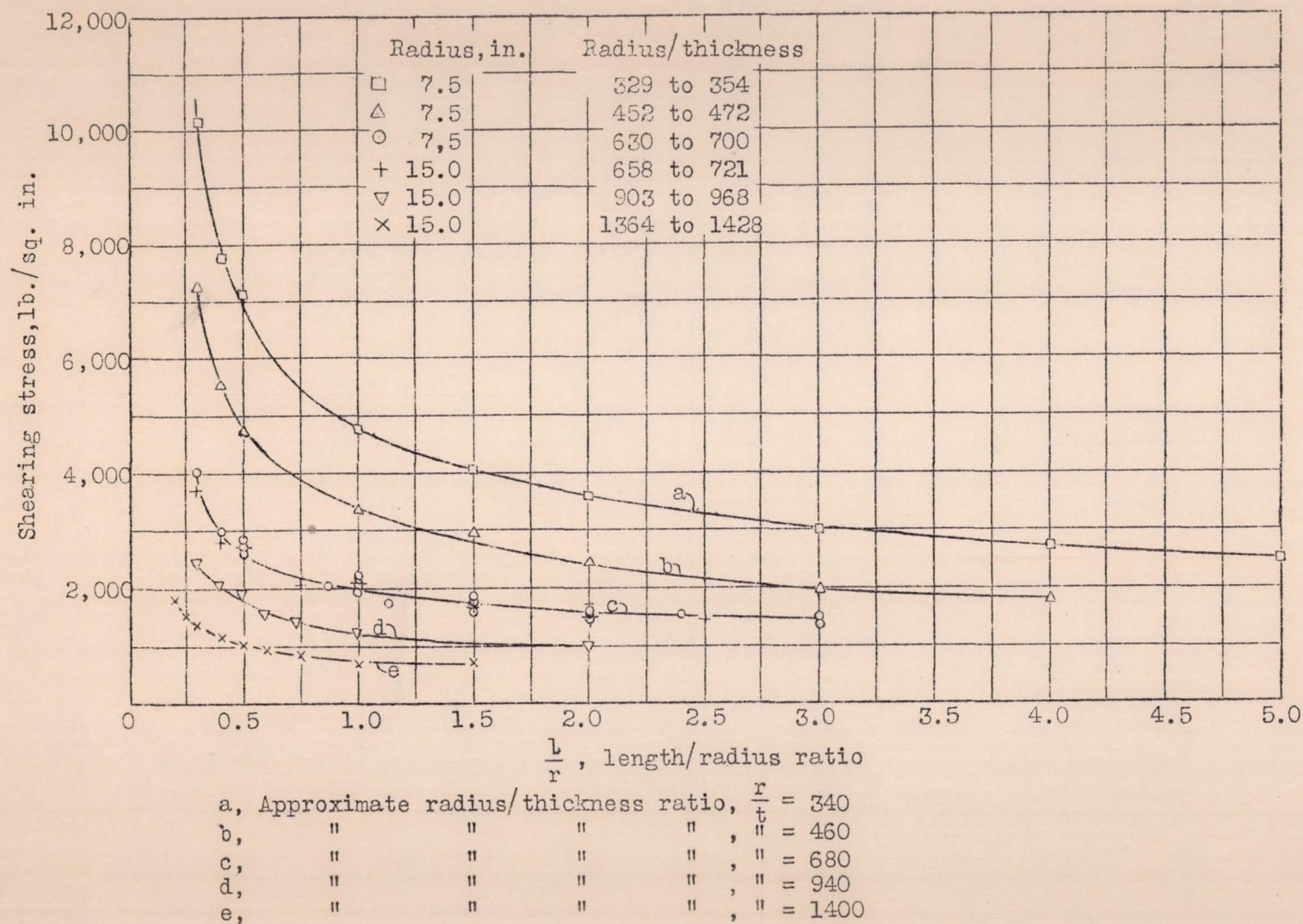
Fig.9 Shearing stress at failure.
