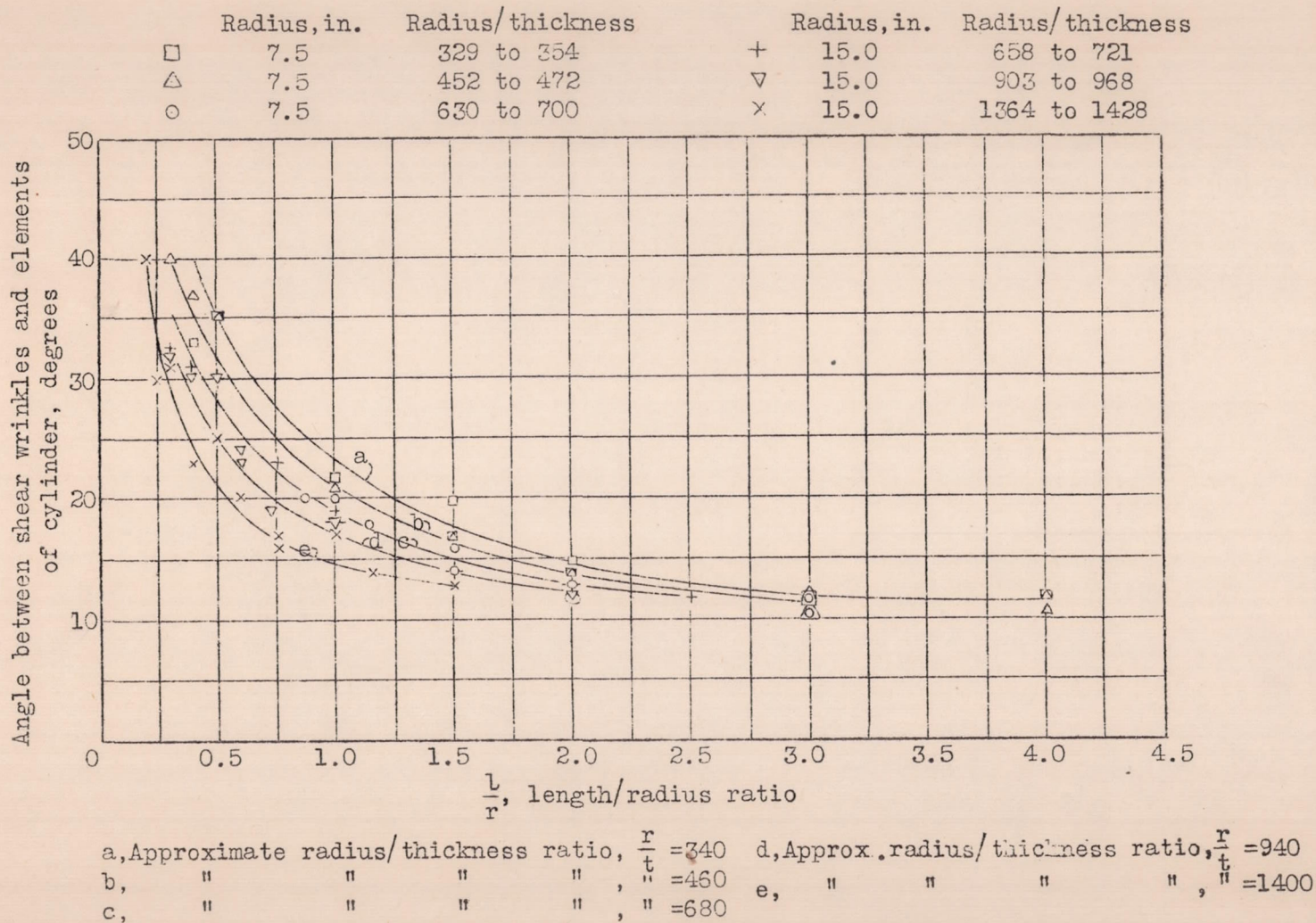
Fig. 8 Angle between shear wrinkles and elements of cylinder.
