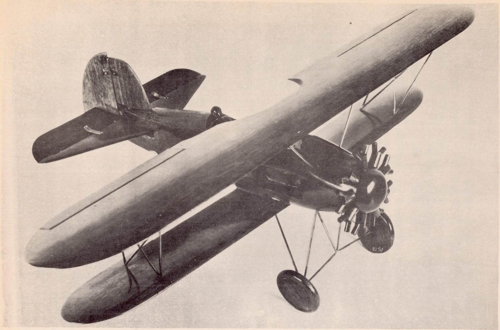
Figure 1.- The 1/12-scale model of the F4B-2 airplane with F4B-4 fin and F4B-3 rudder.
