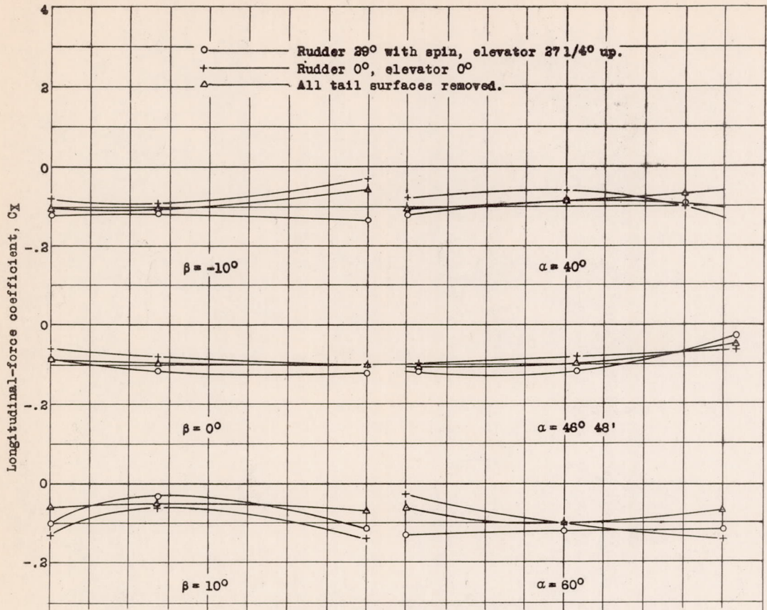
Figure 4.- Variation of C_x with \alpha and \beta . F4B-2 tail surfaces.
