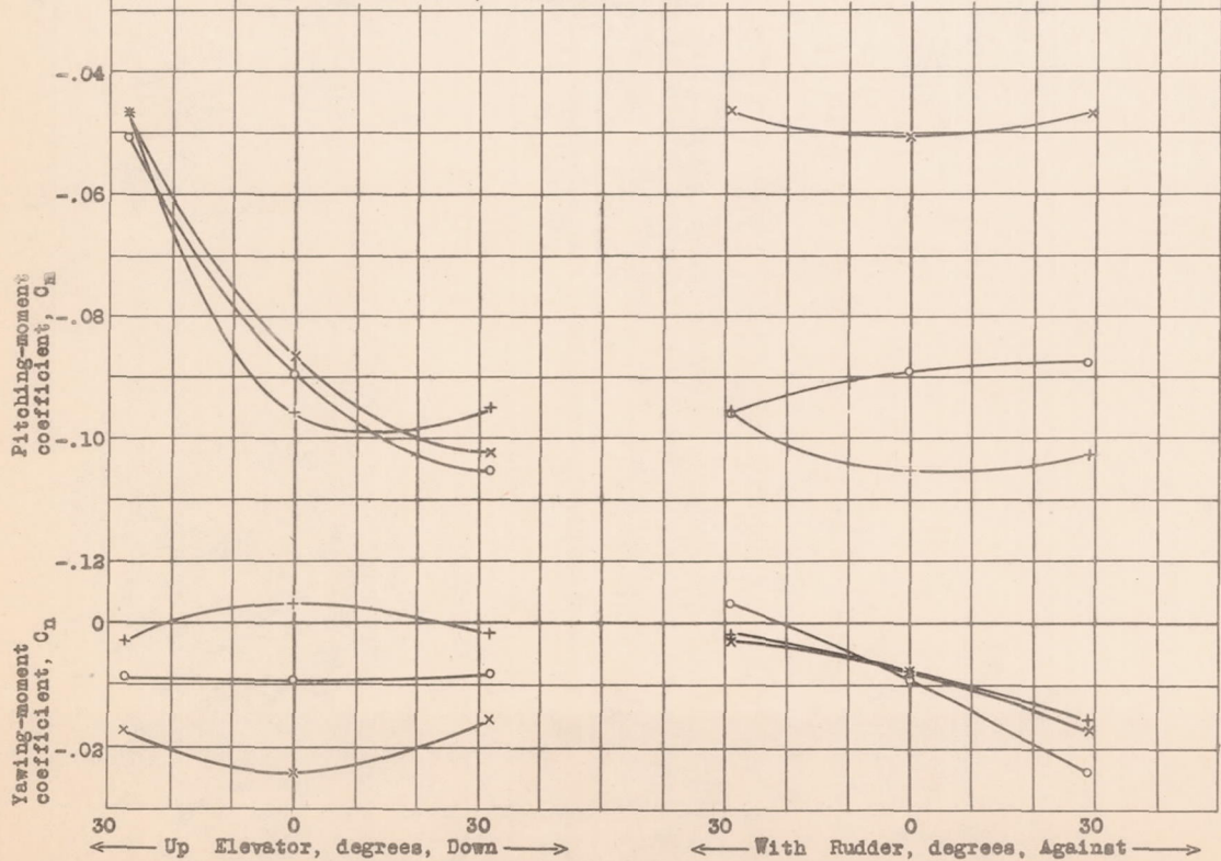
Figure 11.- Variation of C_M and C_N with rudder and elevator movement. F4B-4 fin and F4B-3 rudder with F4B-2 stabilizer, \alpha = 46^\circ 48' and \beta = 0^\circ 42' .
