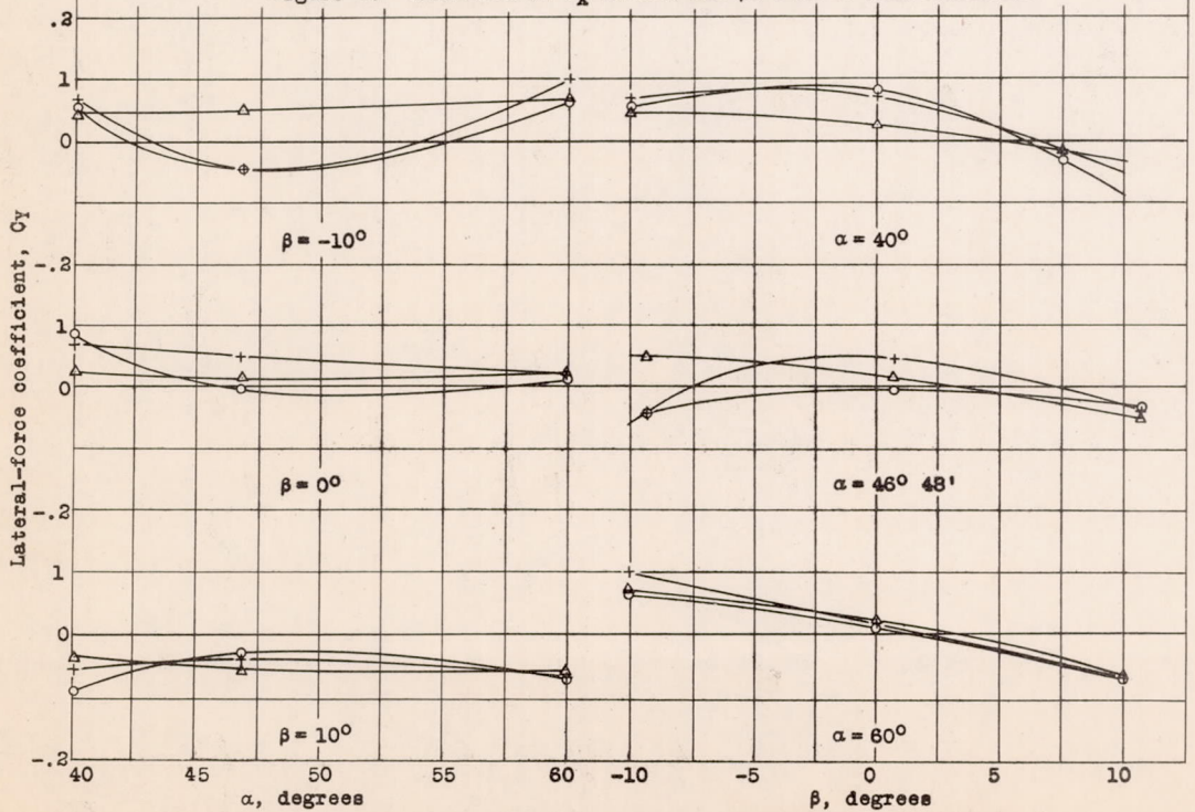
Figure 5.- Variation of C_y with \alpha and \beta . F4B-2 tail surfaces.
