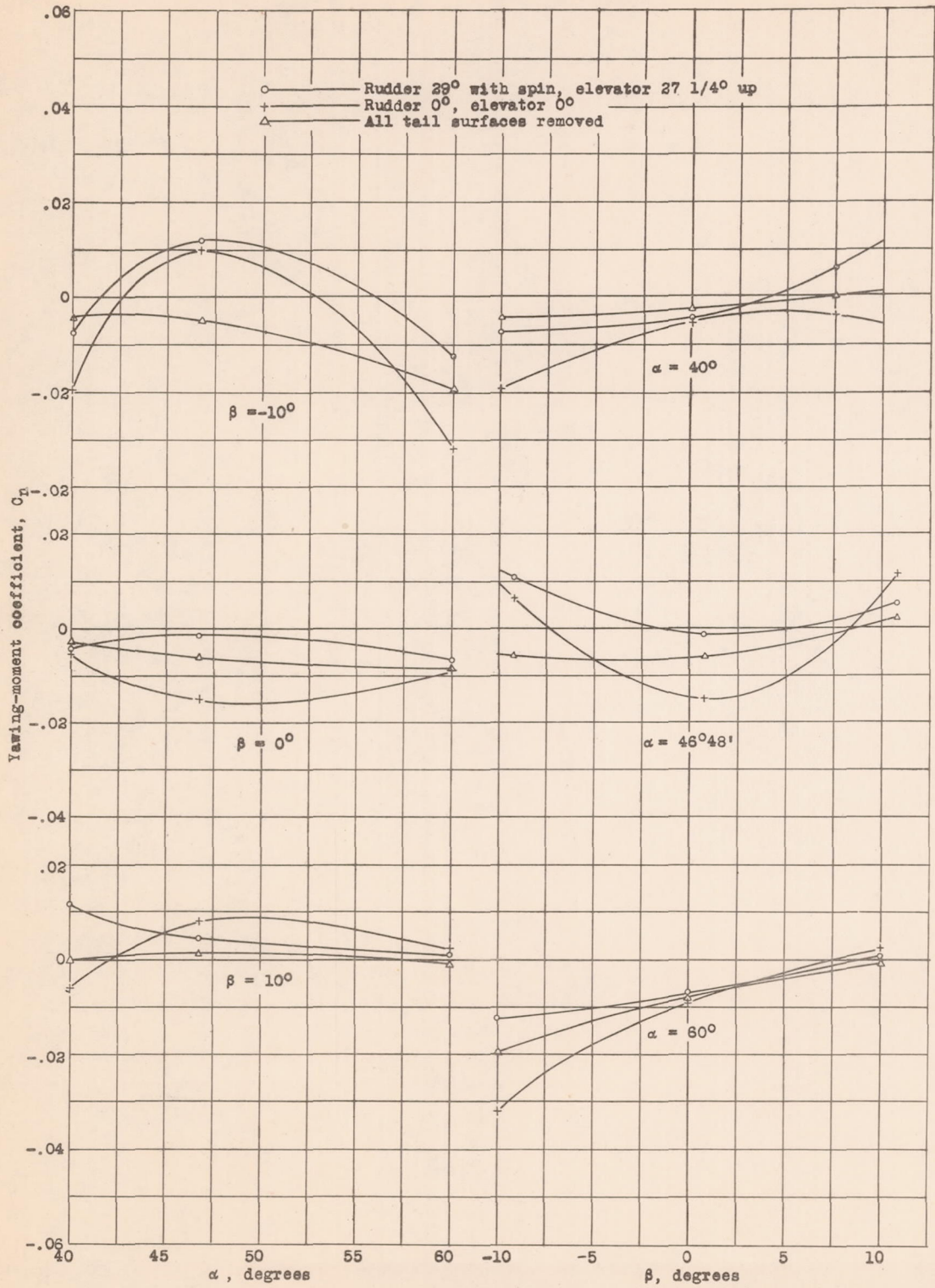
Figure 9.-Variation of C_n with \alpha and \beta . F4B-2 tail surfaces.
