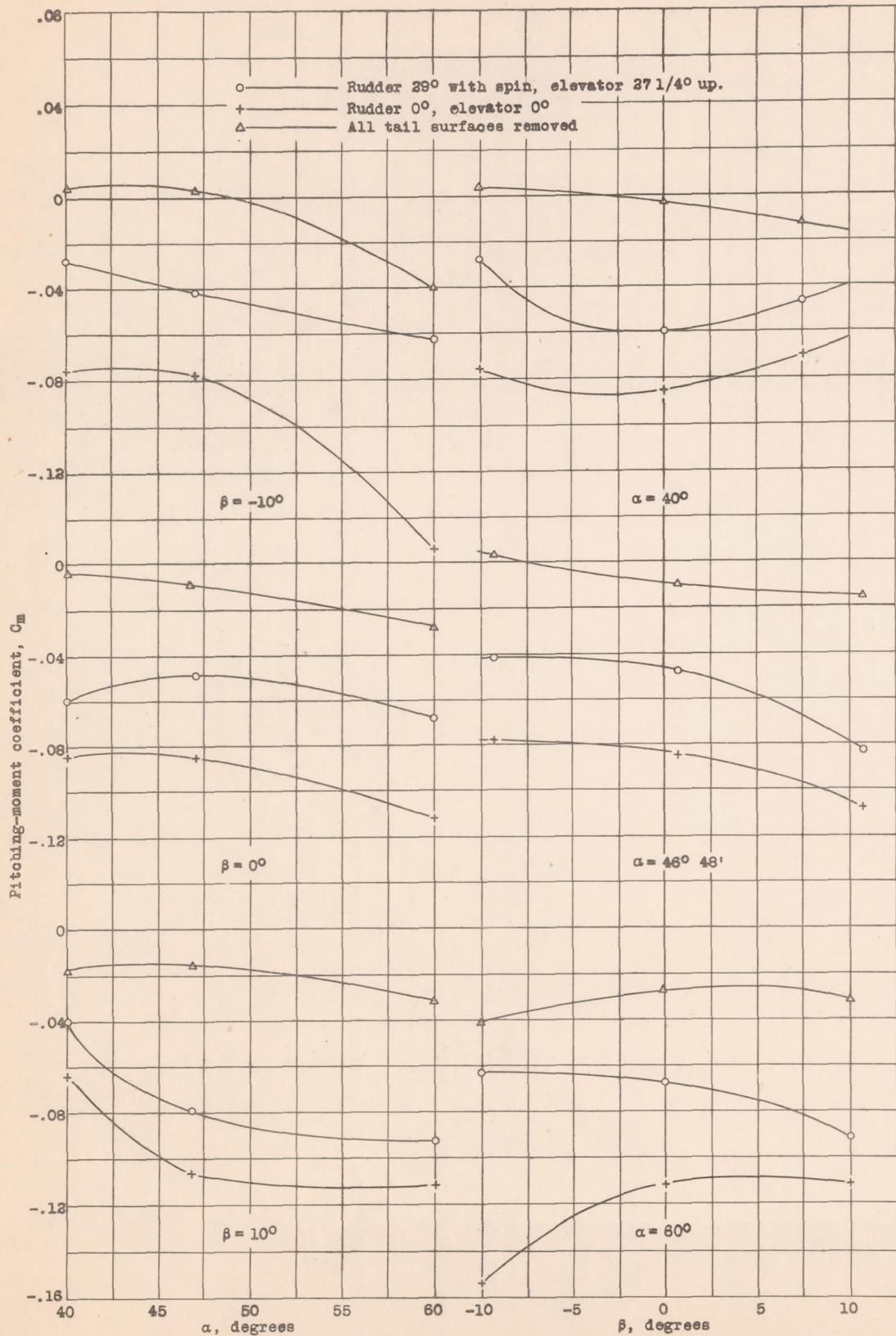
Figure 8.- Variation of C_m with \alpha and \beta . F4B-2 tail surfaces.
