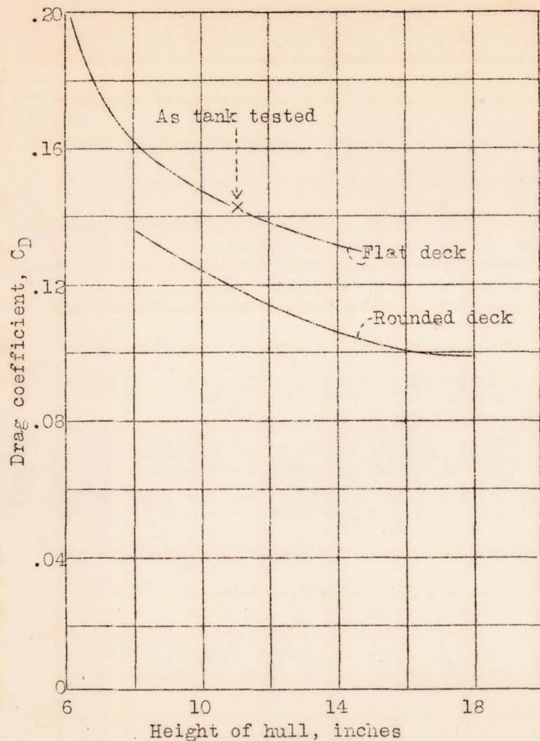
Figure 15.-Variation of drag coefficient with height for hull model 35; pitch angle -2\frac{1}{2}^\circ .
