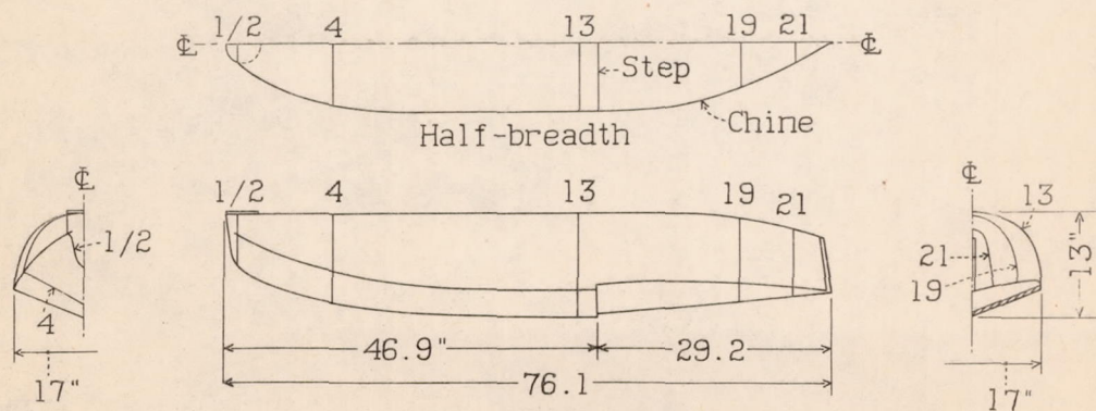
Figure 12.- Lines of N.A.C.A. Model 44.
