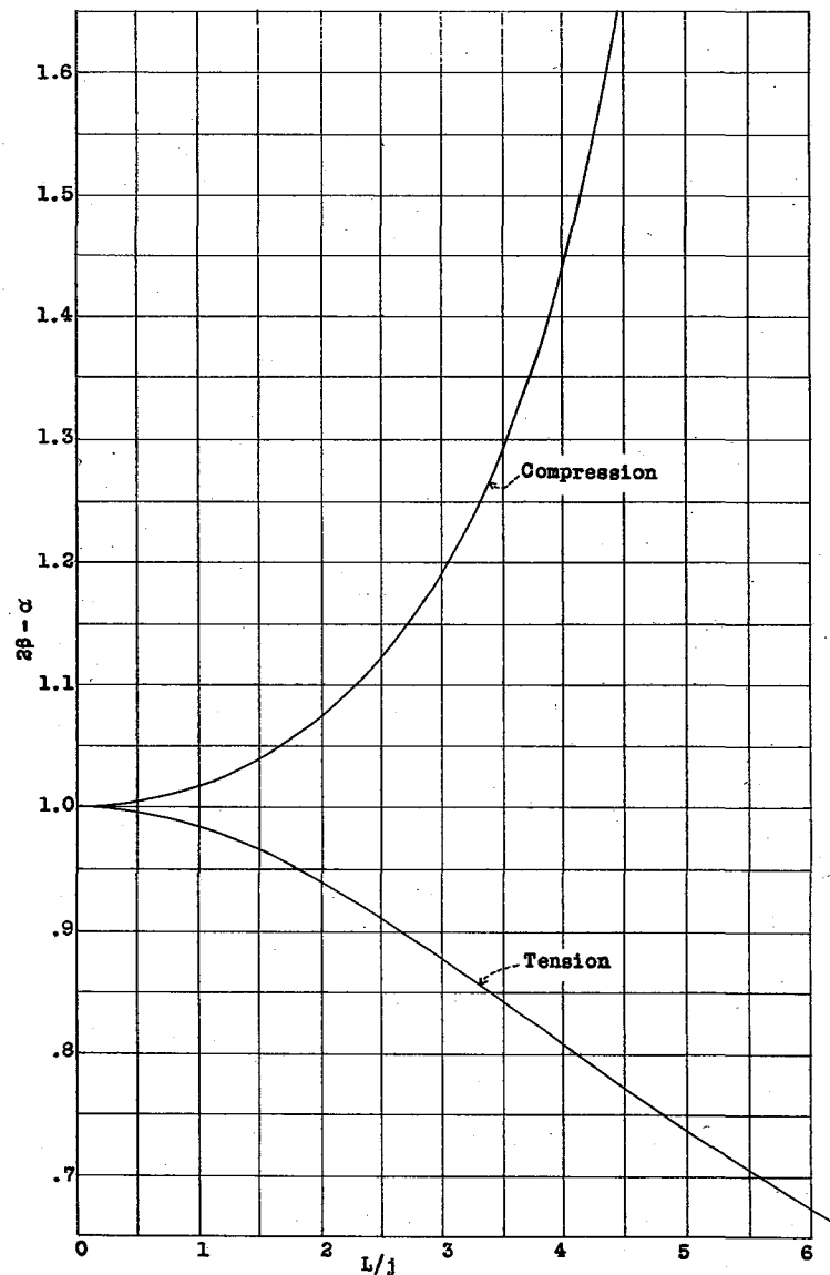
Graph XI.- Column distribution factor. 2\beta - \alpha .
