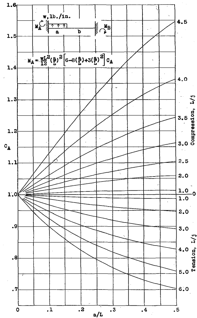
Graph IX.- Fixed-end moment coefficient for M_A . Uniform load of part of the span.
