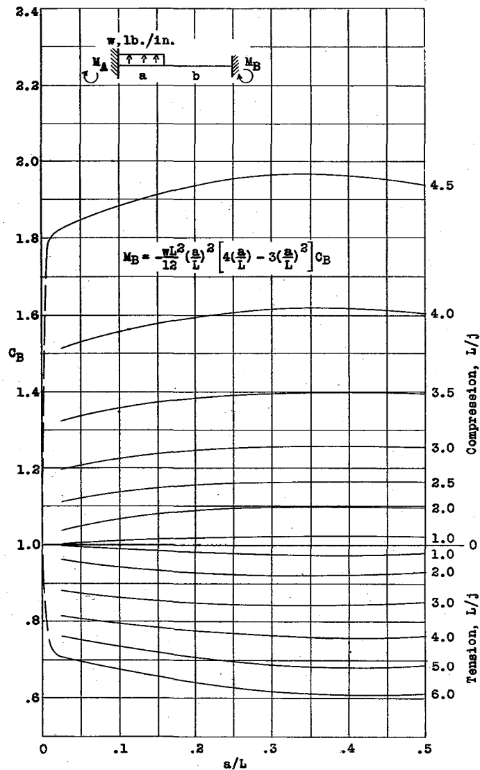
Graph X.- Fixed-end moment coefficient for M_B . Uniform load over part of the span.
