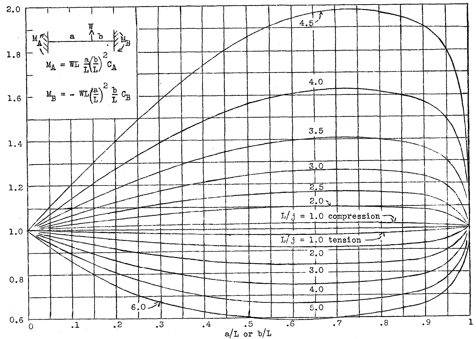
Graph VII. Fixed-end moment coefficient. Concentrated load
