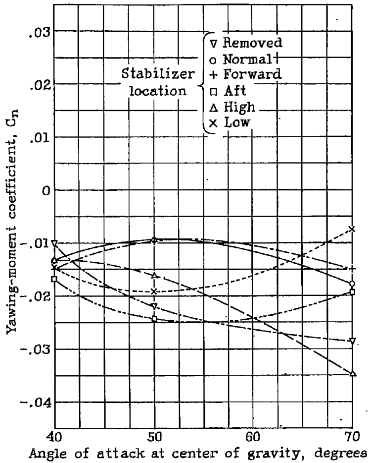
Figure 5.- Yawing-moment coefficients due to fin and rudder. Sideslip at c.g. -10^\circ (outward). C_n (controls 35^\circ with the spin), -C_n (tail surfaces removed).
