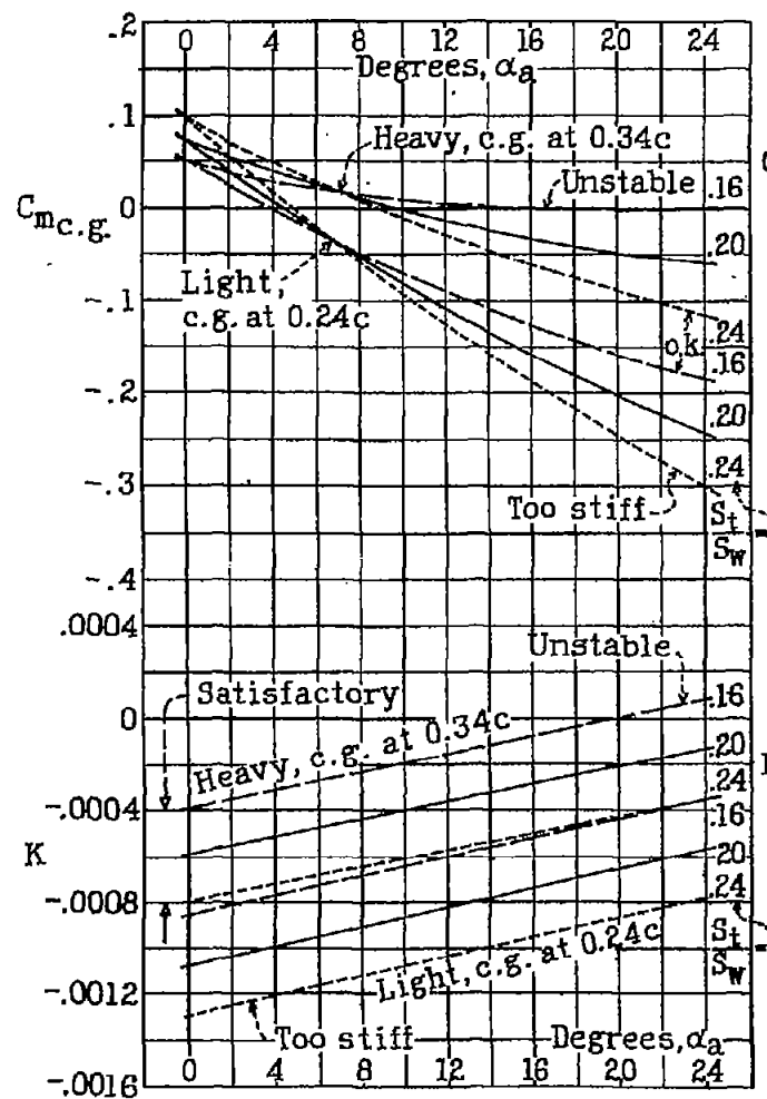
Figure 8.- The effect of horizontal position of the center of gravity on the stability coefficient. Light and heavy low-wing commercial airplanes.
