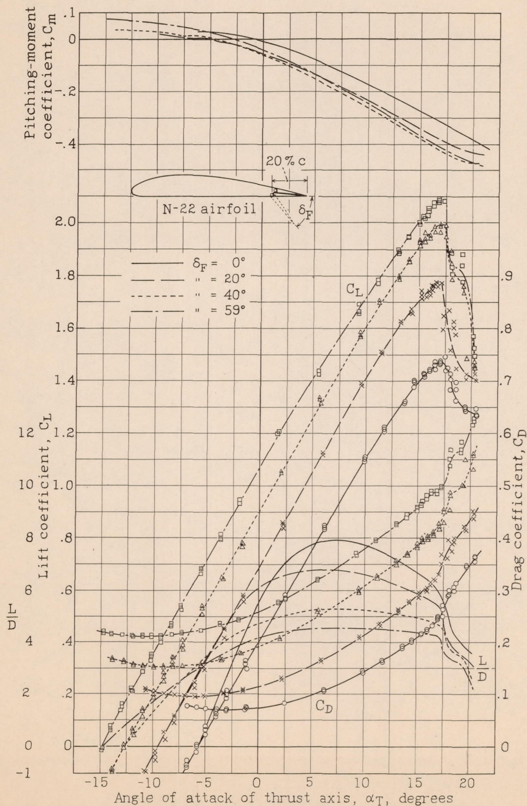
Figure 5-Lift, drag, and pitching-moment curves for the Fairchild F-22 airplane with split trailing-edge wing flaps. Horizontal tail surfaces set 0^\circ to the thrust axis. Corrected for wind-tunnel effects.
