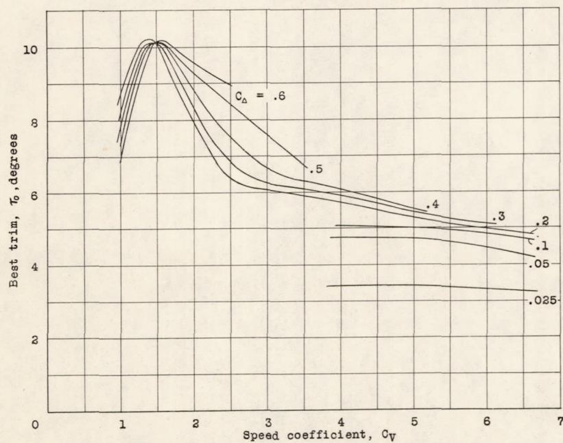
Figure 12.-Variation of best trim, \gamma_0 , with speed coefficient, C_V
