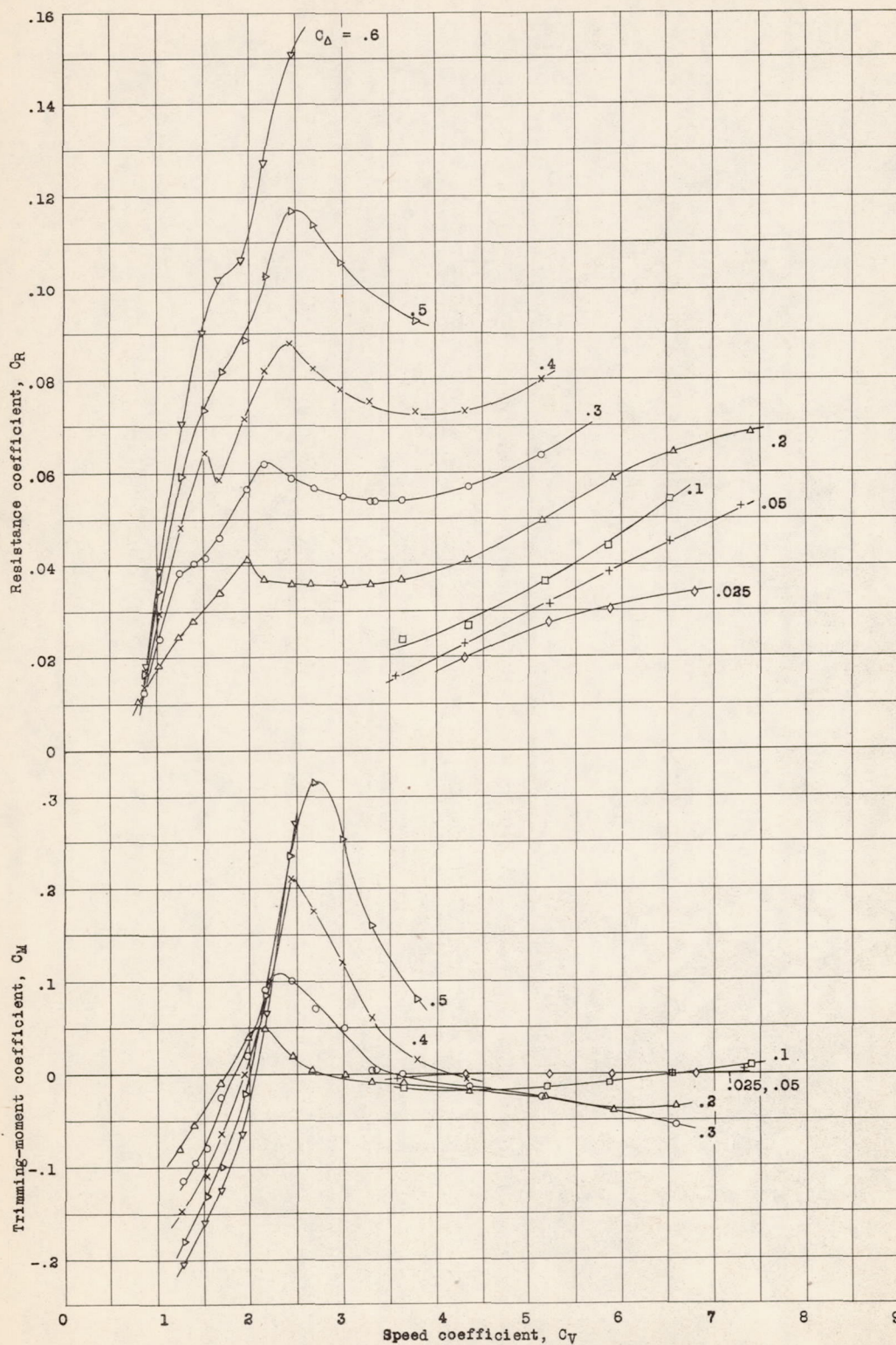
Figure 6.-Resistance coefficient and trimming-moment coefficient. \tau = 7^\circ
