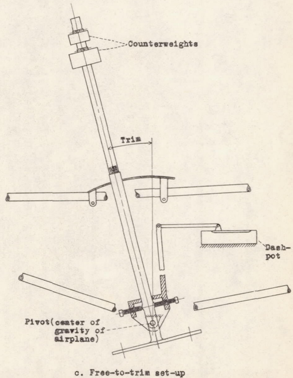
Figure 2.—Diagrams of set-ups for free-to-trim and fixed-trim tests.
