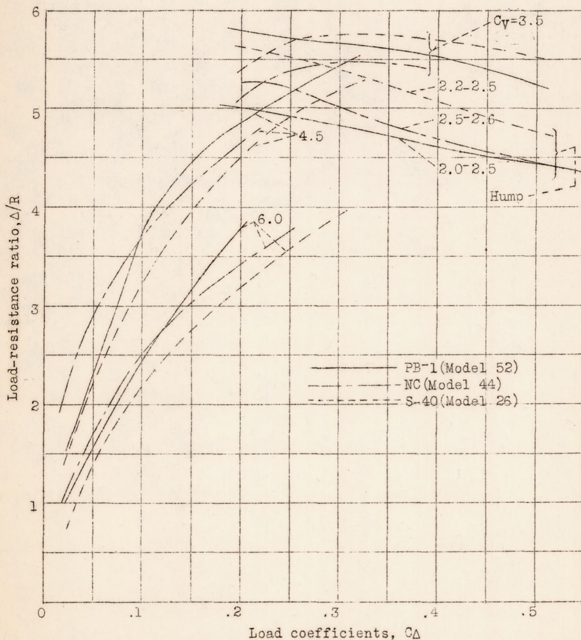
Figure 19.- Comparison of load-resistance ratios of PB-1, NC, and S-40 flying-boat hulls.
