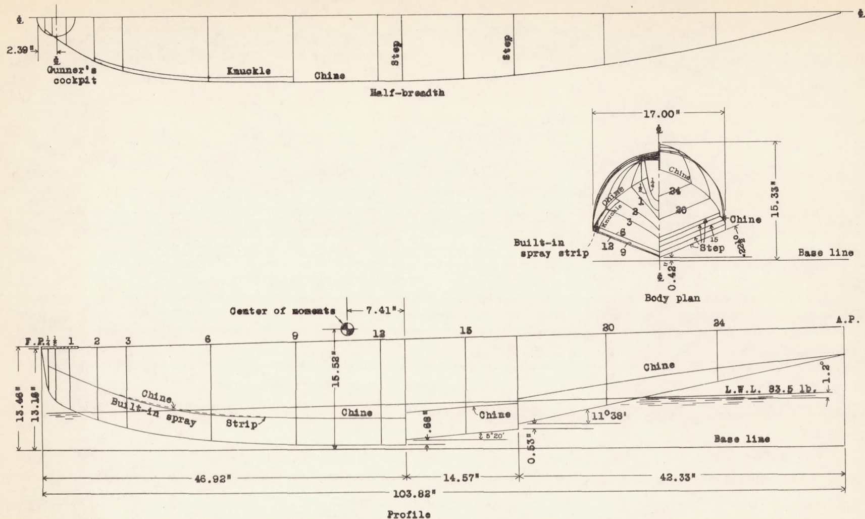
Figure 1.—Lines of N.A.C.A. model 53 (Boeing PB-1).
