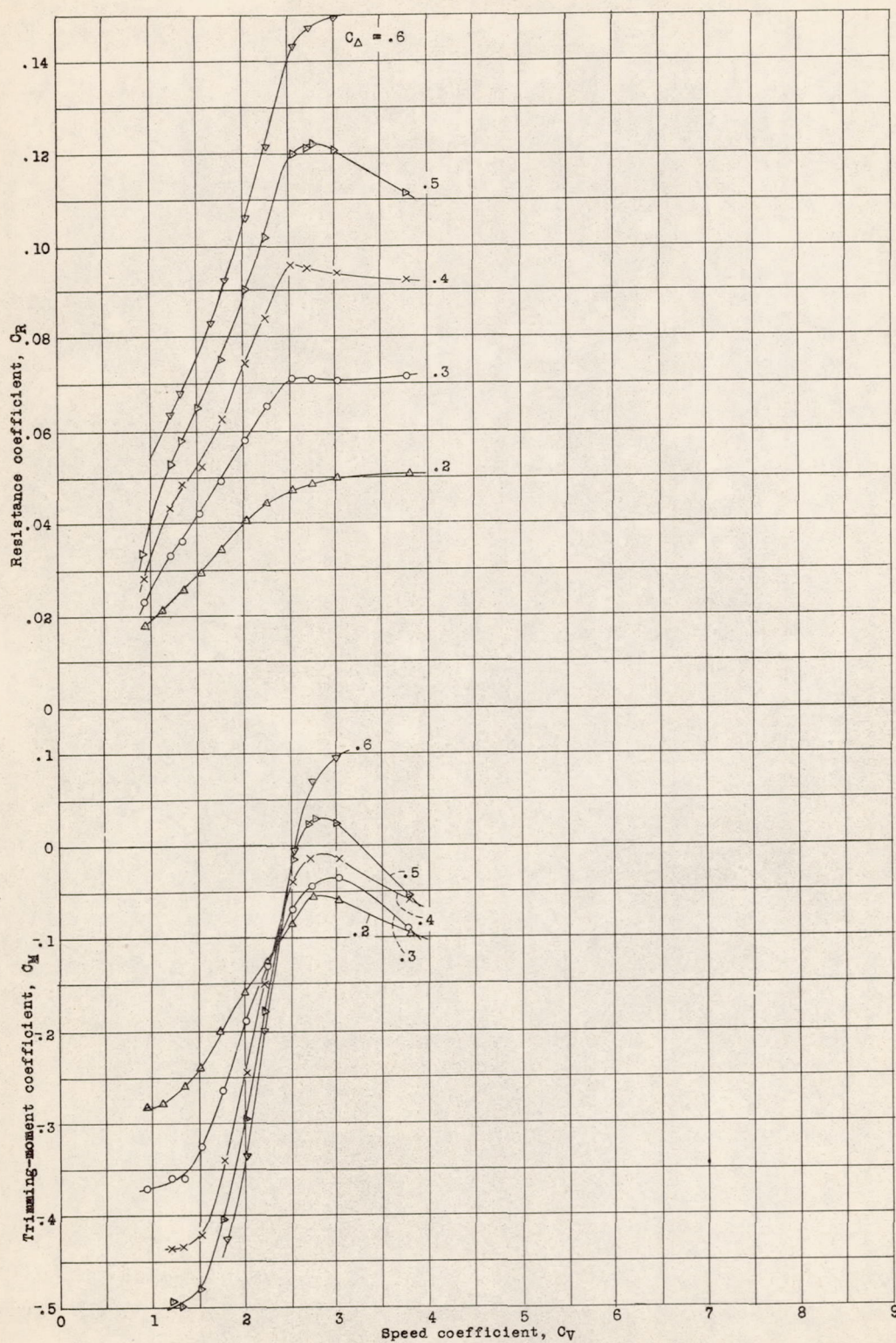
Figure 8.- Resistance coefficient and trimming-moment coefficient, \tau = 11^\circ
