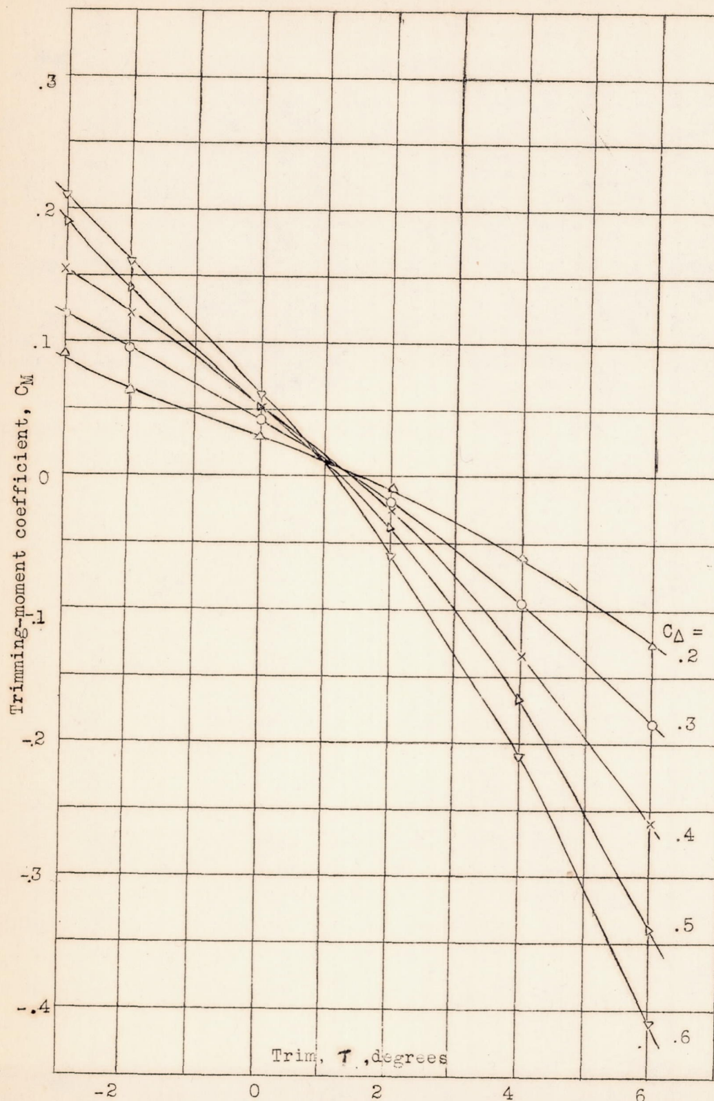
Figure 15. Trimming-moment coefficients at rest.
