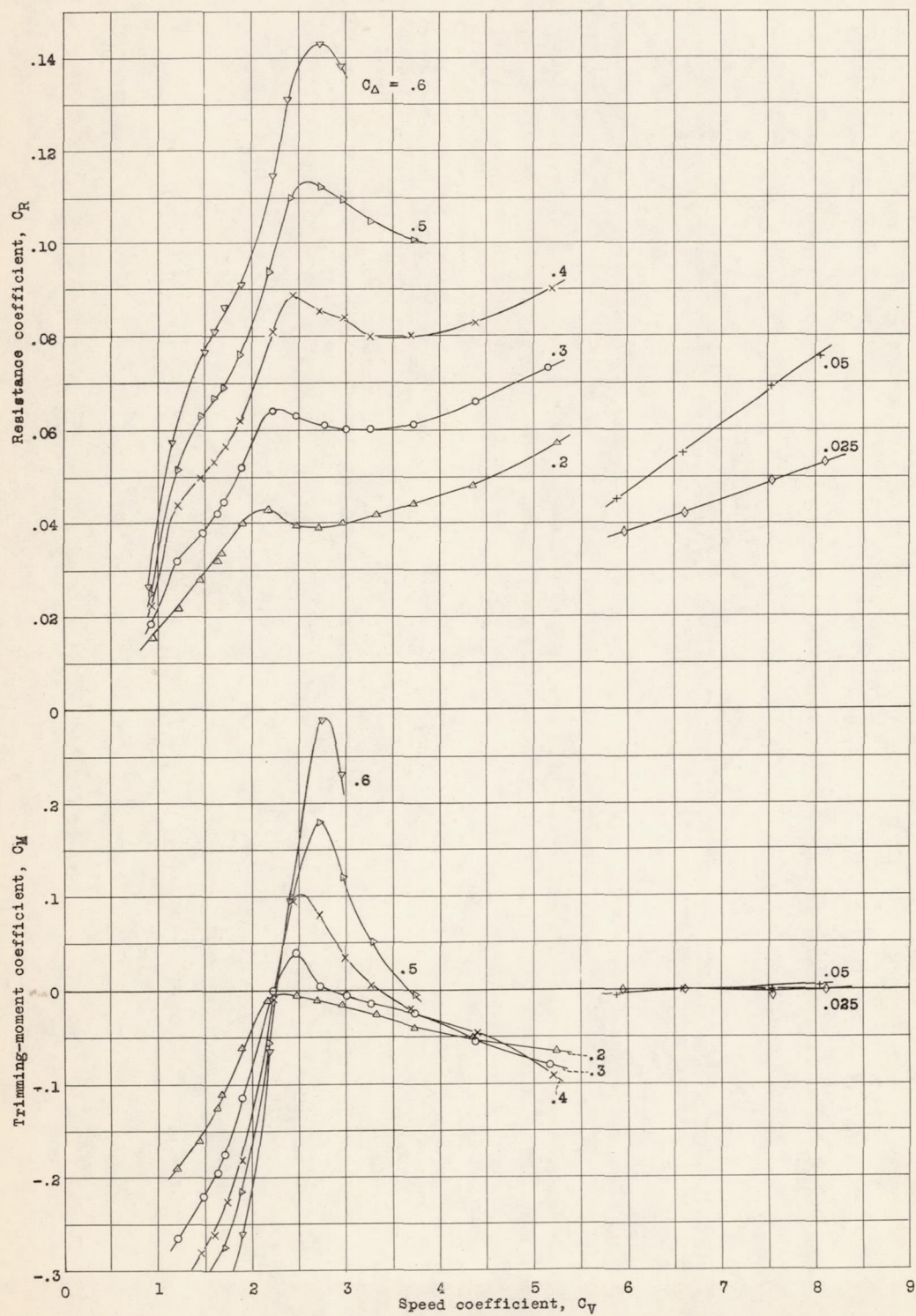
Figure 7.-Resistance coefficient and trimming-moment coefficient. \tau = 9^\circ
