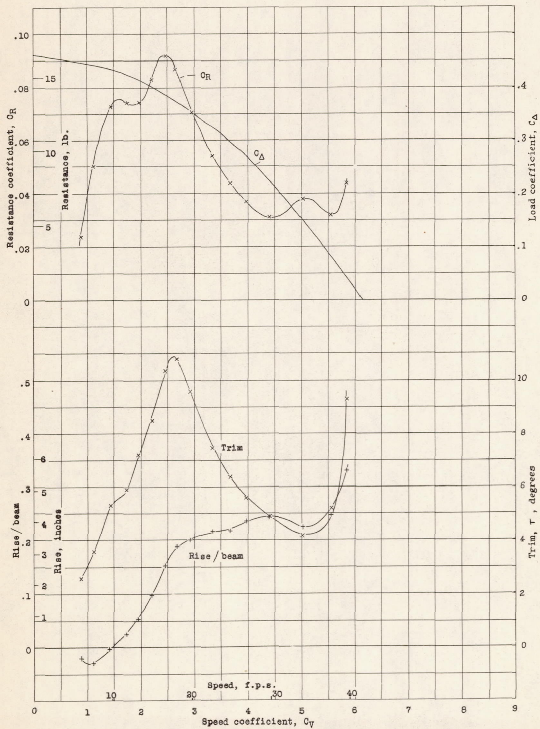
Figure 14.- Resistance coefficient, trim, and rise/beam. Specific free-to-trim test.
