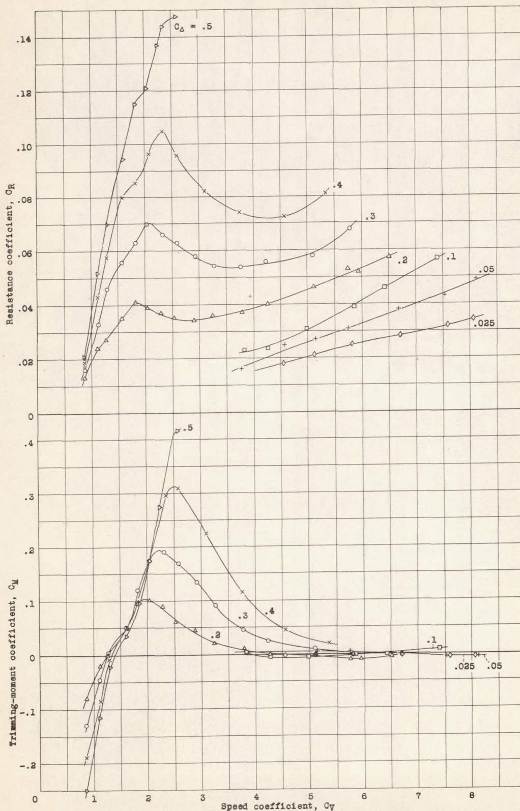
Figure 5.-Resistance coefficient and trimming-moment coefficient. \tau = 5^\circ
