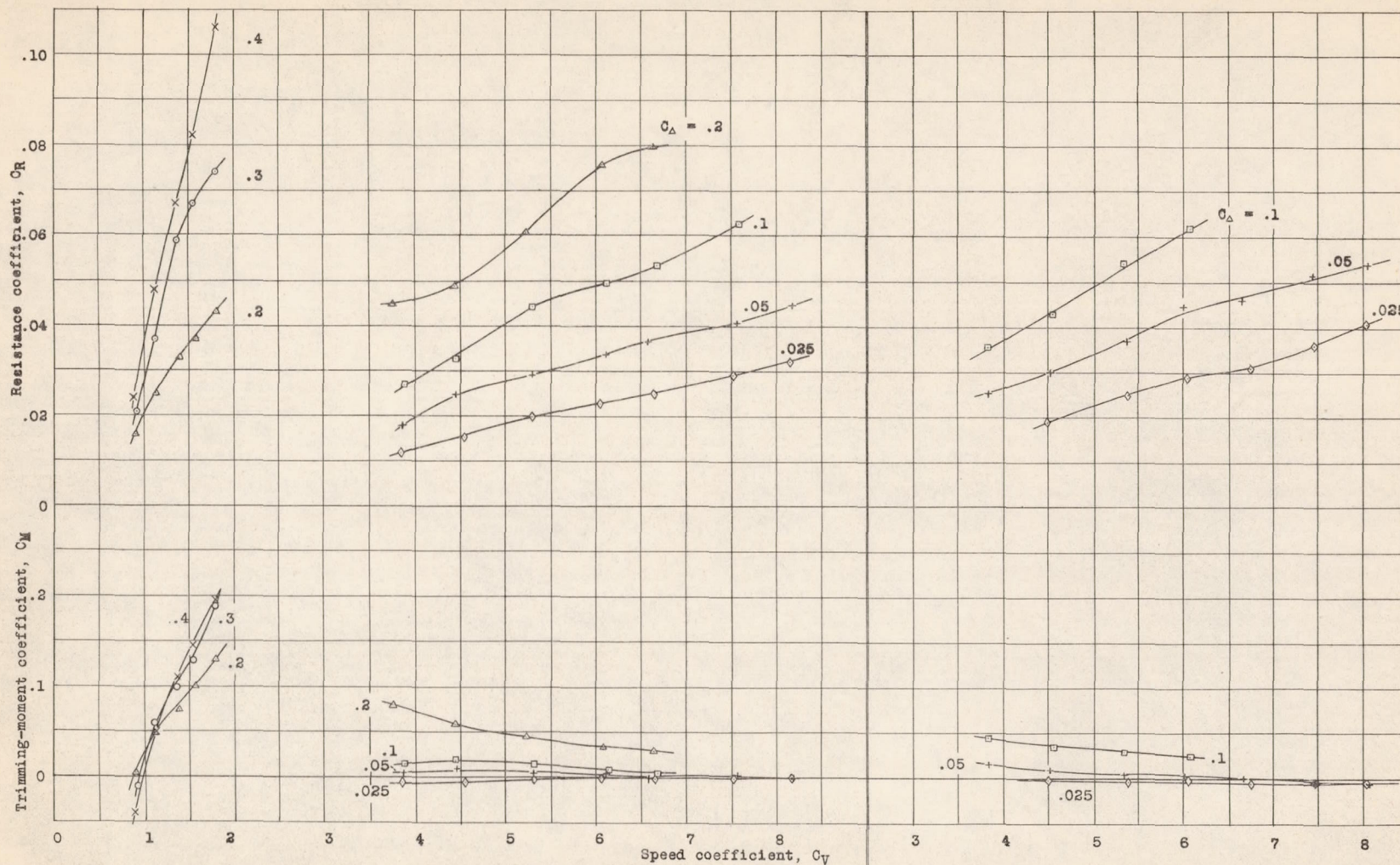
Figure 4.-Resistance coefficient and trimming-moment coefficient, \tau = 3^\circ .
