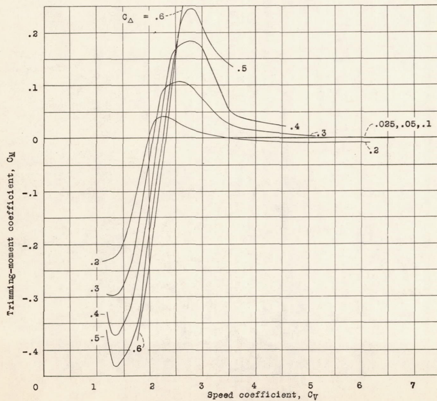
Figure 10.-Variation of C_M with C_V at best trim.
