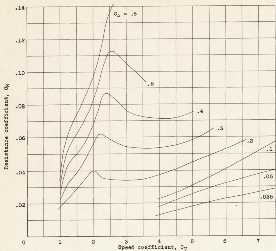
Figure 9.-Variation of C_R with C_V at best trim.
