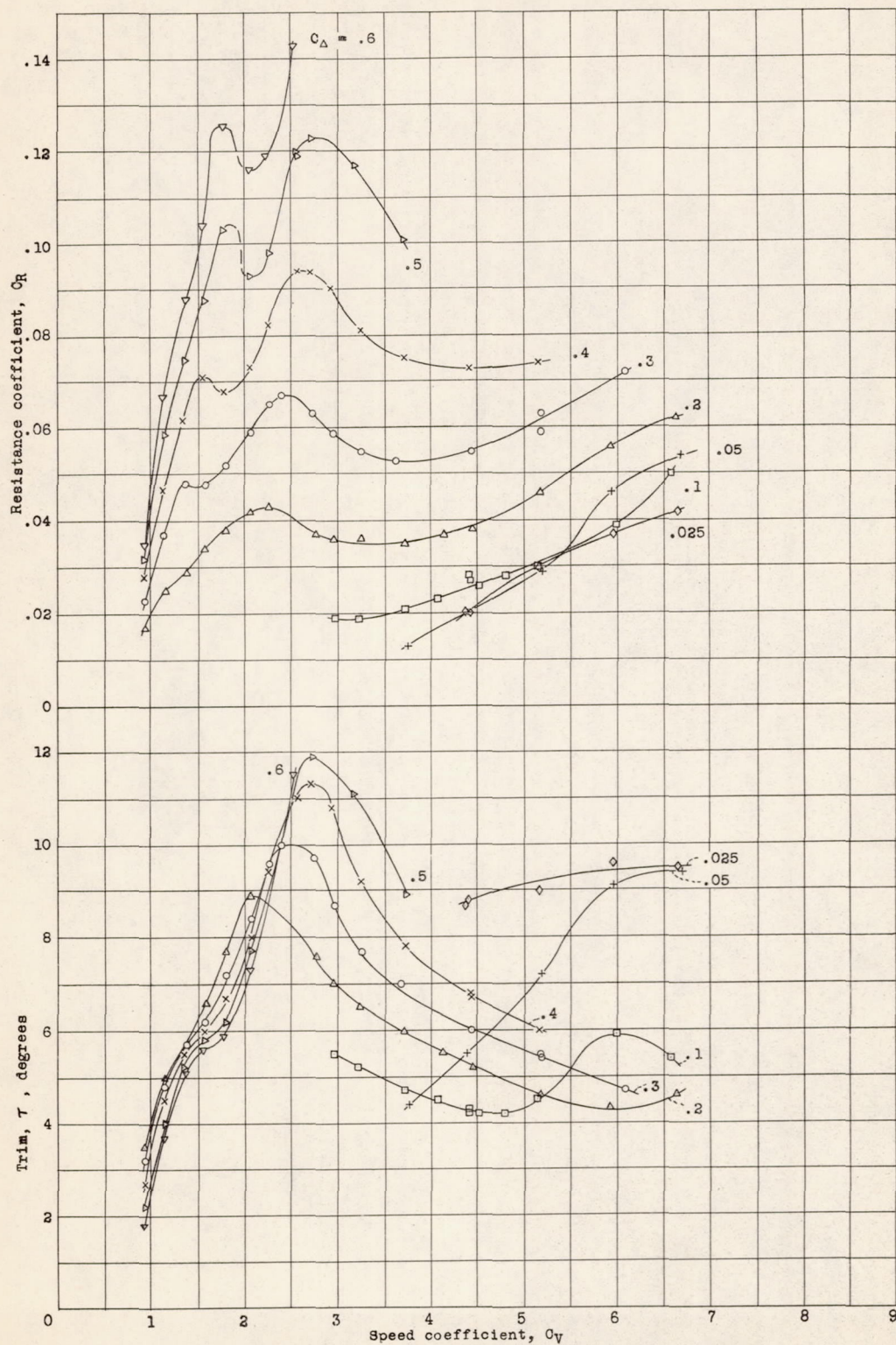
Figure 13.- Resistance coefficient and trim. General free-to-trim test.
