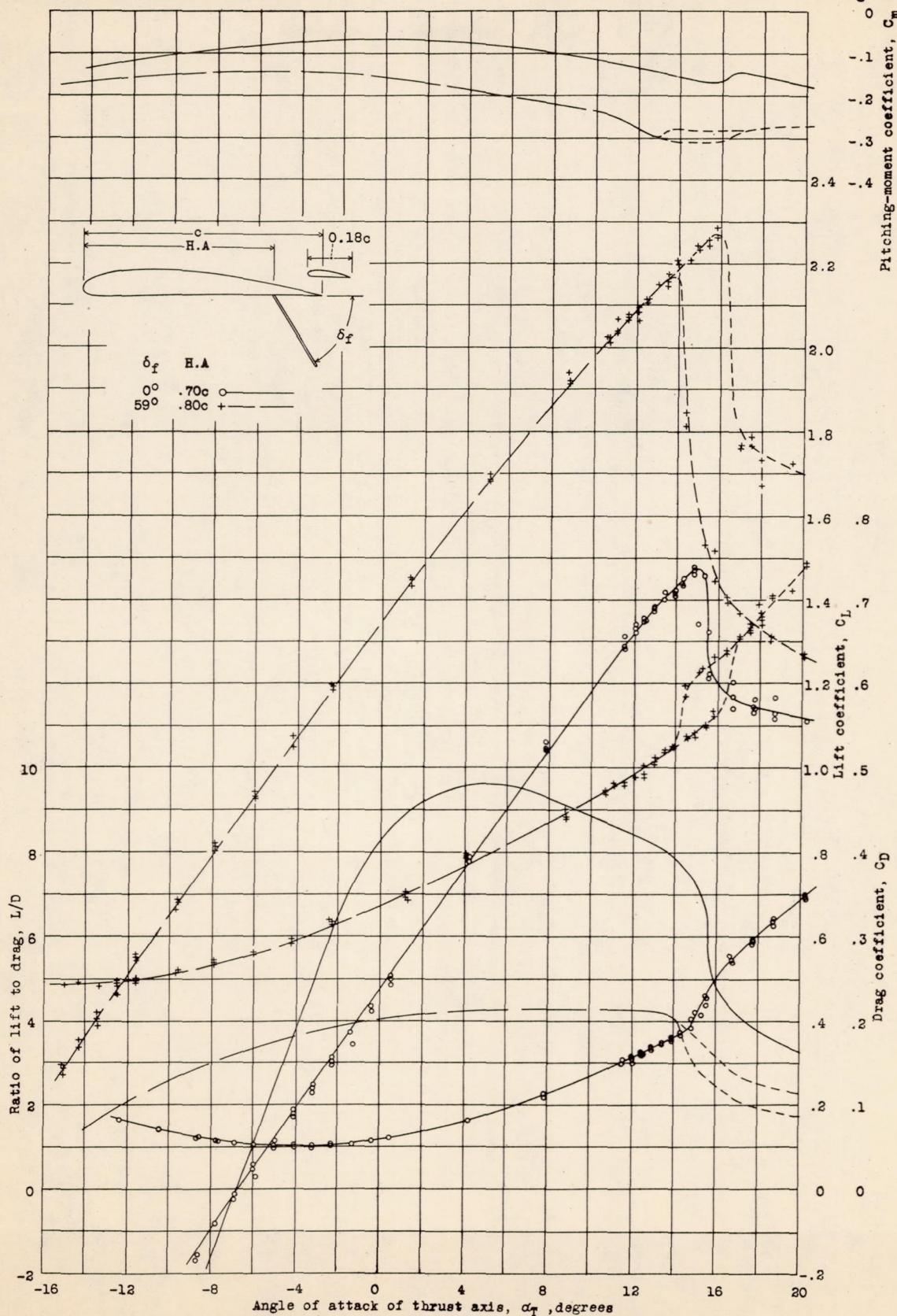
Figure 9.- Aerodynamic characteristics of Fairchild 22 airplane with 0.30c Zap flaps and 0.22c Zap ailerons. Ailerons set 3^\circ relative to the wing chord; propeller and horizontal tail surfaces removed; results corrected for wind-tunnel effects; test velocity, approximately 57 m. p. h.
