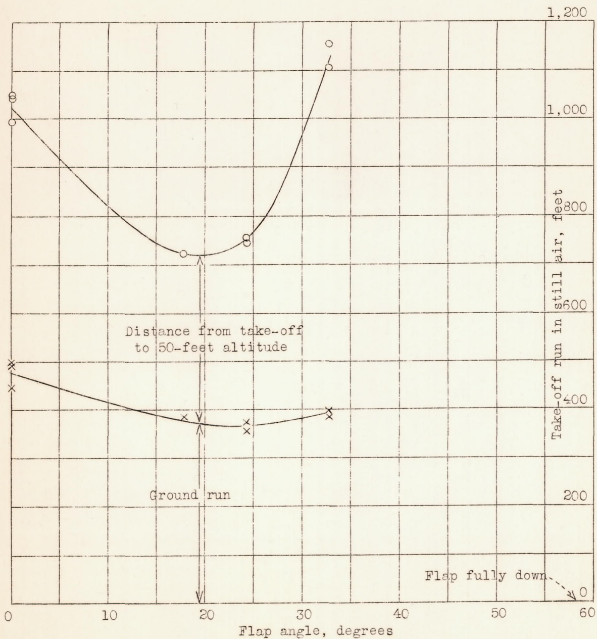
Figure 19.- Variation of take-off run with Zap flap setting on Fairchild 22 airplane.
