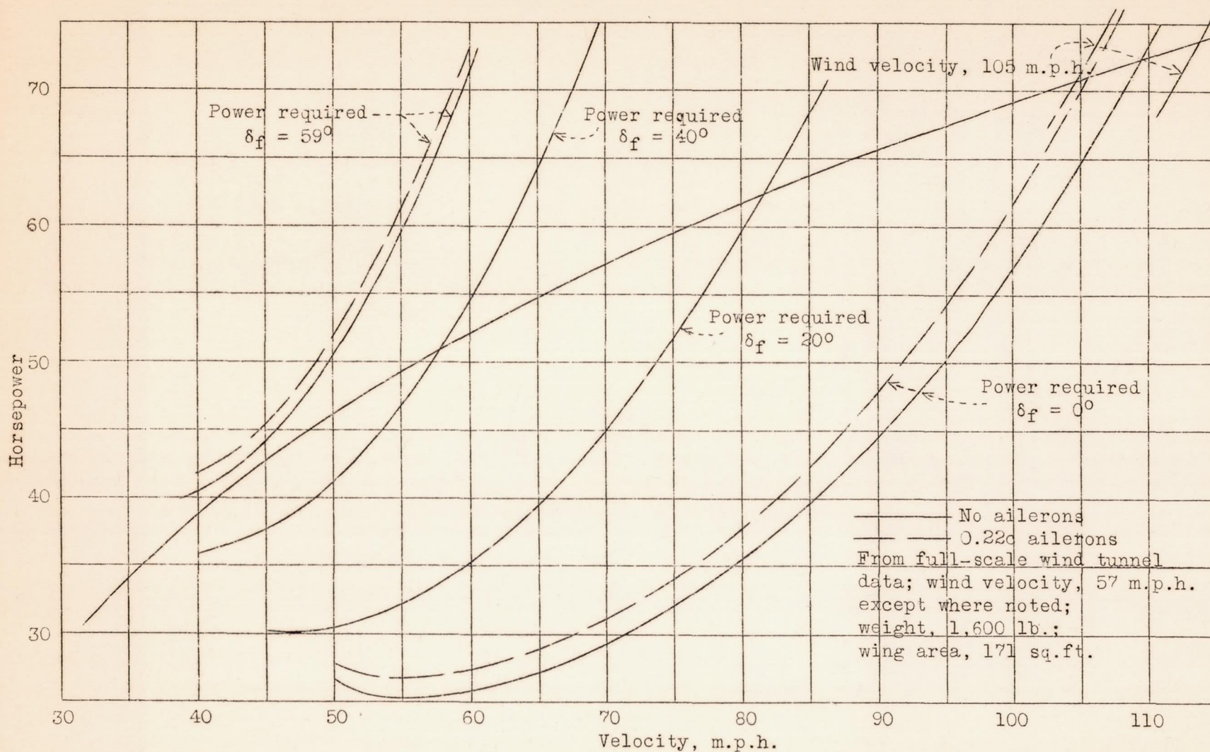
Figure 15.- Horsepower curves for Fairchild 22 airplane with Zap wing.
