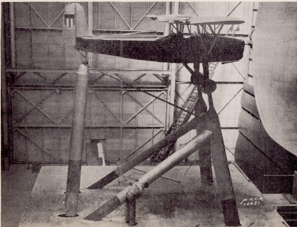
Figure 5.- Fairchild 22 airplane with Zap wing mounted in the full-scale wind tunnel.
