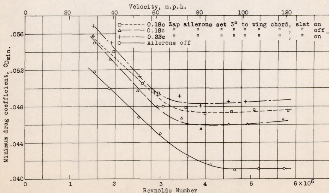
Figure 11.- Scale effect on the minimum drag coefficient of the Fairchild 22 airplane with flaps up. Propeller and horizontal tail surfaces removed; results corrected for wind-tunnel effects.
