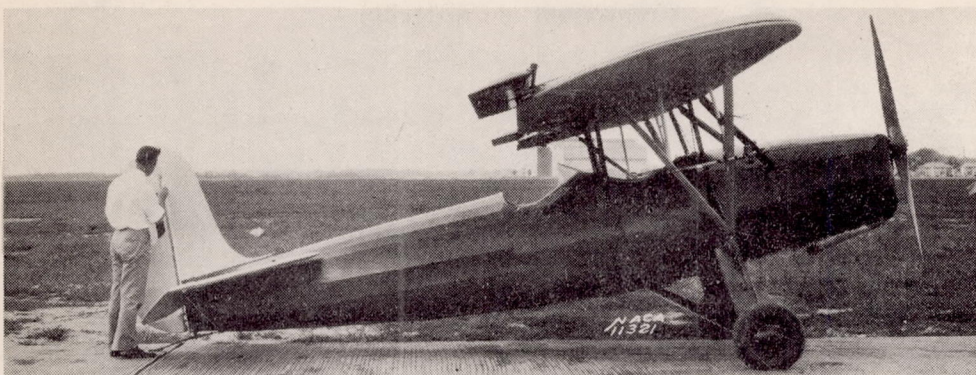
Figure 3.- Fairchild 22 airplane with Zap flaps in the up position.
