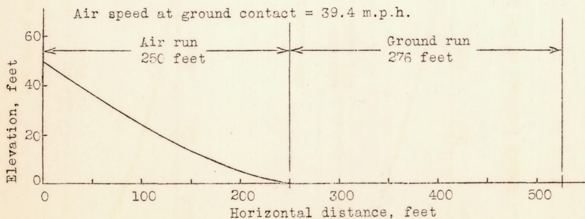
Figure 21.- Normal landings of the Fairchild 22 airplane with the Zap flap down.
