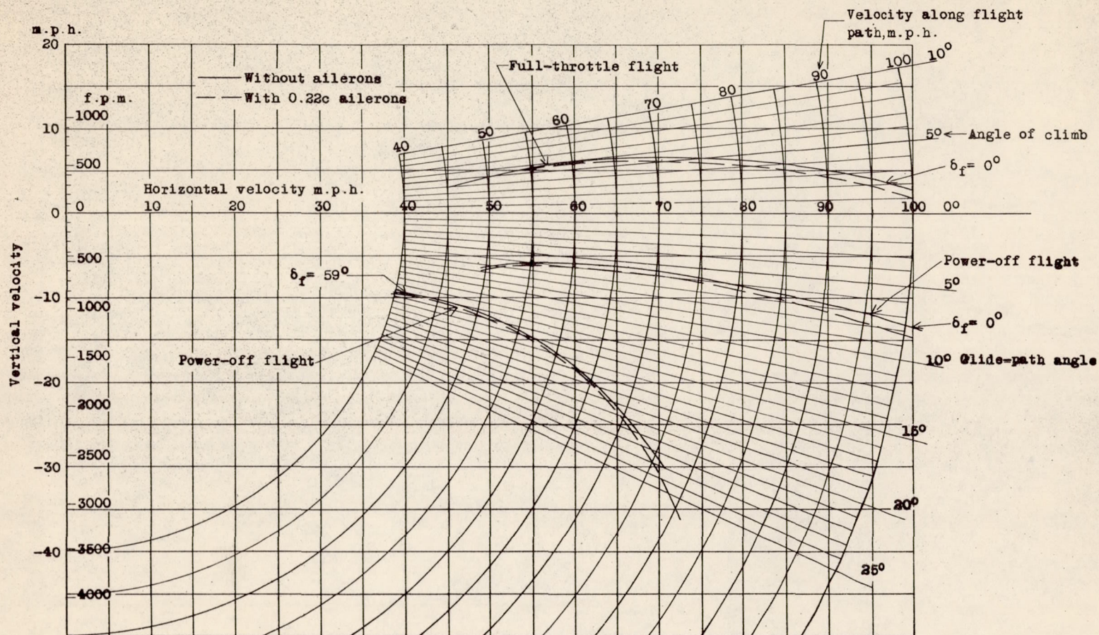
Figure 14.- Velocity diagram for Fairchild 22 airplane with Zap wing. From full-scale wind-tunnel data; wind velocity, 57 m.p.h.; weight, 1600 lb.; wing area, 171 sq. ft.
