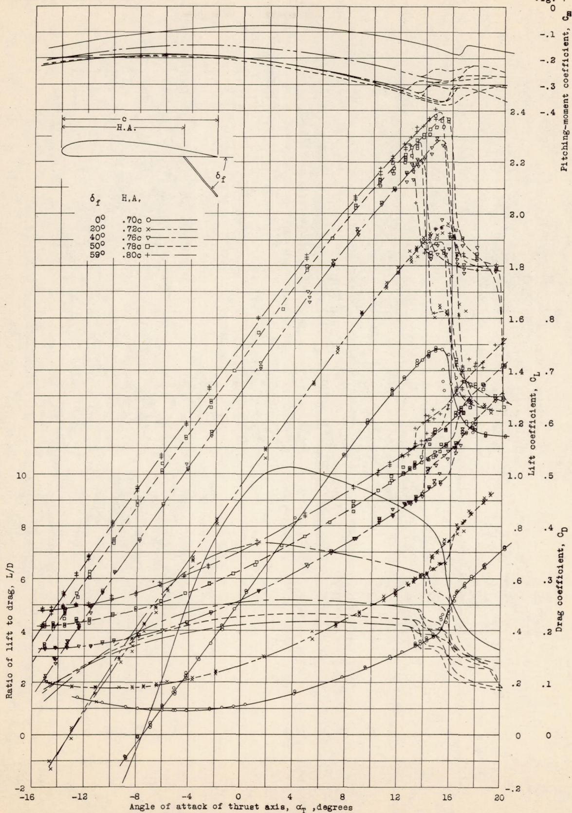
Figure 7.- Aerodynamic characteristics of Fairchild 22 airplane with 0.30c Zap flaps. Ailerons, propeller, and horizontal tail surfaces removed; results corrected for wind-tunnel effects; test velocity, approximately 57 m. p. h.
