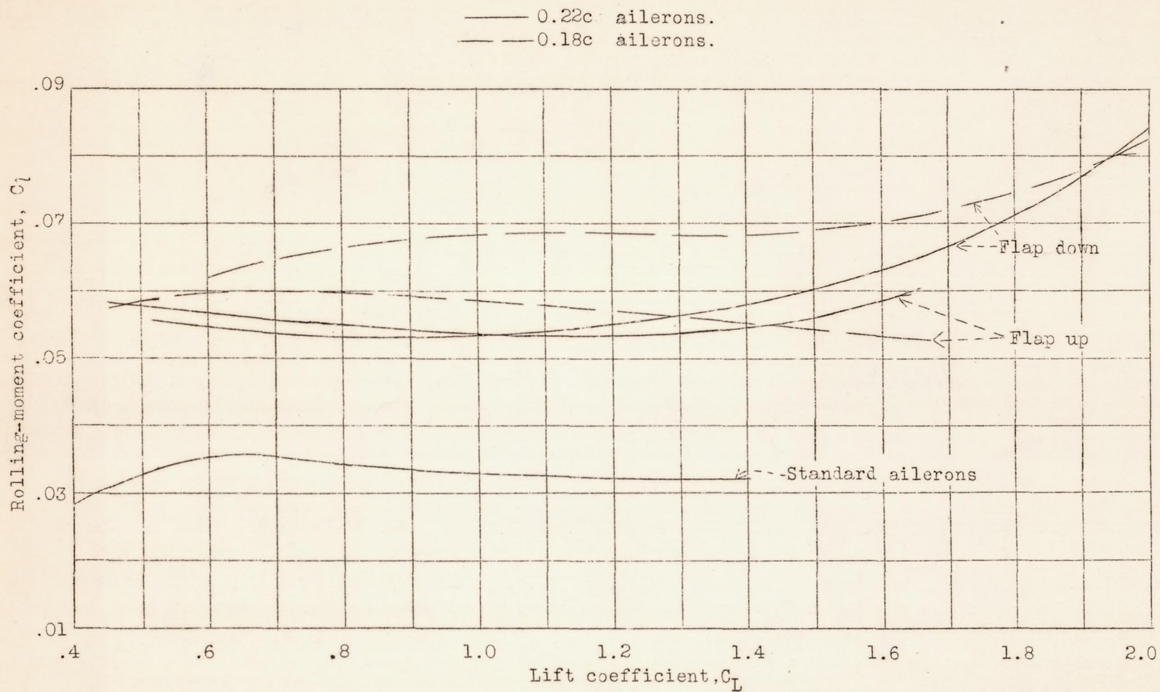
Figure 18.- Rolling-moment coefficients for Fairchild 22 airplane with Zap ailerons.
