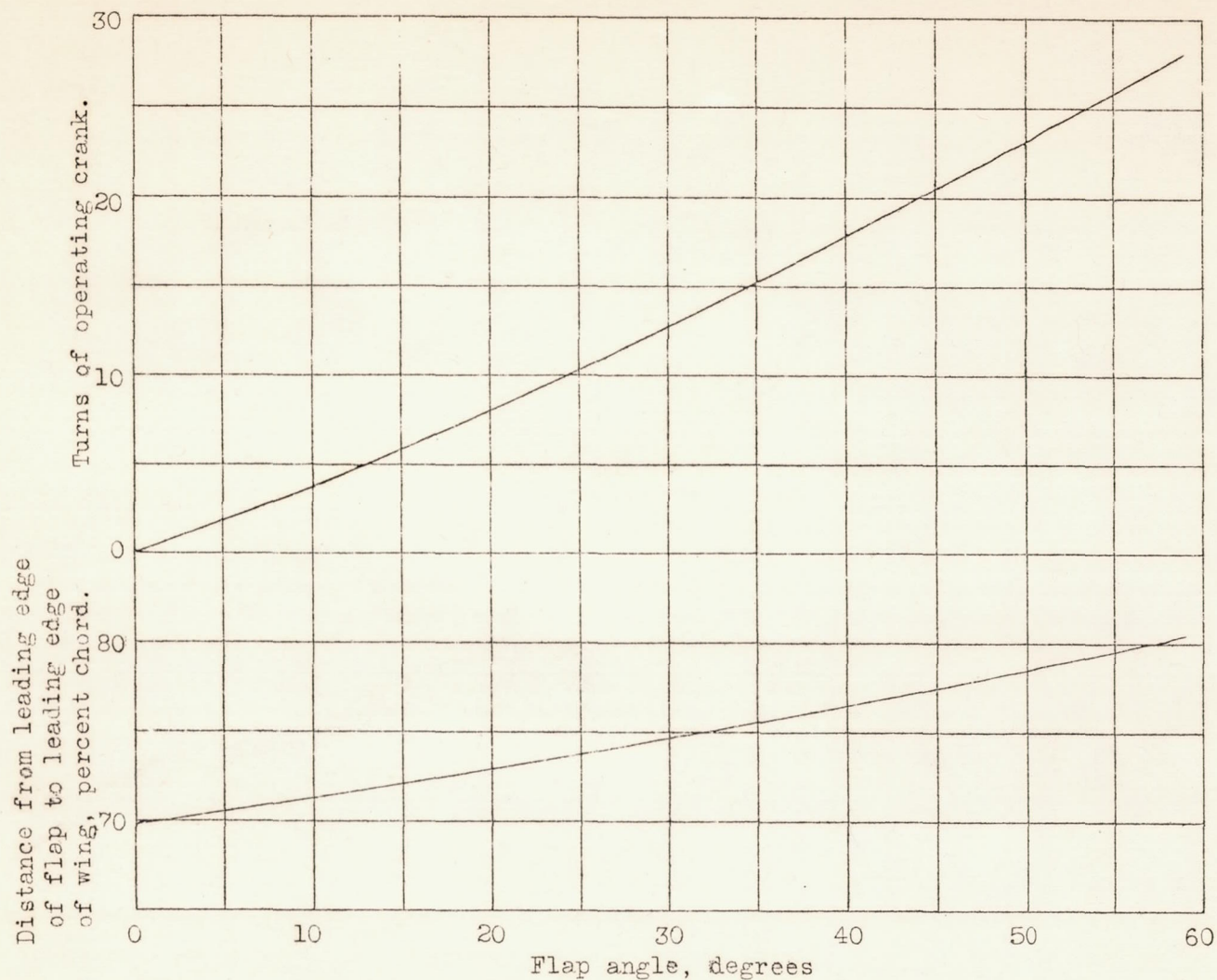
Figure 6.- Relation of flap position and turns of operating crank to flap angle for Zap wing on Fairchild 22 airplane.
