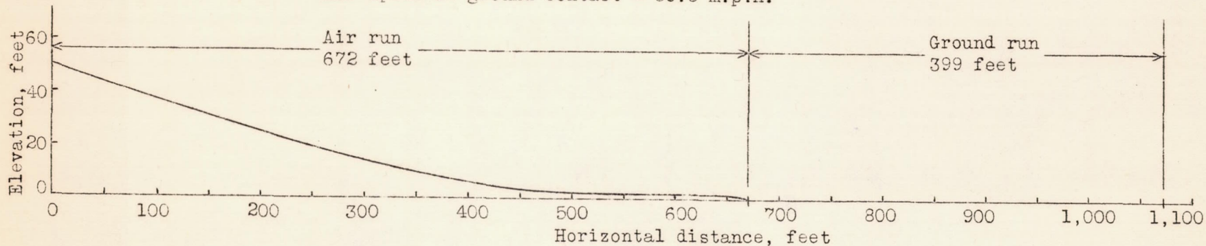
Figure 20.- Normal landings of the Fairchild 22 airplane with the Zap flap up.
