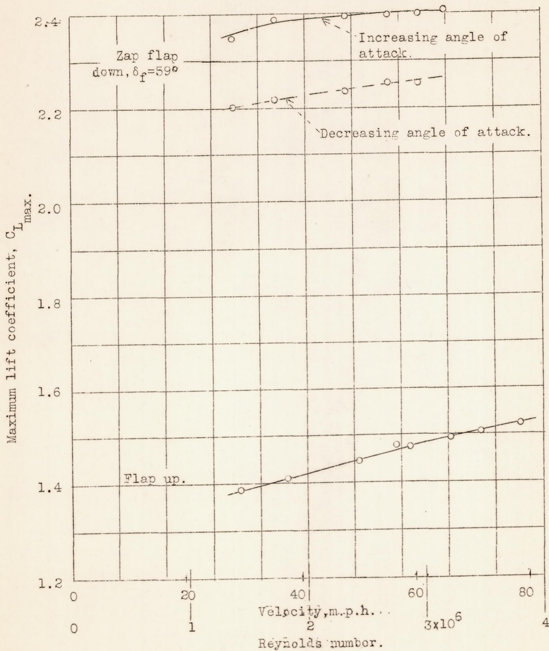
Figure 13.- Scale effect on the maximum lift coefficient of the Fairchild 22 airplane. Ailerons, propeller, and horizontal tail surfaces removed; results corrected for wind-tunnel effects.
