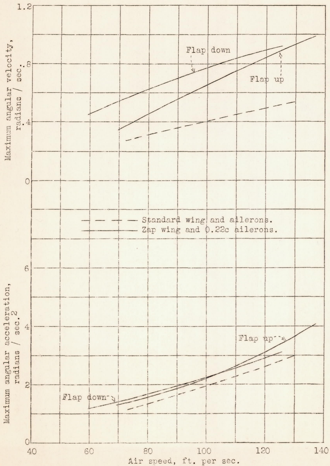
Figure 17.- Maximum rolling accelerations and velocities obtained with 0.22c Zap ailerons on Fairchild 22 airplane.
