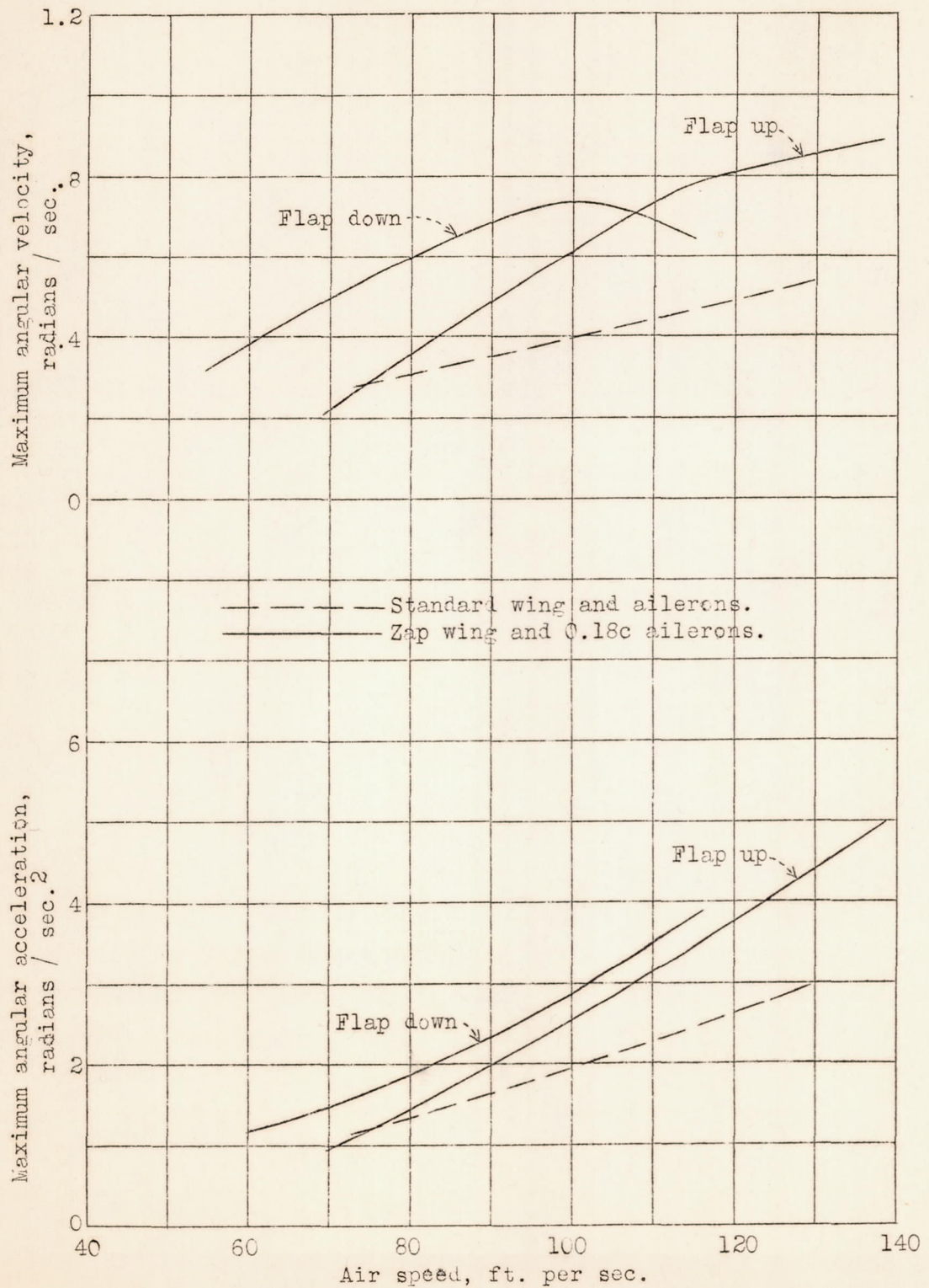
Figure 16.- Maximum rolling accelerations and velocities obtained with 0.18c Zap ailerons on Fairchild 22 airplane.
