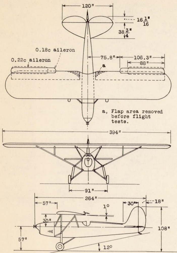
Figure 1.- Three-view drawing of Zap wing installation on Fairchild 22 airplane.
