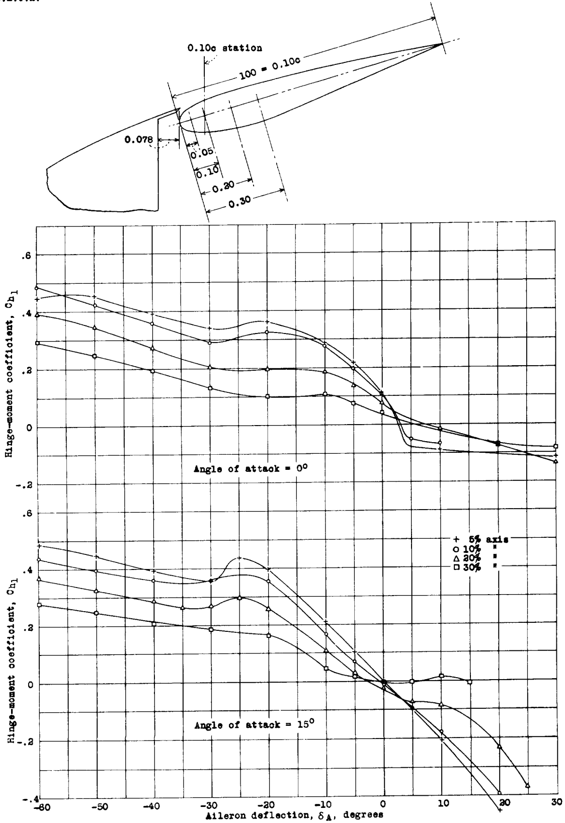
Figure 19.- Hinge-moment coefficients of a slot-lip aileron at 0.10c with 0.078 aileron chord clearance with 0.04c gap and 0.07c width and various aileron-hinge axes.
