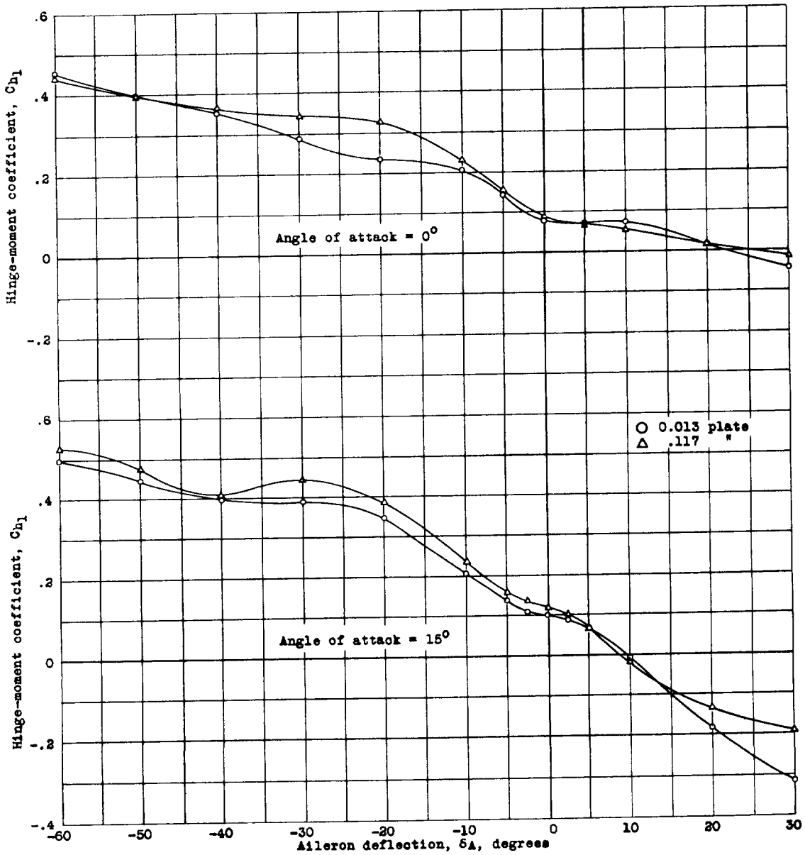
Figure 12.-- Hinge-moment coefficients of a slot-lip aileron at 0.30 chord with a slot with a straight front wall with a clearance of 0.13 aileron chord and a slot gap 0.042c and slot width 0.086c.
