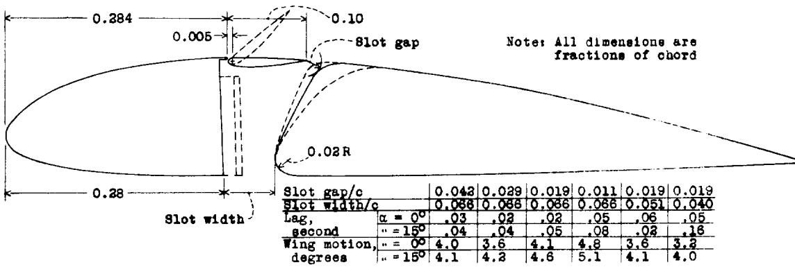
Figure 13.- Lag and rolling moment due to a slot-lip aileron at 0.30 chord with a straight front wall with a clearance of 0.078 aileron chord with several slot gaps and widths.
