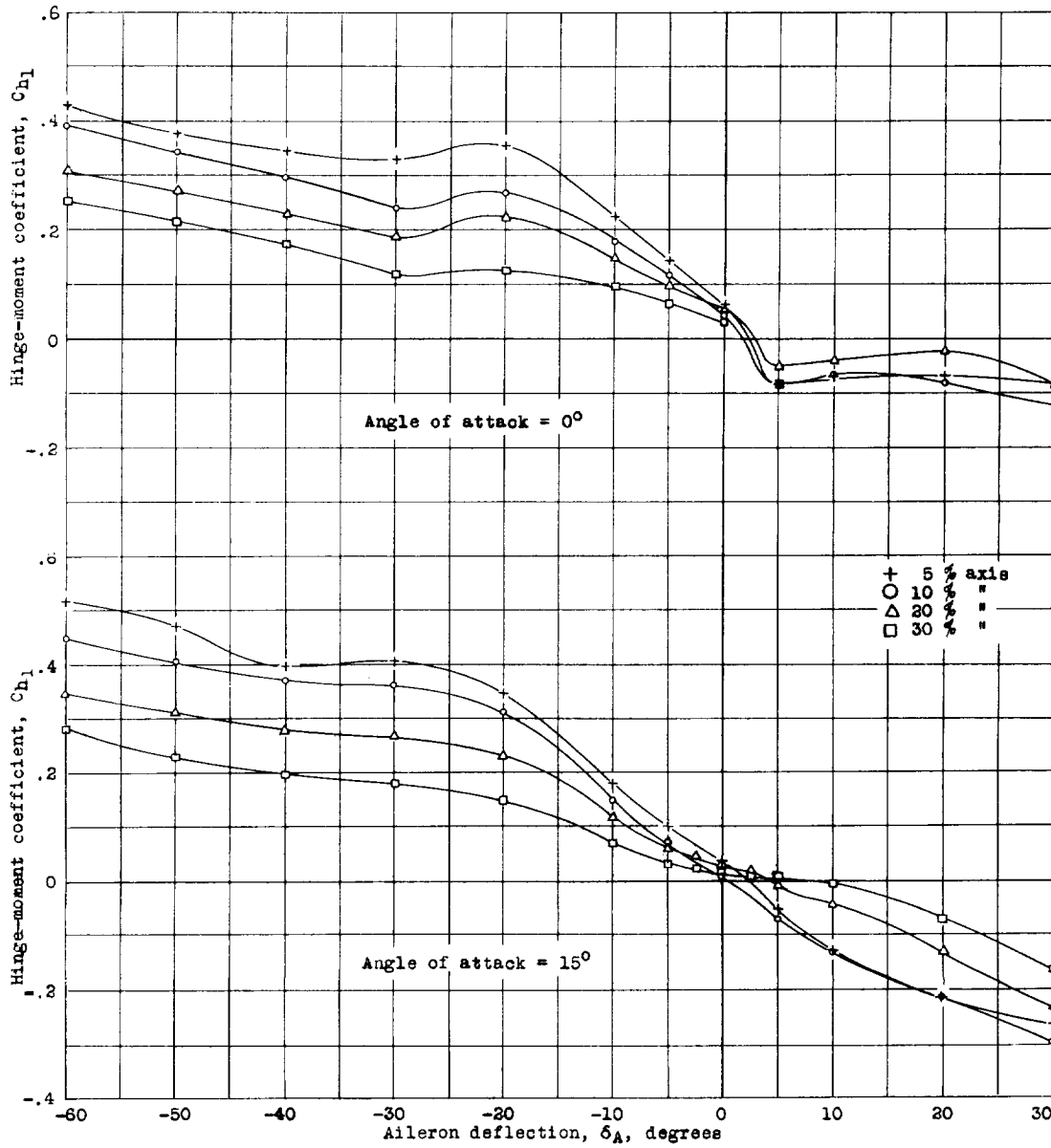
Figure 15.- Hinge-moment coefficients of a slot-lip aileron at 0.30 chord with 0.078 aileron chord clearance with slot gap 0.03c and width 0.06c with various aileron-hinge axes.
