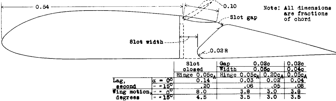
Figure 16.- Lag and rolling moment due to a slot-lip aileron of 0.55 chord with 0.061 aileron chord clearance with slot gap 0.02c and width 0.04c and 0.05c with two different aileron-hinge axes.
