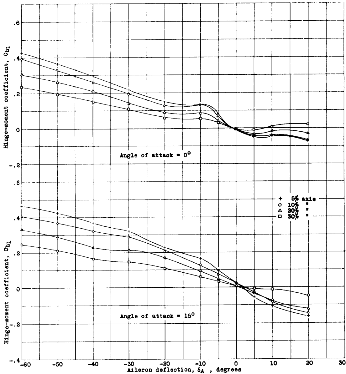
Figure 17.- Hinge-moment coefficients of a slot-lip aileron at 0.55 chord with 0.078 aileron chord clearance with slot gap 0.02c and width 0.05c and various aileron-hinge axes.
