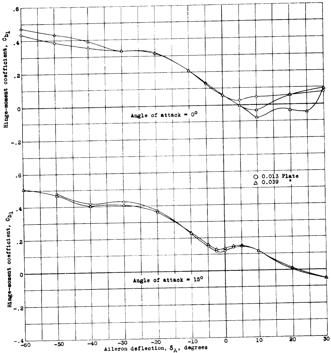
Figure 10.- Hinge-moment coefficients of a slot-lip aileron at 0.30 chord with a slot with a straight front wall with a clearance of 0.026 aileron chord and a slot gap 0.042c and slot width 0.066c.
