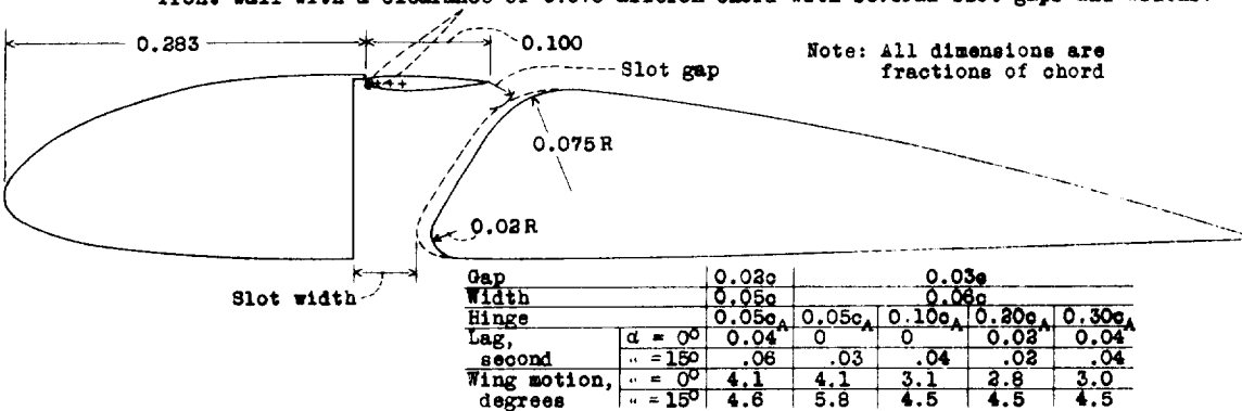
Figure 14.- Lag and rolling moment due to a slot-lip aileron at 0.30 chord with two slot gaps and widths and various hinge axes.
