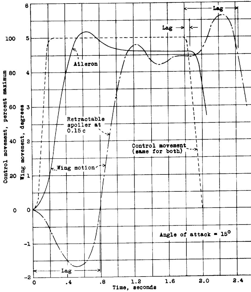
Figure 3.- Typical time history curves.
