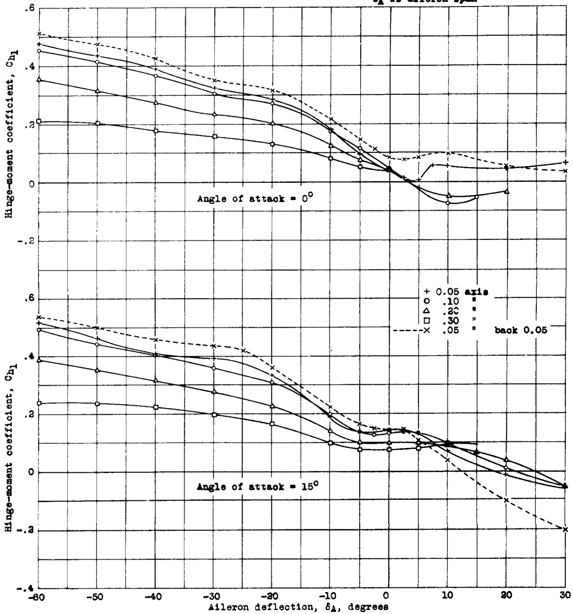
Figure 9.- Hinge-moment coefficients of a slot-lip aileron at 0.30 chord with a special-shape slot of slot gap 0.042c and slot width 0.068c with various aileron hinge-axis positions.
