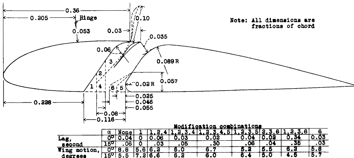
Figure 7.- Effect of various modifications of a fixed slot on the lag and rolling moment due to an adjoining retractable spoiler.
