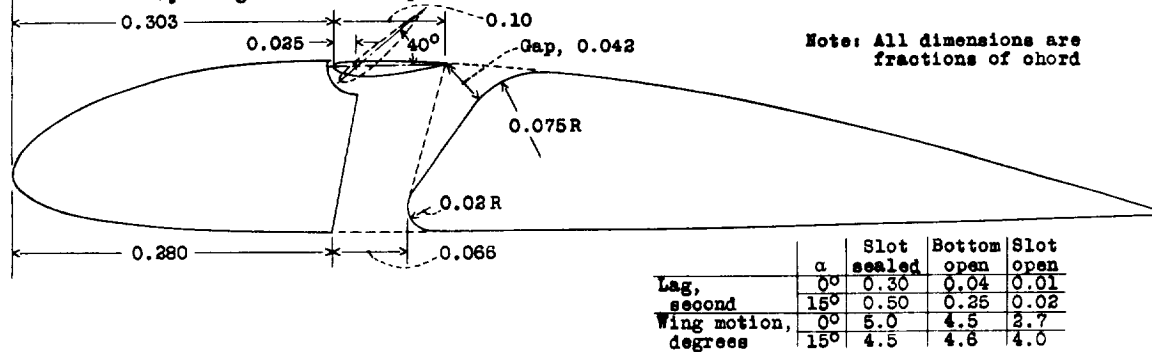
Figure 8.- Lag and rolling moment due to a slot-lip aileron at 0.30 chord with a special-shape slot of slot gap 0.042c and slot width 0.066c with the slot both open and sealed.
