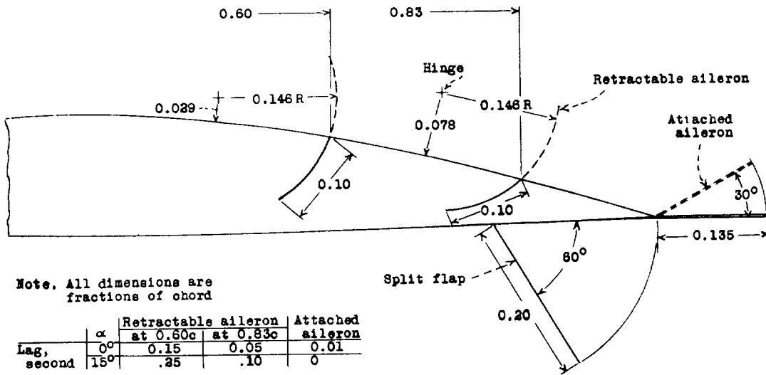
Figure 4.- Effect of a split flap on lag due to retractable spoilers near the trailing edge of the wing.
