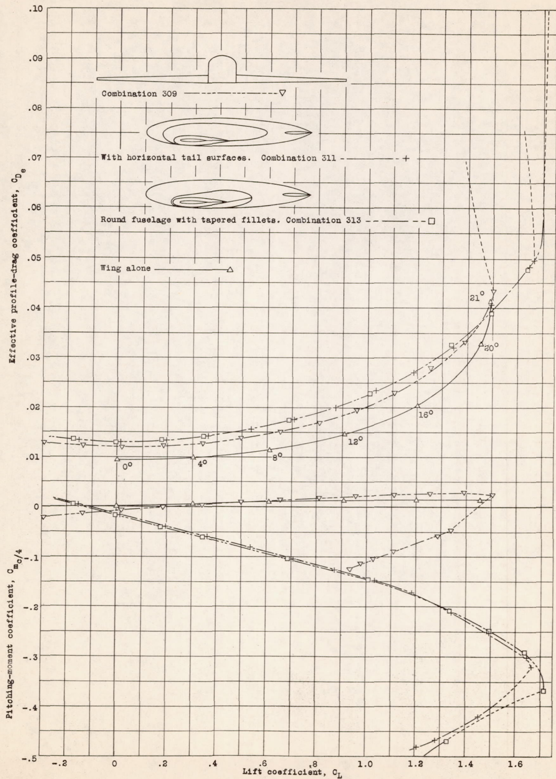
Figure 6. - Characteristics for low-wing combination with straight-side junctures and horizontal tail surfaces; round fuselage, tapered N.A.C.A. 0018-09 airfoil; k/c = -0.22 , i_s = 0^\circ .
