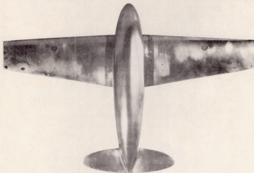
Figure 2. - Combination 309 (Combination 308 inverted) showing cross-section shape of straight-side junctures.
