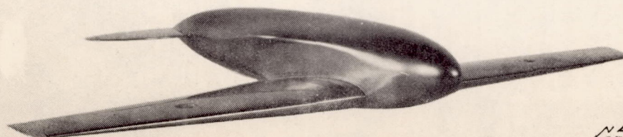
Figure 3. - Combination 311 (Combination 310 inverted) showing straight-side junctures and horizontal tail surfaces
