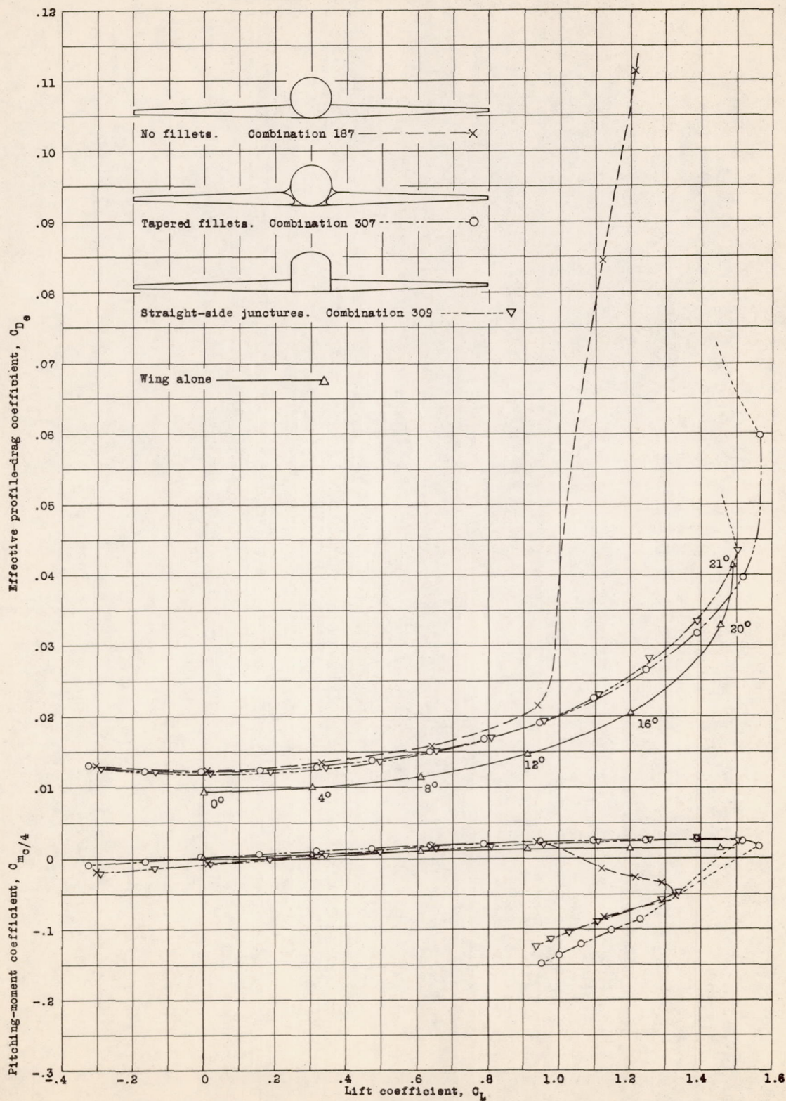
Figure 5. - Effect of straight-side junctures on the low-wing combination; round fuselage, tapered N.A.C.A. 0018-09 airfoil; k/c = -0.22
