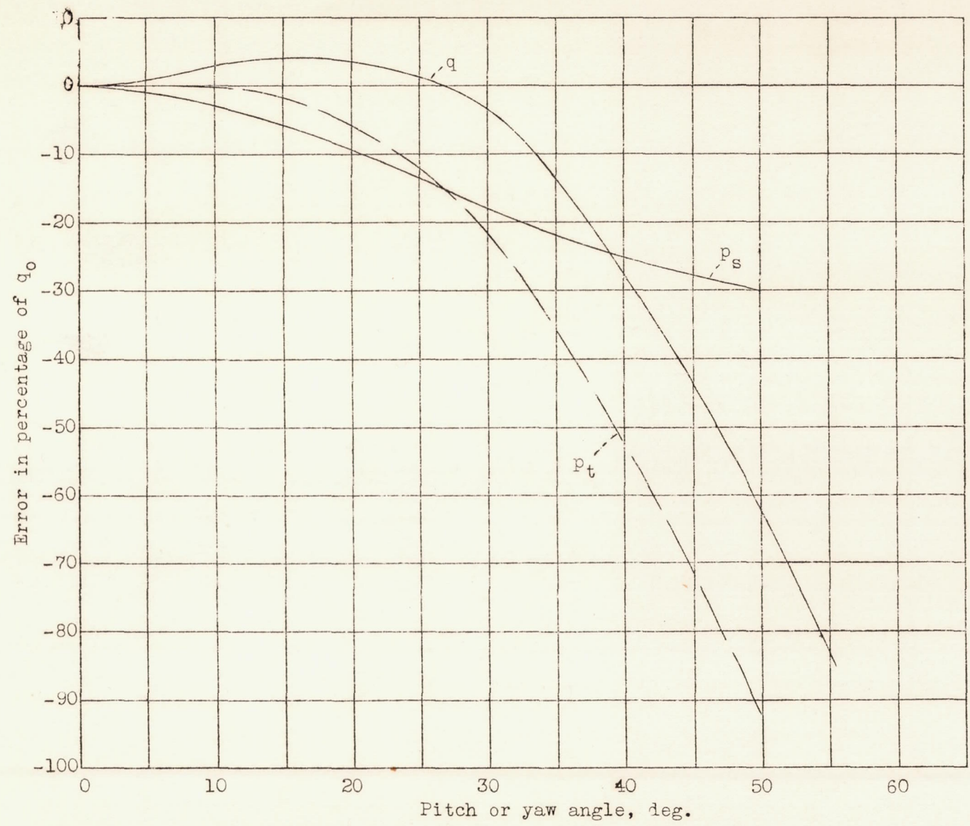
Figure 2.- Typical effect of inclination on pitot-static tube.
