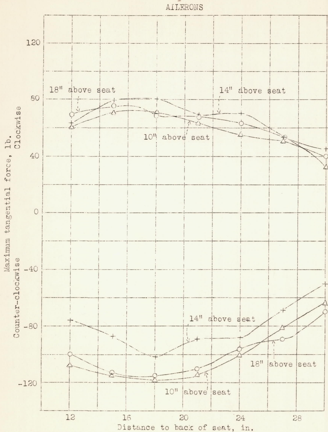
Figure 15.- Variation of tangential force with height of center of 12 inch wheel above seat, pilot secure, grip normal, pilot B.
