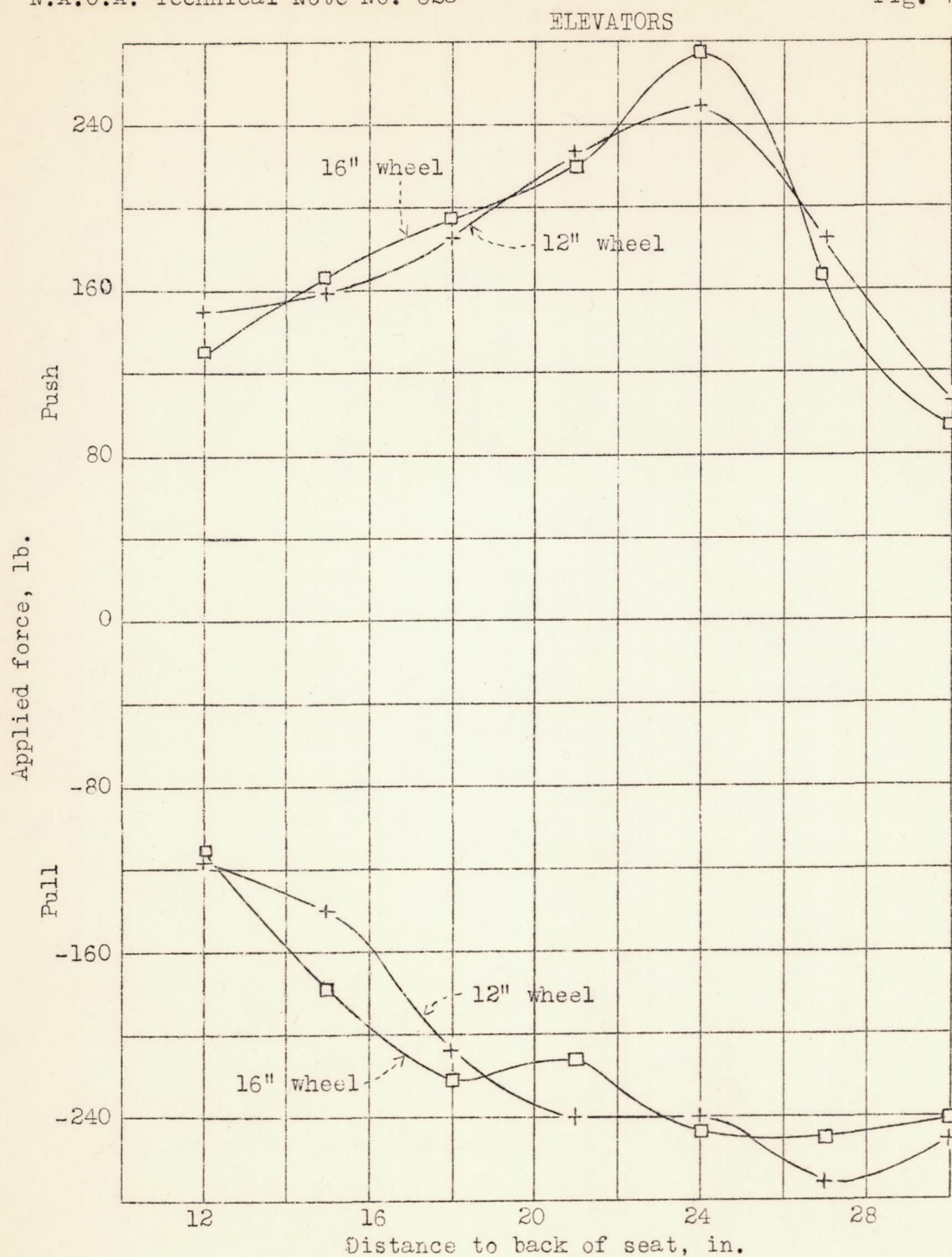
Figure 7.- Variation of push and pull forces with wheel diameter, center of wheel 16 inches above seat, pilot secure, grip normal, pilot B.
