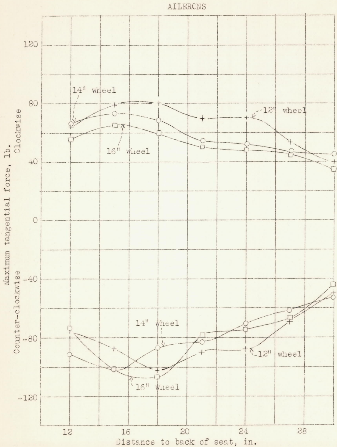
Figure 11.- Variation of tangential force with wheel diameter, 12, 14 and 16 inch wheels, center of wheel 14 inches above seat, pilot secure, grip normal, pilot B.
