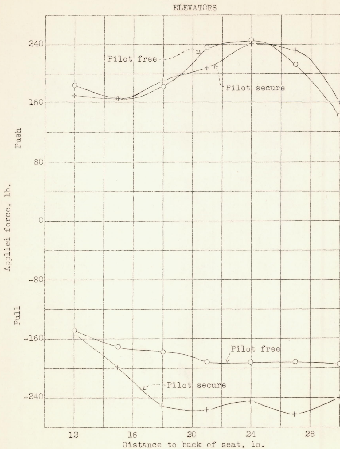
Figure 4.- Variation of push and pull forces with pilot free and pilot secure, 12 inch wheel, center of wheel 16 inches above seat, grip normal, pilot A.
