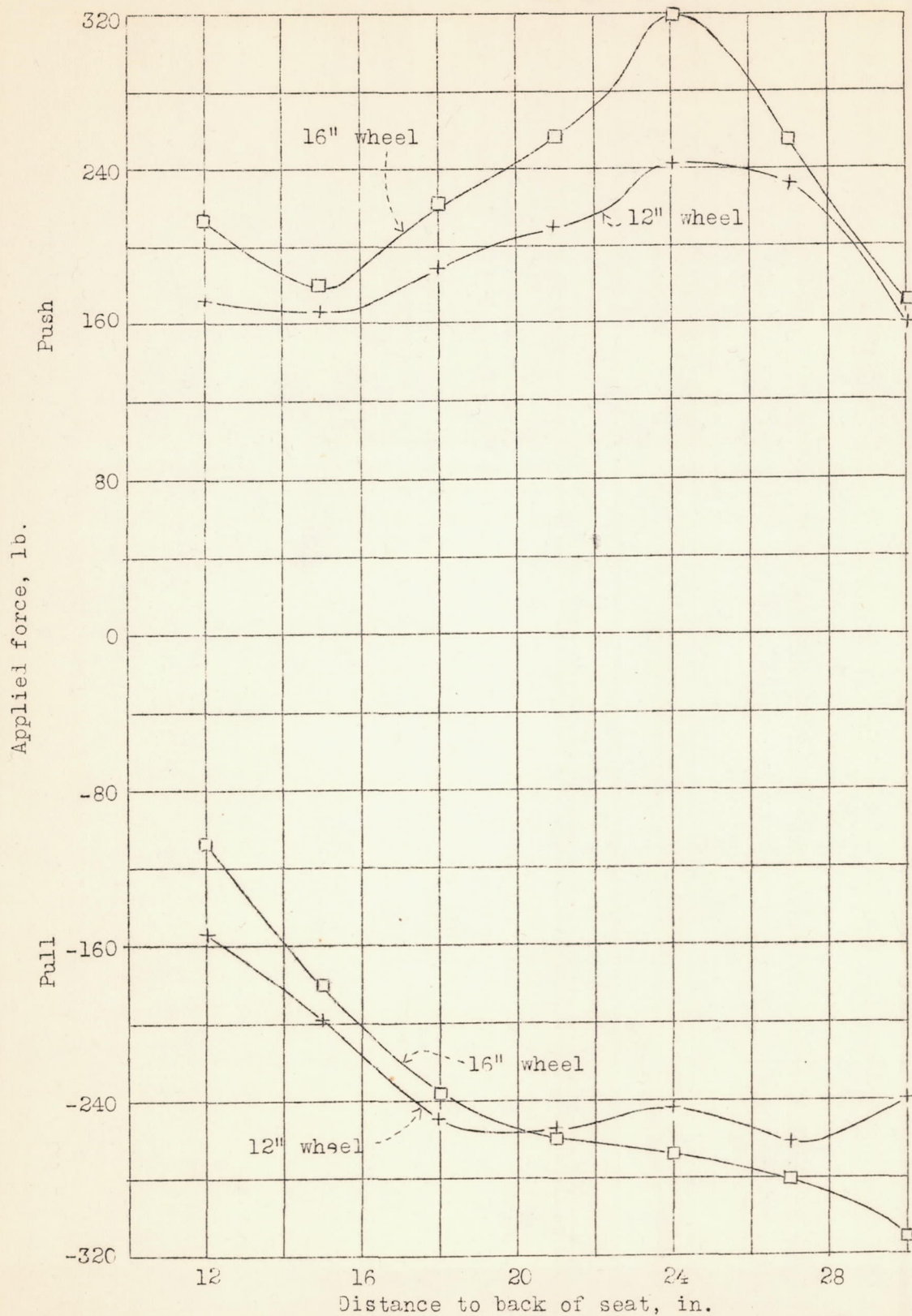
Figure 6.- Variation of push and pull forces with wheel diameter, center of wheel 16 inches above seat, pilot secure, grip normal, pilot A. .
