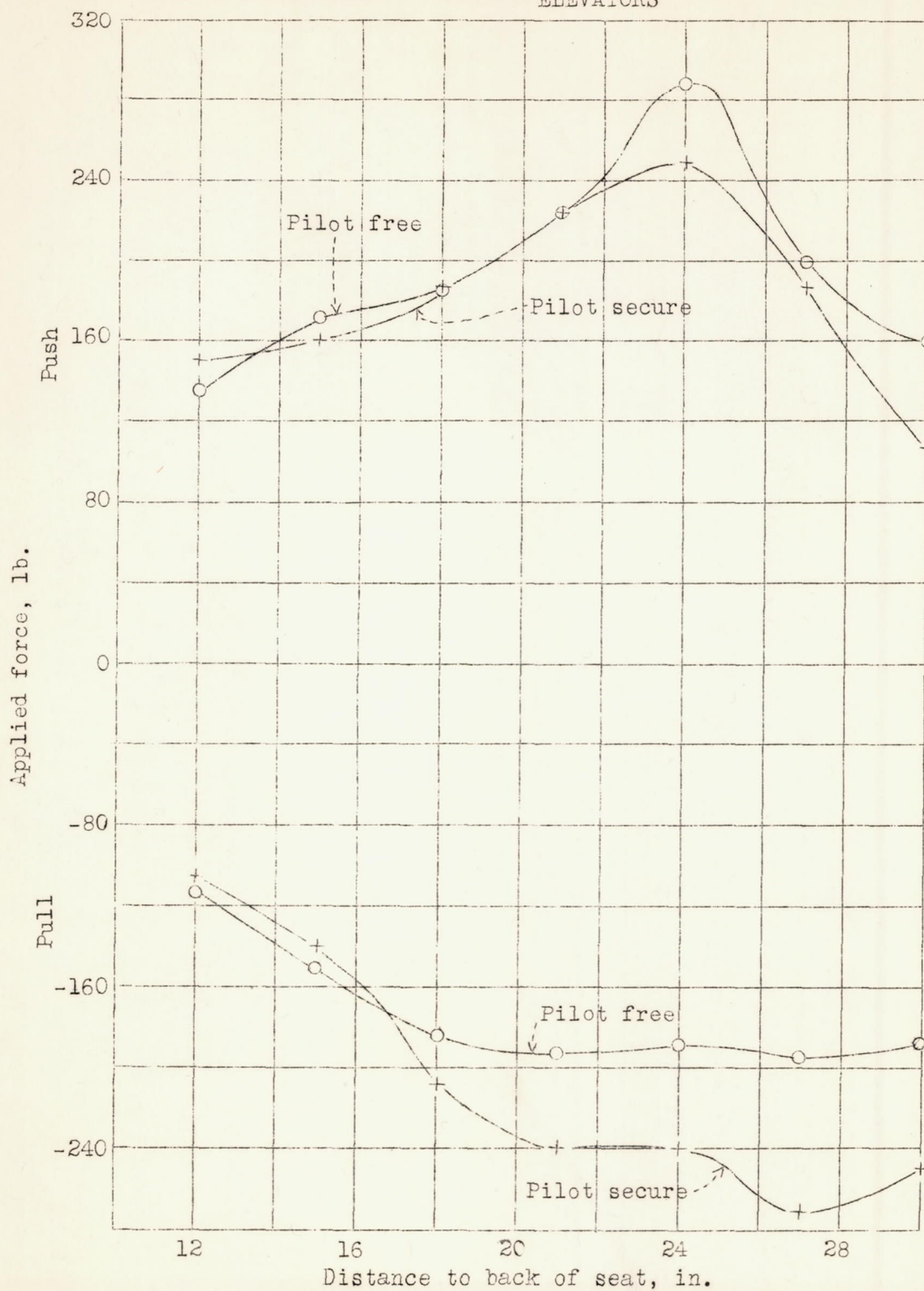
Figure 5.- Variation of push and pull forces with pilot free and pilot secure, 12 inch wheel, center of wheel 16 inches above seat, grip normal, pilot B.
