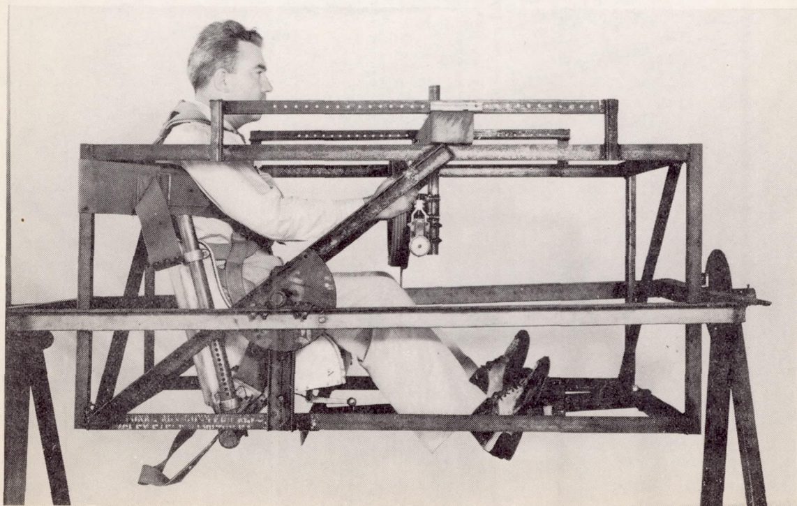
Figure 2.- Set-up for measuring tangential forces.
