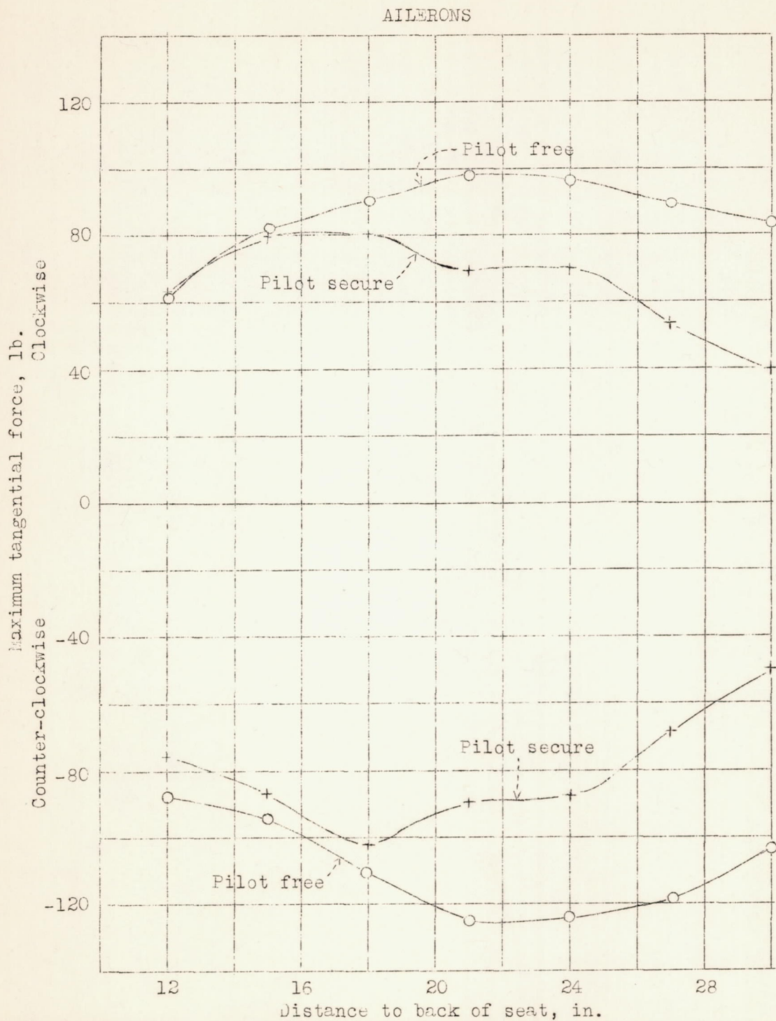
Figure 13.- Variation of tangential force with pilot free and pilot secure, 12 inch wheel, center of wheel 14 inches above seat, pilot B.
