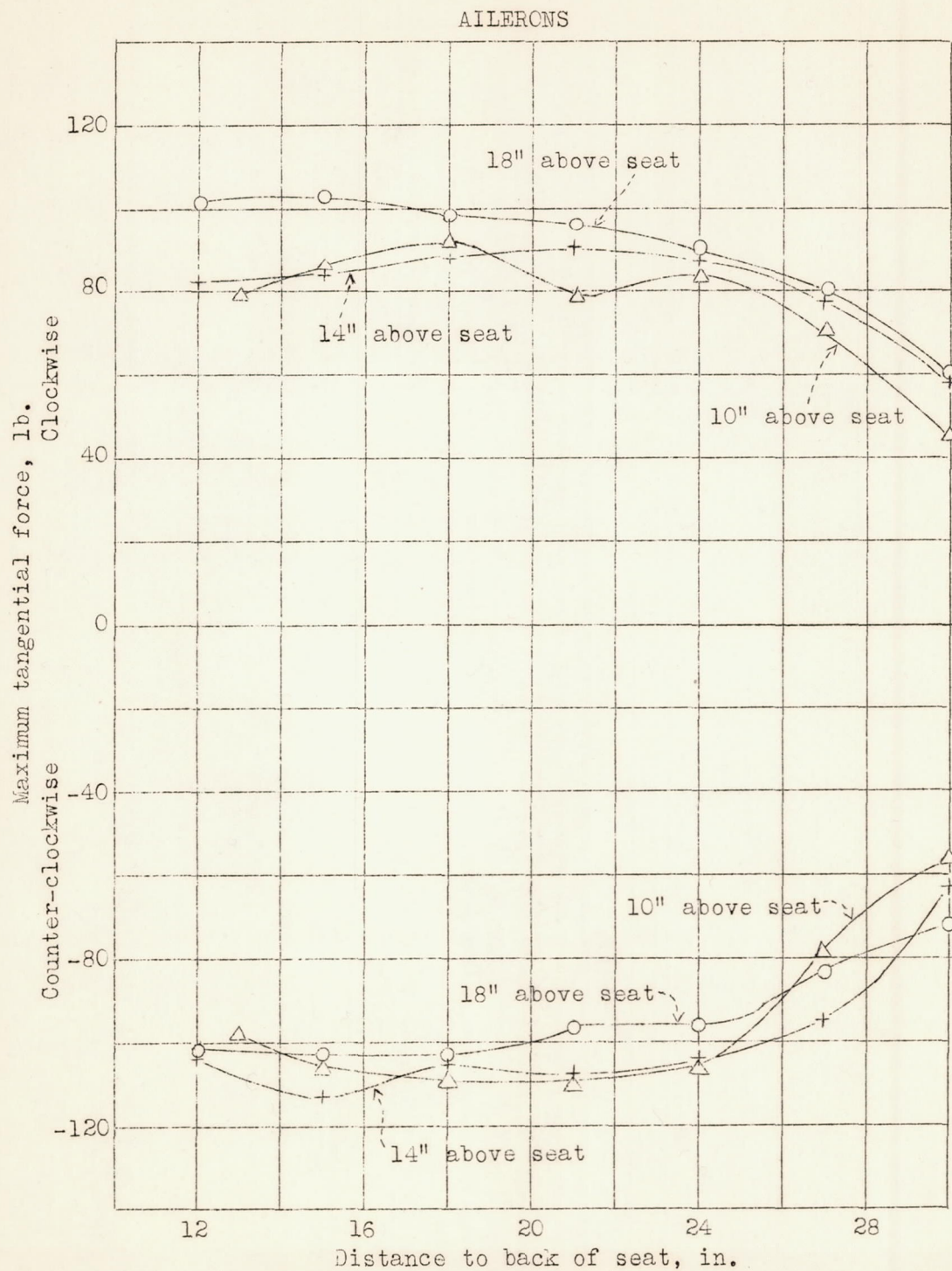
Figure 14.- Variation of tangential force with height of center of 12 inch wheel above seat, pilot secure, grip normal, pilot A.
