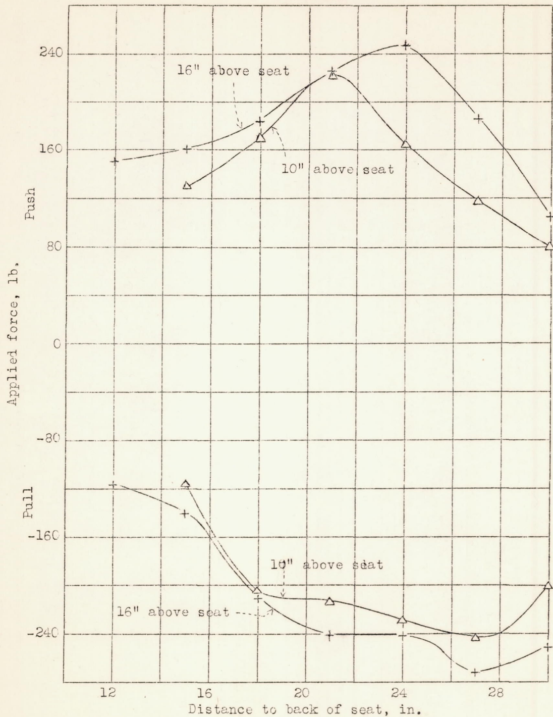
Figure 9.- Variation of push and pull forces with height of center of wheel above seat, 12 inch wheel, grip normal, pilot secure, pilot B.
