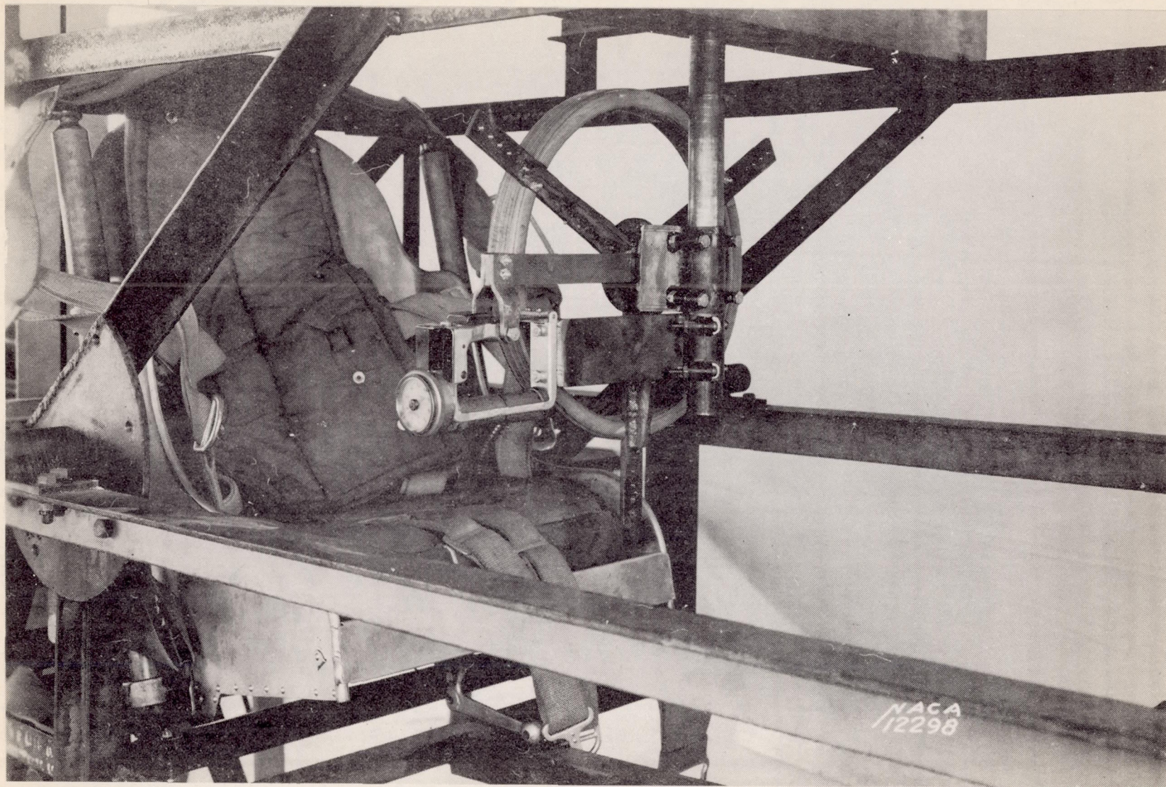
Figure 3.- Detailed view of set-up for measuring tangential forces.
