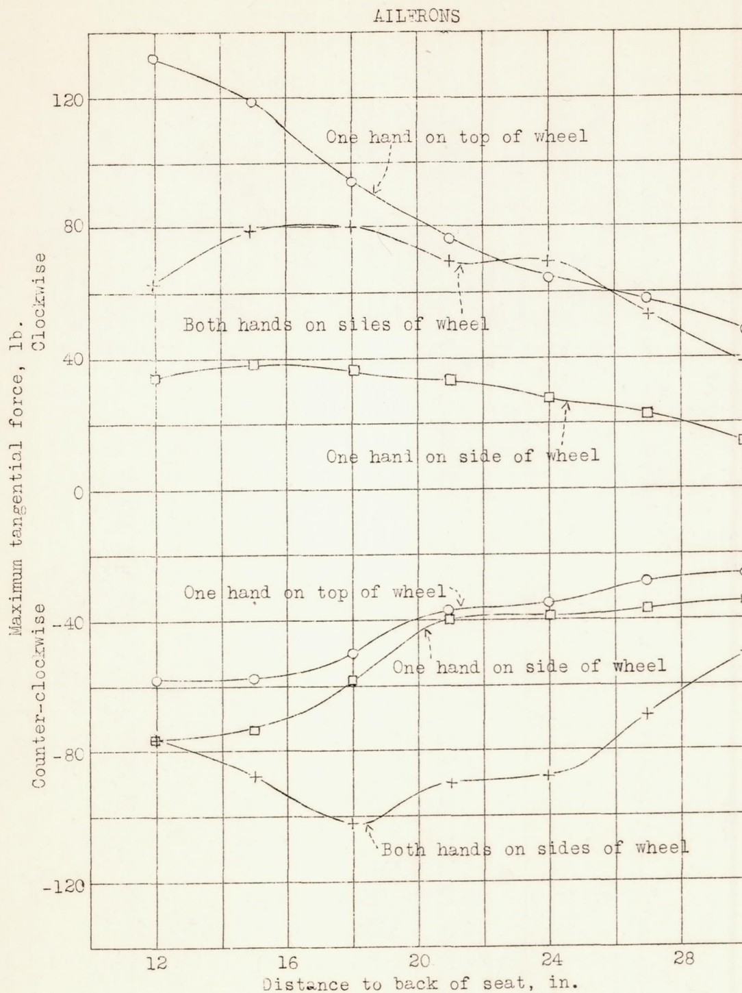
Figure 19.- Variation of tangential force with one hand (right) in two positions on wheel, with both hands, grip normal, 12 inch wheel, center of wheel 14 inches above seat, pilot secure, pilot B.
