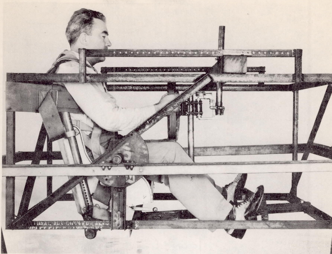
Figure 1.- Set-up for measuring push and pull forces.
