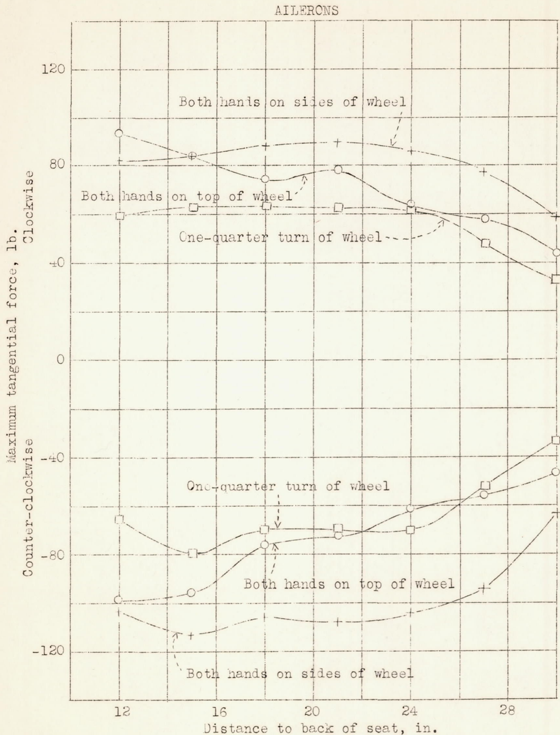
Figure 16.- Variation of tangential force with various two-hand grips, 12 inch wheel, center of wheel 14 inches above seat, pilot secure, pilot A.
