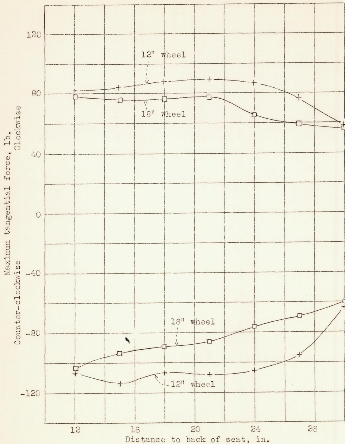
Figure 10.- Variation of tangential force with wheel diameter, 12 and 18 inch wheels, center of wheel 14 inches above seat, pilot secure, grip normal, pilot A.
