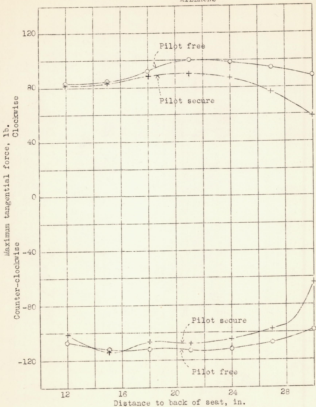
Figure 12.- Variation of tangential force with pilot free and pilot secure, 12 inch wheel, center of wheel 14 inches above seat, grip normal, pilot A.
