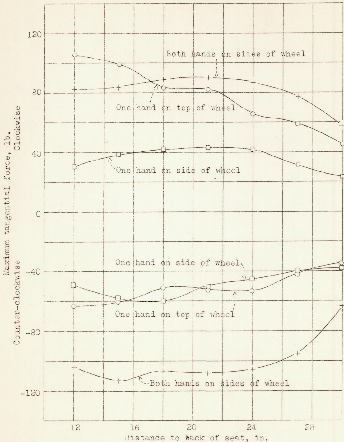
Figure 18.- Variation of tangential force with one hand (right) in two positions on wheel, with both hands, grip normal, 12 inch wheel, center of wheel 14 inches above seat, pilot secure, pilot A.
