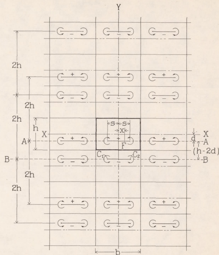
Figure 14.- Image pattern that satisfies boundary condition for closed rectangular tunnel with wing offset from center.
