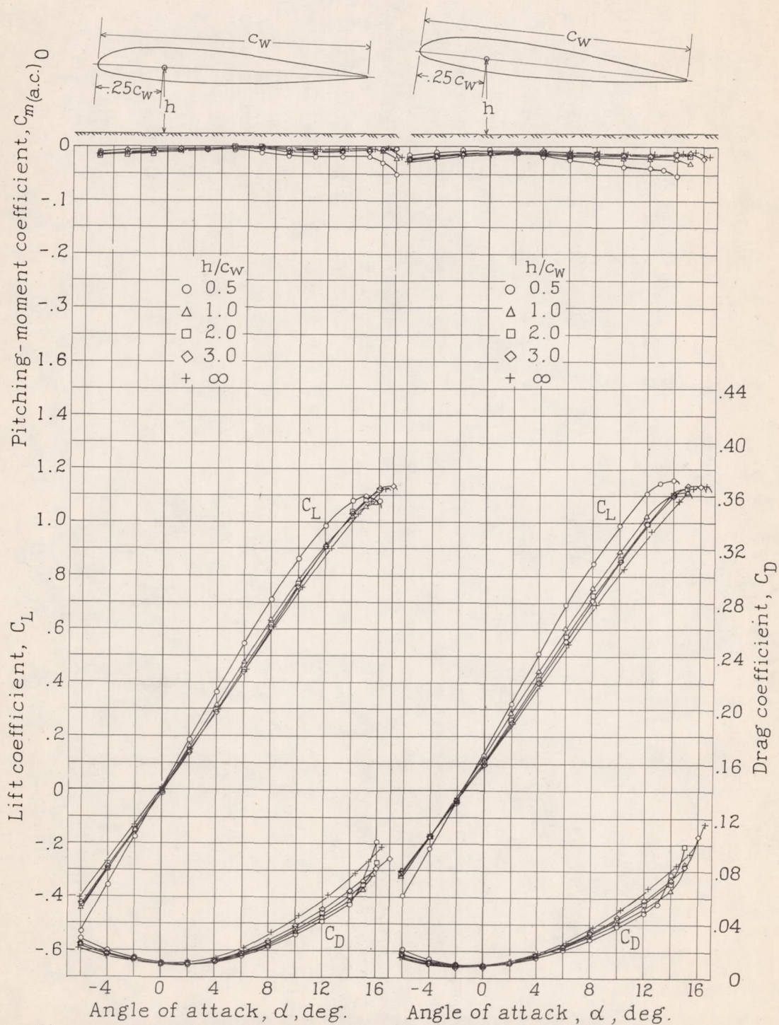
Figure 4.- Rectangular wing.
