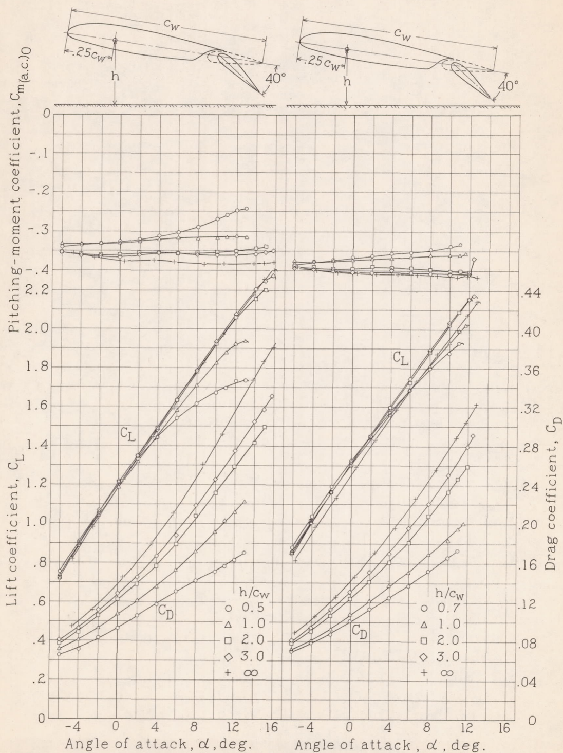
Figure 8. - Rectangular wing.
