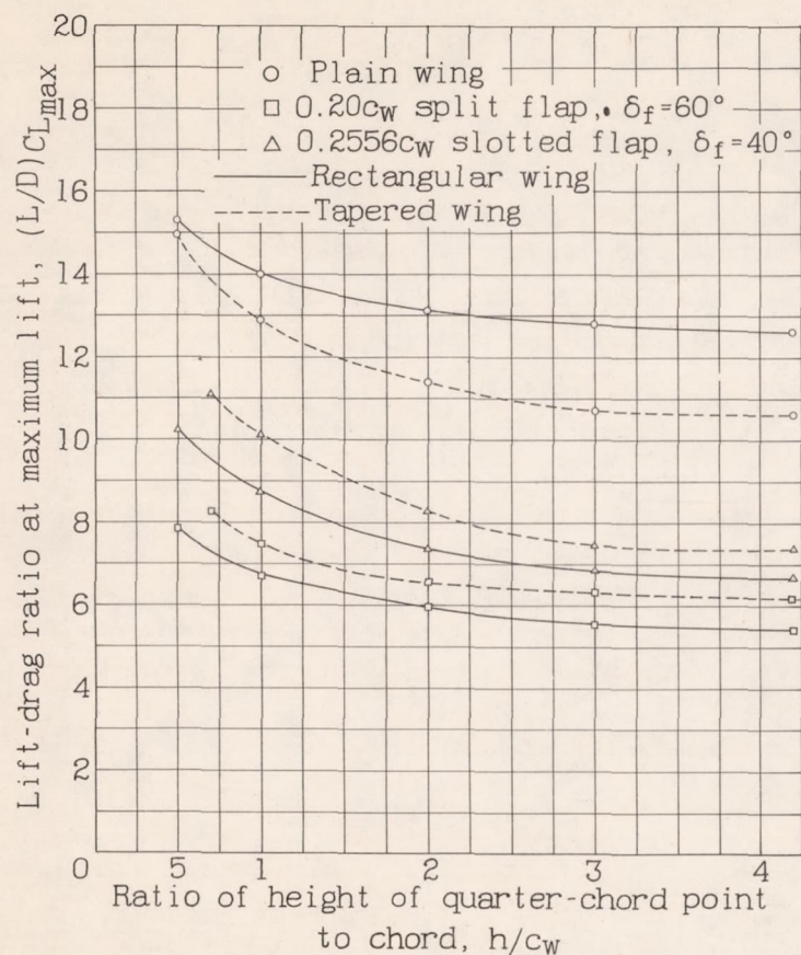
Figure 12.- Effect of ground proximity on lift-drag ratios at maximum lift of N.A.C.A. 23012 wings.
