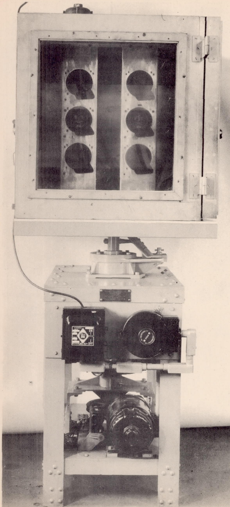
Figure 7.- Sperry scorsby used to sub- ject gyroscopic instru- ments to a combined pitch- roll-and yaw motion. Two instruments are shown in- stalled, in the temperature chamber which is mounted on the scorsby table.
