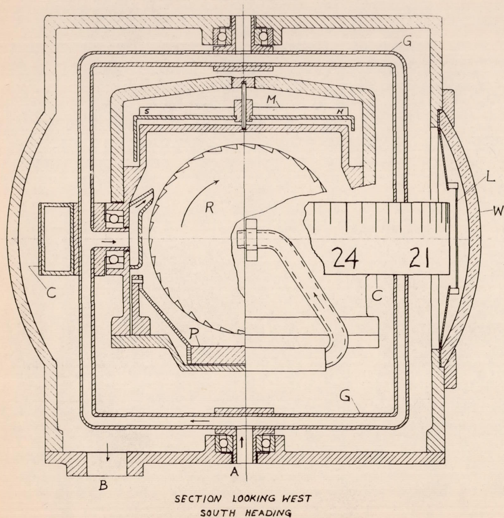
Figure 10.- Diagram of gyromagnetic compass.
