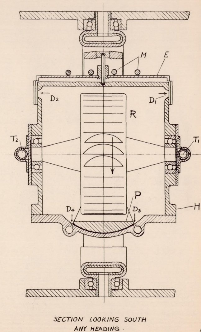
Figure 10.- Diagram of gyromagnetic compass.
