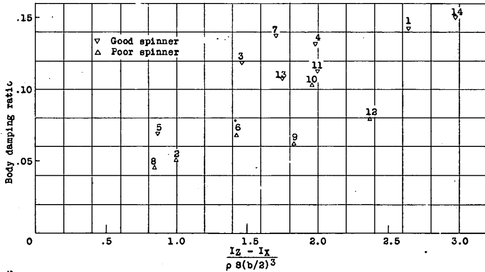
Figure 6.- Variation of body damping ratio with inertia pitching parameter for 14 American monoplanes.
