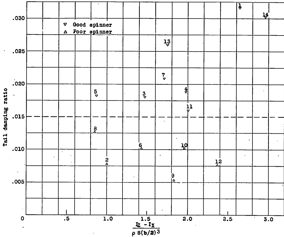
Figure 8.- Variation of tail damping ratio with inertia pitching parameter for 14 American monoplanes.
