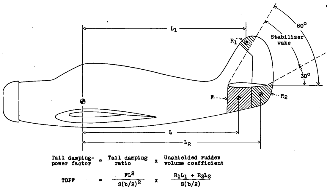
Figure 9.- Method of computing tail damping-power factor.
