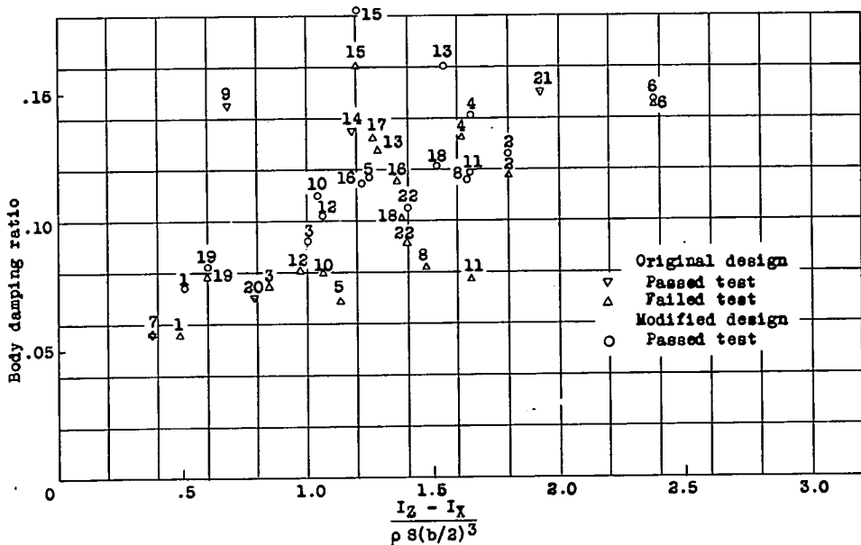
Figure 4.- Variation of body damping ratio with inertia pitching parameter for 22 British monoplanes (From reference 1).
