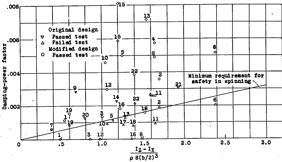
Figure 2.- Variation of damping-power factor with inertia pitching parameter for 22 British monoplanes (From reference 1).
