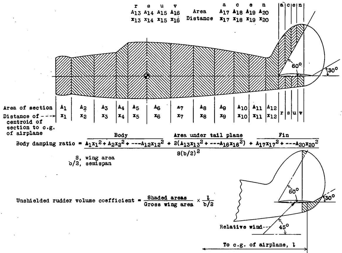
Figure 1.- Method of computation of damping coefficients.
