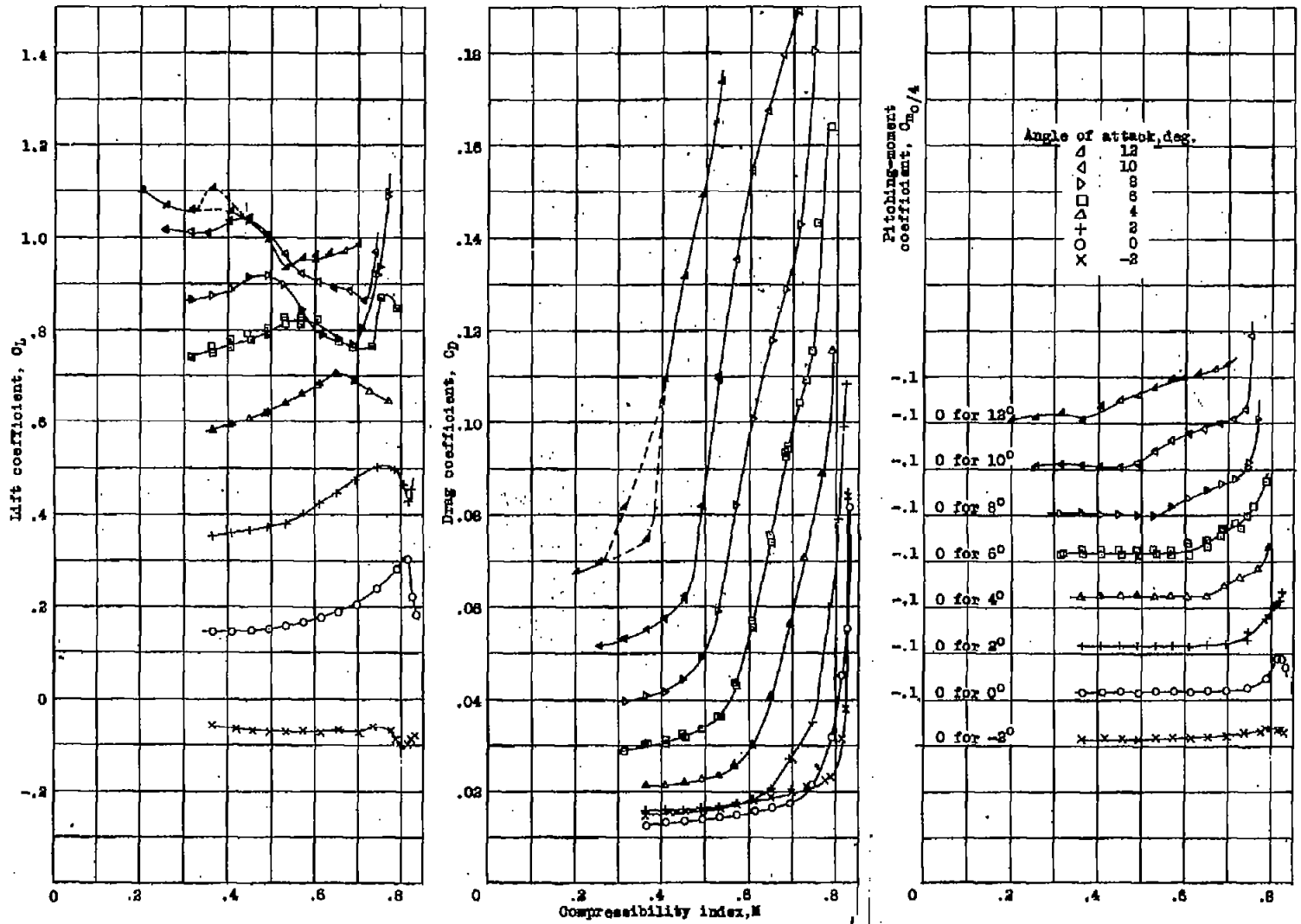
Figure 2.- Effect of compressibility on the aerodynamic characteristics of the N-55 airfoil.
