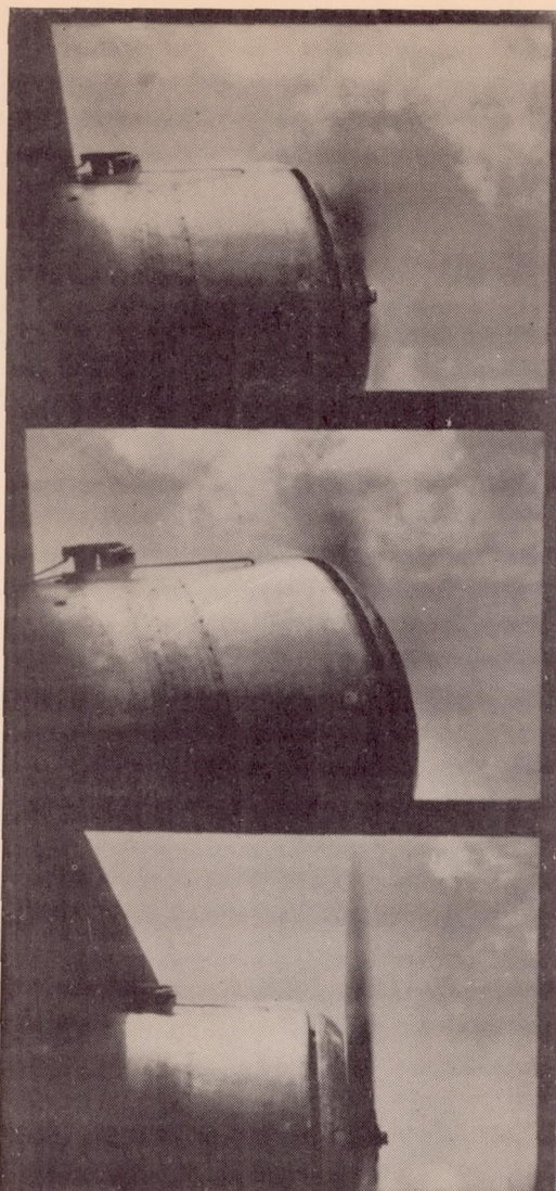
Figure 8.- Smoke flow coming out of the slot. Nose-slot cowling 3-B.
