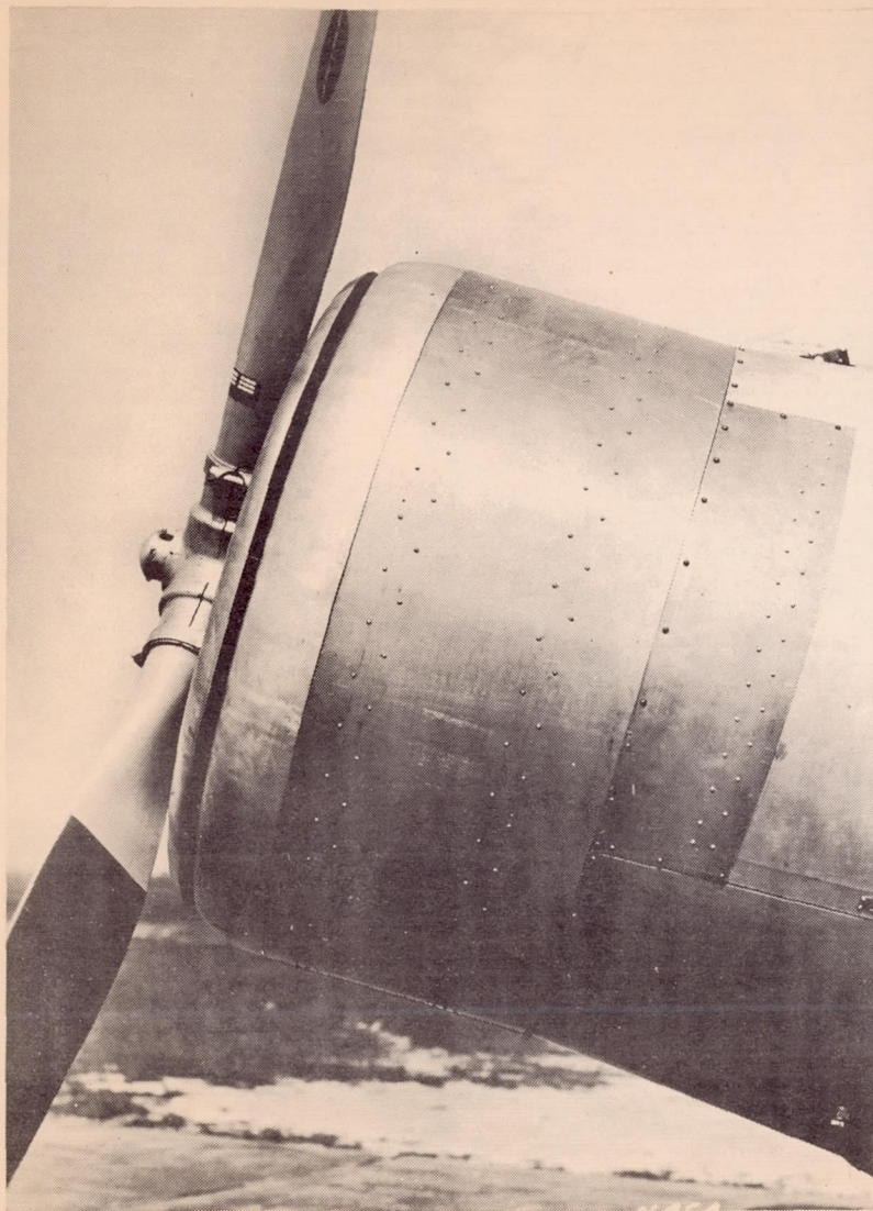
Figure 4.- Close-up of nose-slot cowling 1.
