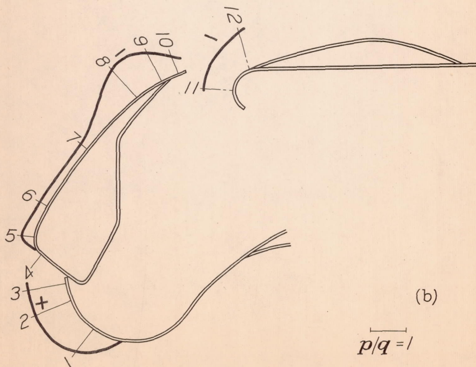
Figures 11a, 11b.- Pressure distribution over nose-slot cowl 3-C. Level flight. (a) High-speed position. (b) Low-speed position.
