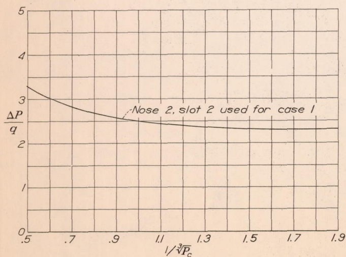
Figure 17.- Variation of \Delta P/q with 1/\sqrt{P_c} (reference 2).
