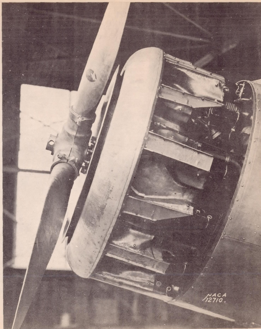
Figure 5c.- Close-up of nose-slot cowling 2. Ring removed to show internal arrangement.
