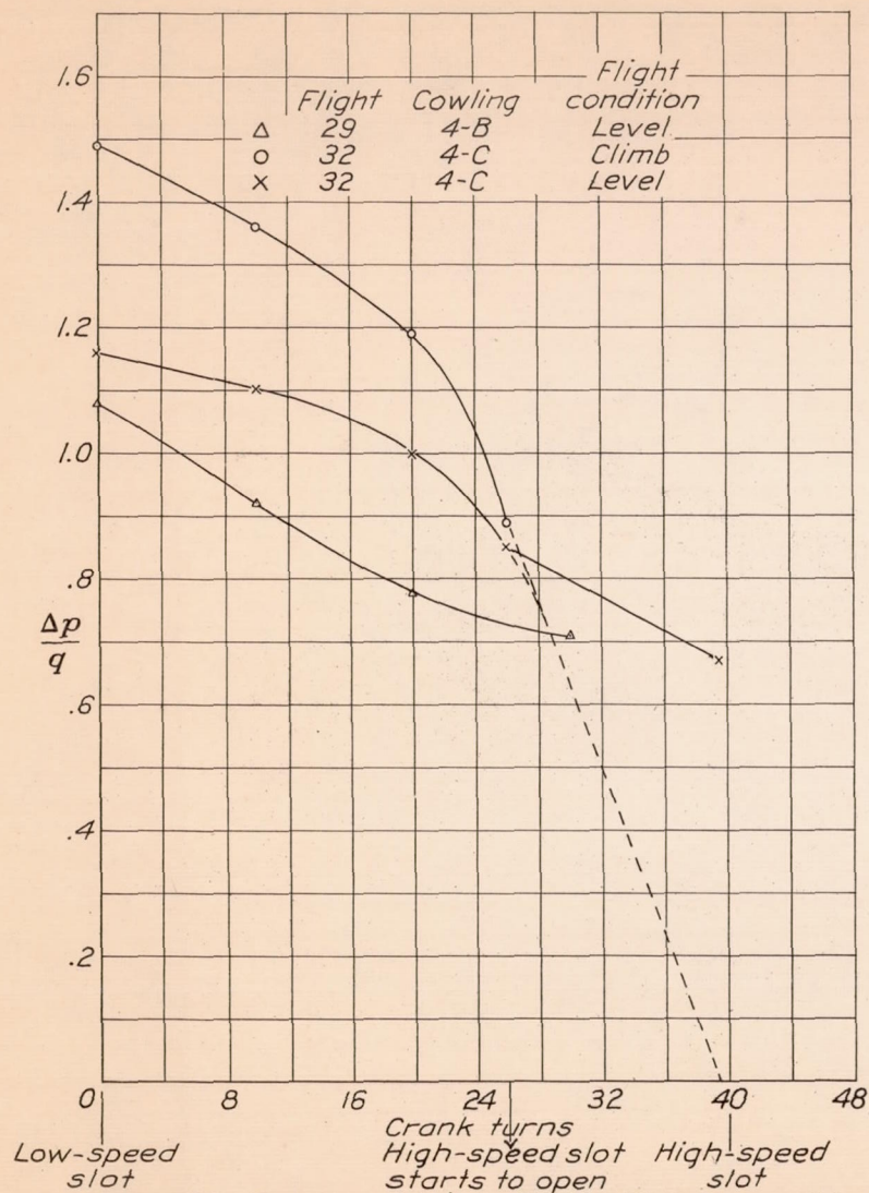
Figure 15.- Variation of \Delta p/q in flight with cowling position for nose-slot cowlings 4-B and 4-C.
