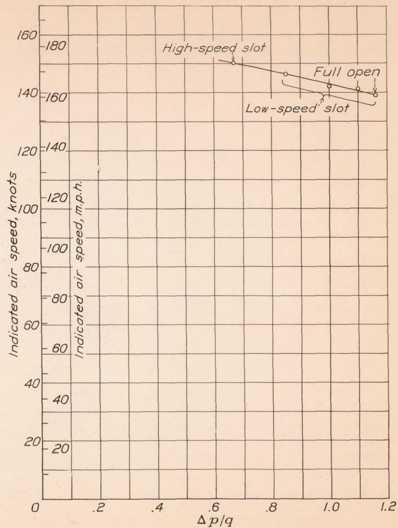
Figure 16.- Variation of air speed with \Delta p/q for the constant-power level-flight condition as obtained with nose-slot cowling 4-C.
