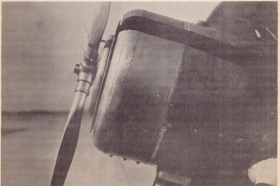
Figure 14b.- Side view of nose-slot cowling 4-A. High-speed position; round-edge disk in place.
