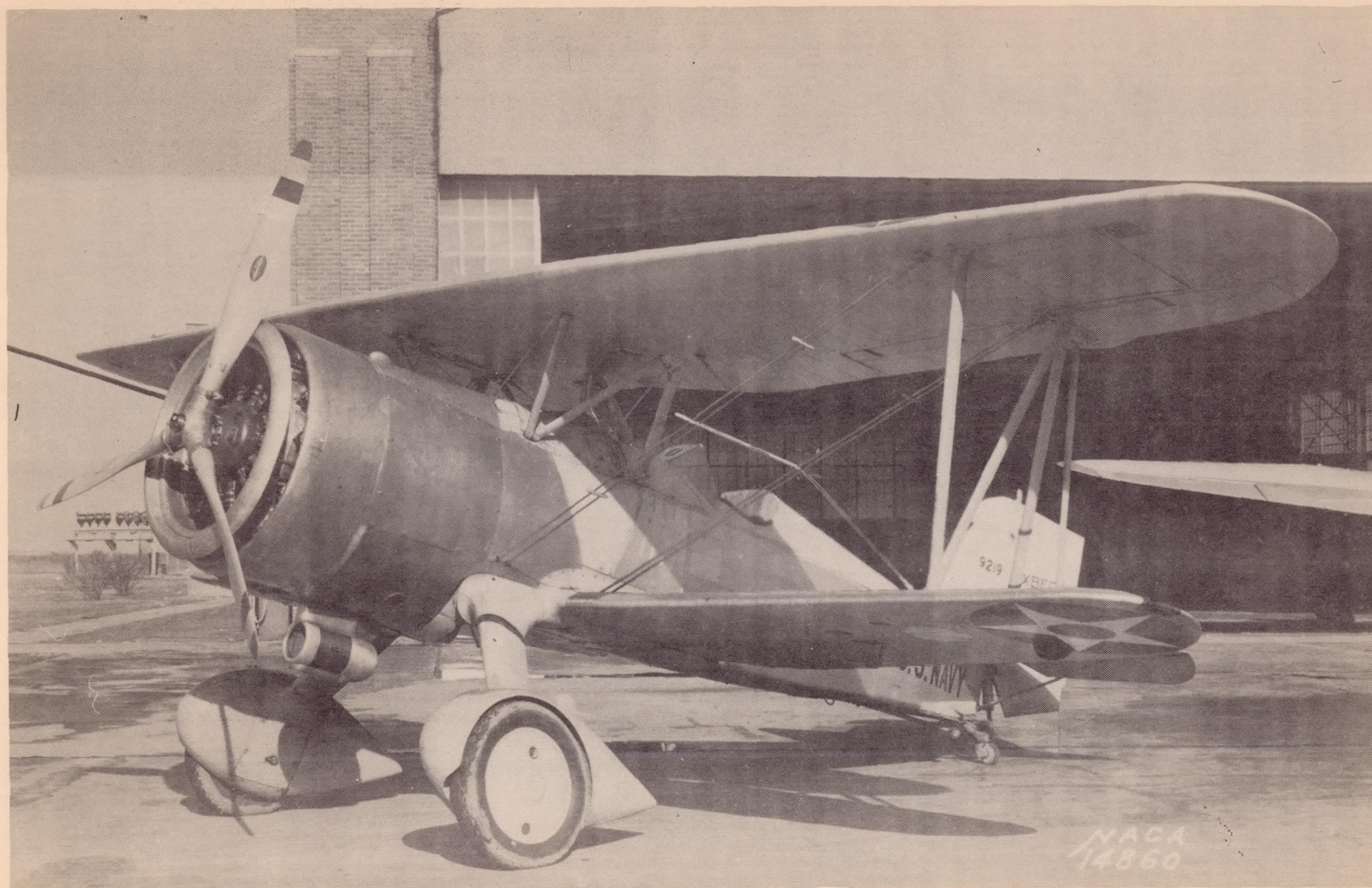
Figure 12.- The BFC-1 airplane equipped with nose-slot cowling 4-A in the low-speed position.
