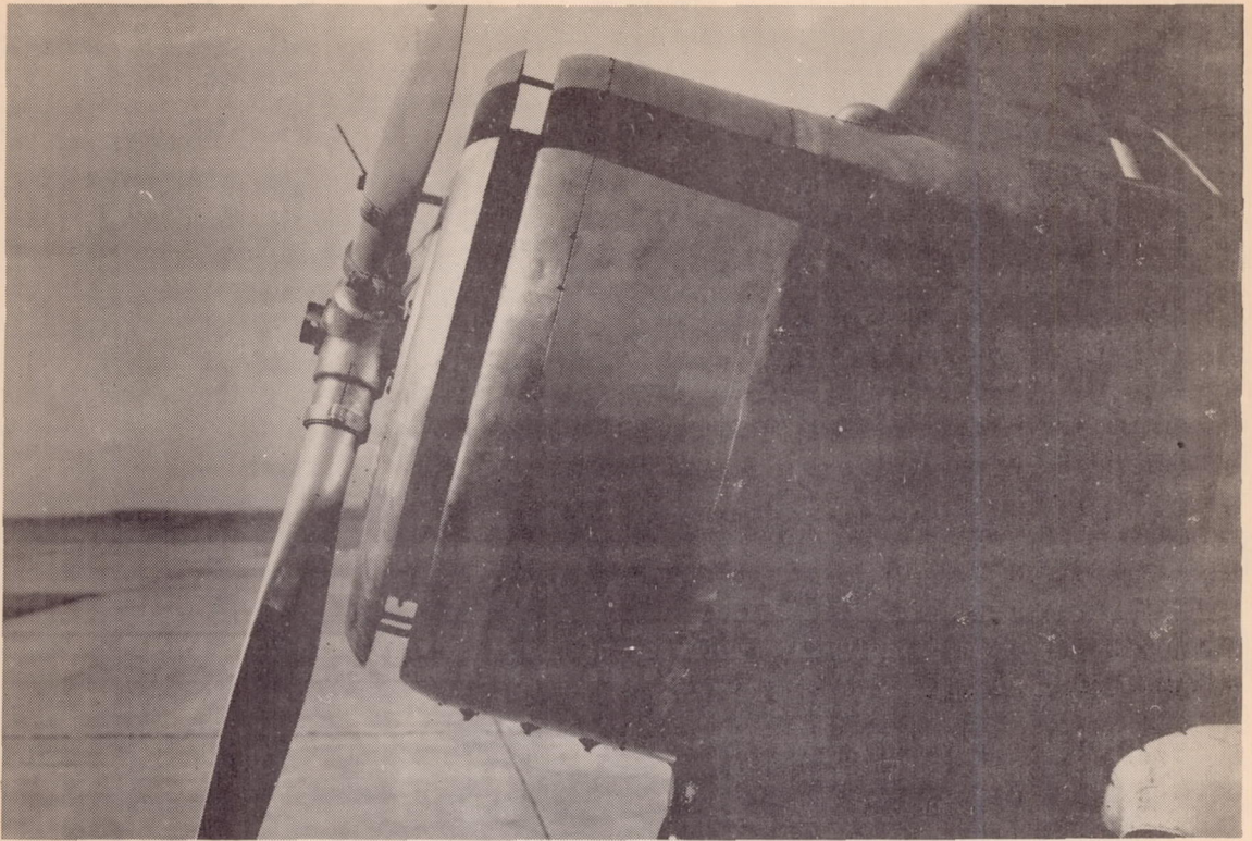
Figure 14a.- Side view of nose-slot cowling 4-A. Low speed position.
