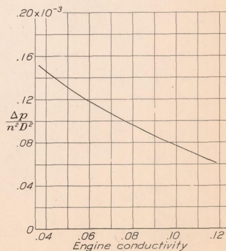
Figure 19.- Variation of \Delta p/n^2 D^2 with engine conductivity (reference 2).
