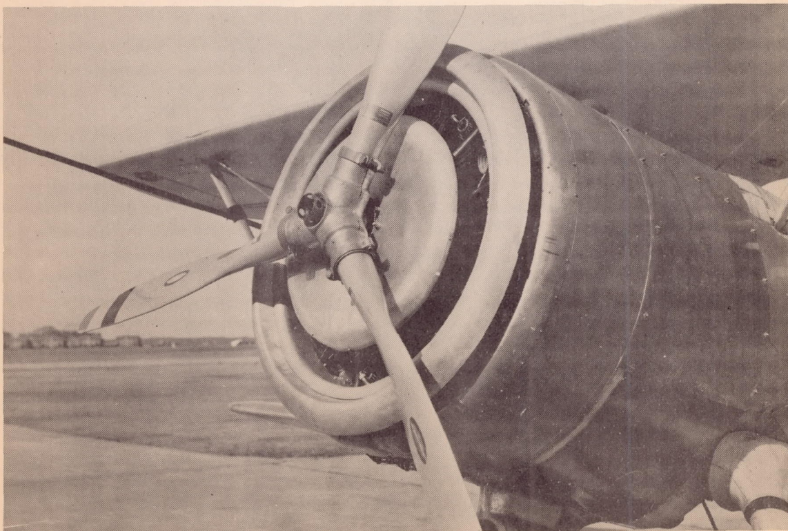
Figure 13b.- Close-up of nose-slot cowling 4-A in the low-speed position. Round-edge disk in place.
