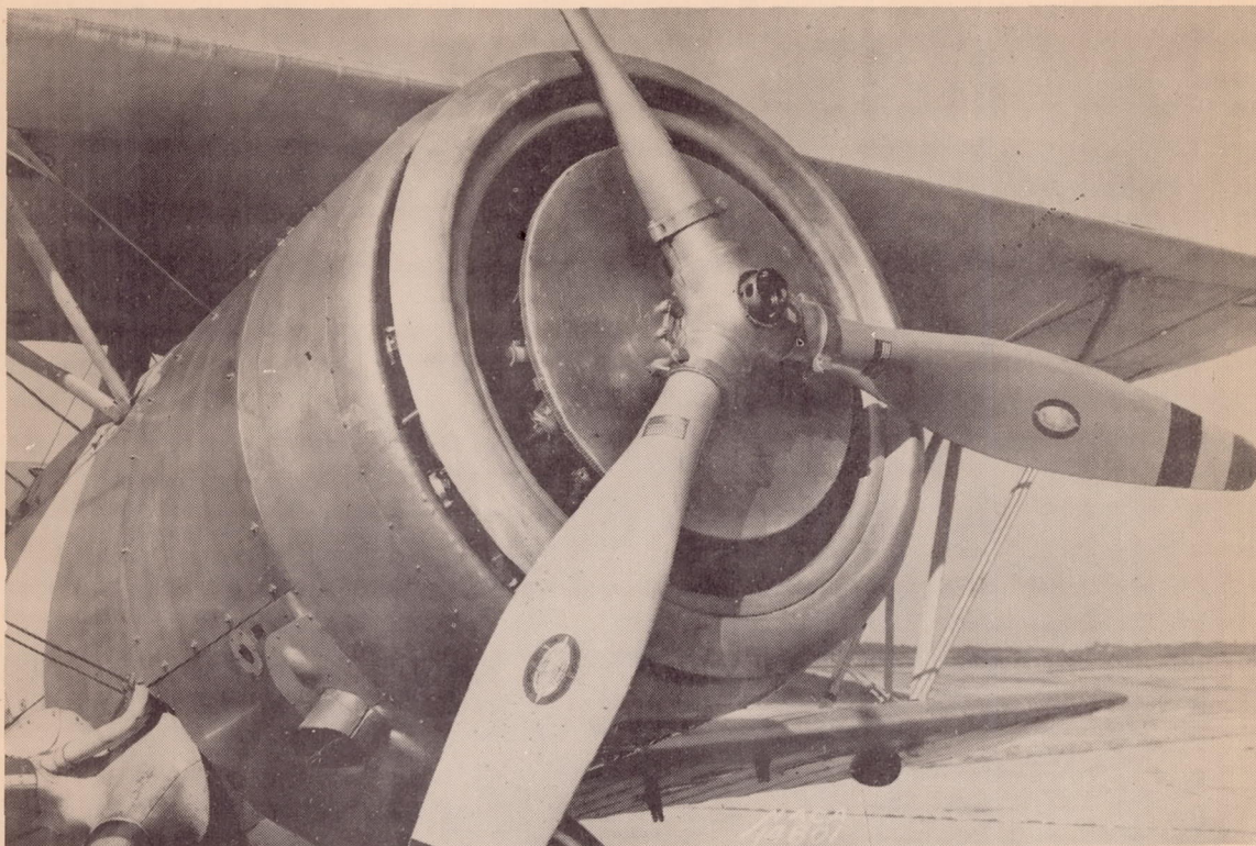
Figure 13a.- Close-up of nose-slot cowling 4-A in the low-speed position. Square-edge disk in place.
