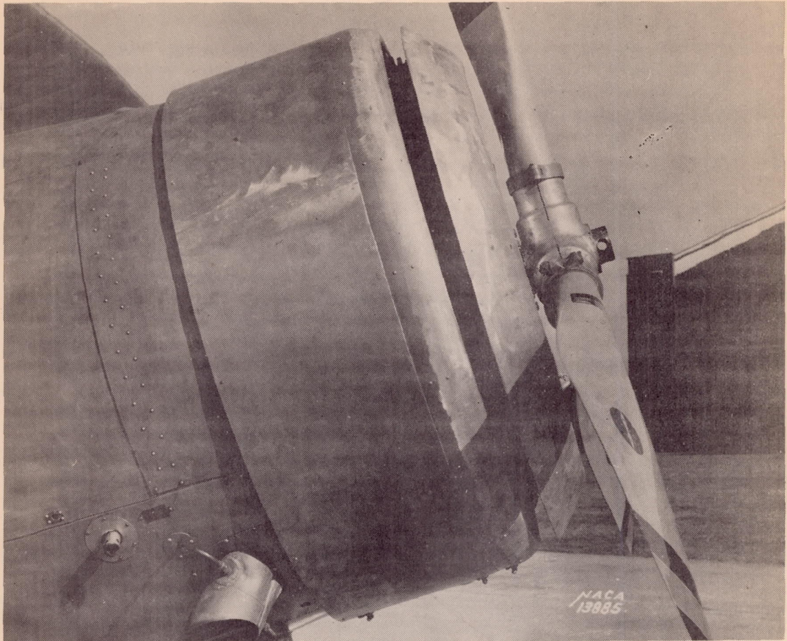
Figure 6.- Close-up of the nose-slot cowling 3-F in the low-speed position.
