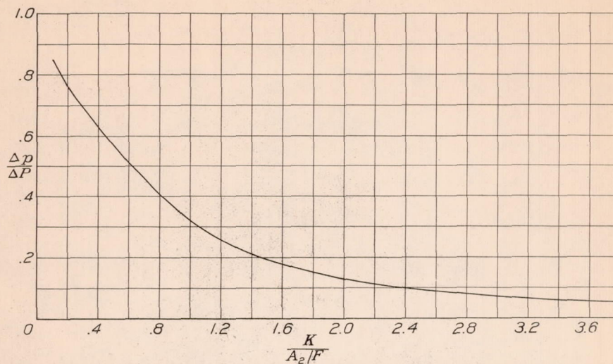
Figure 18.- Variation of \Delta p/\Delta P with \frac{K}{A_2/F} (reference 2).
