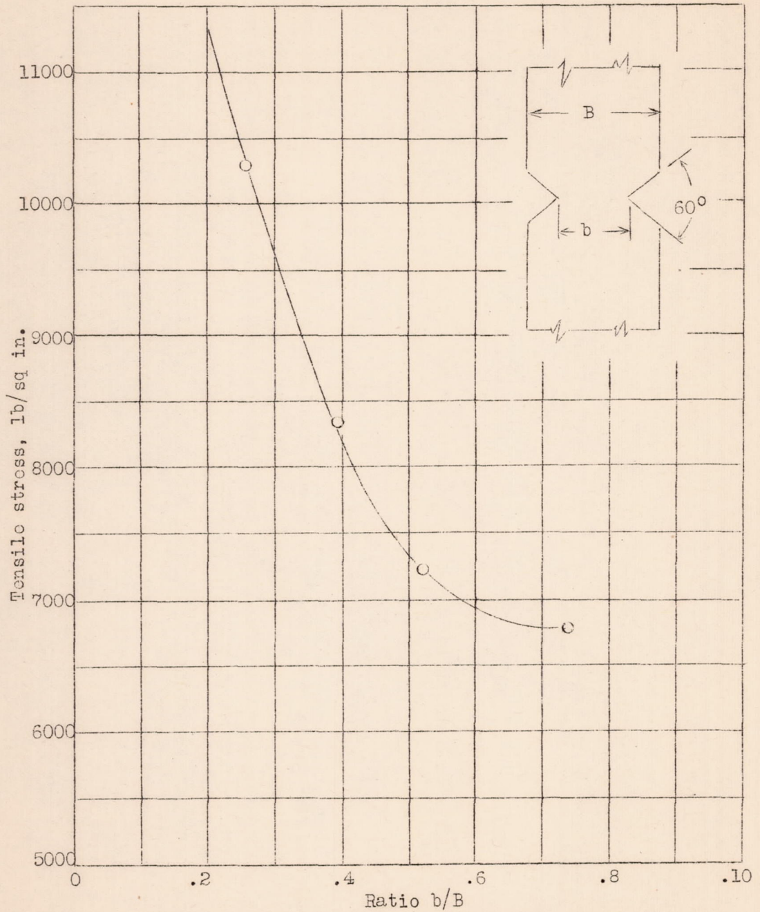
Figure 11.- Notch-sensitivity tests of fabric-base synthetic resin.
