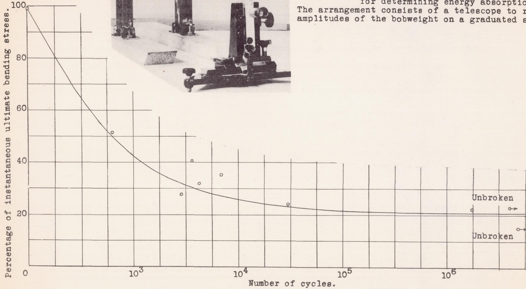
Figure 9.— Dynamic-endurance tests of compound 1840.
