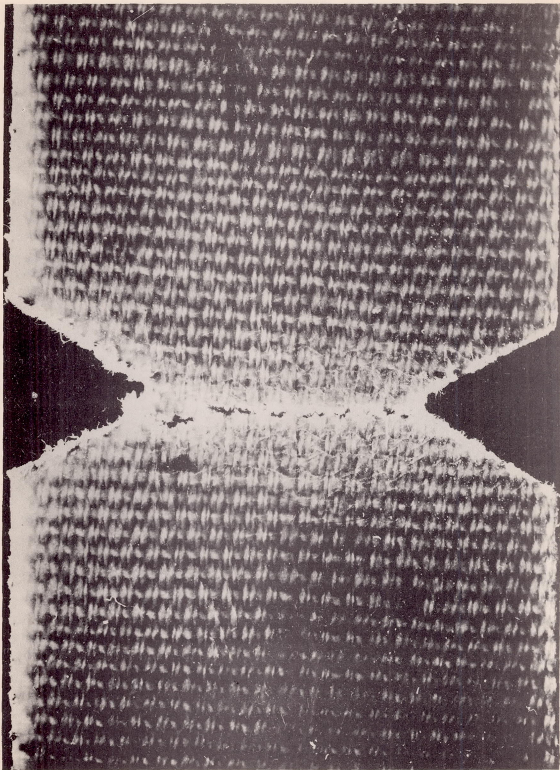
Figure 14. - Photomicrograph of bearing bolt in synthetic resin, fabric base.
