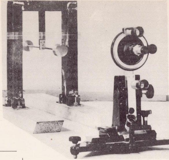
Figure 10.— Free torsional-oscillation system for determining energy absorption. The arrangement consists of a telescope to read amplitudes of the bobweight on a graduated scale.
