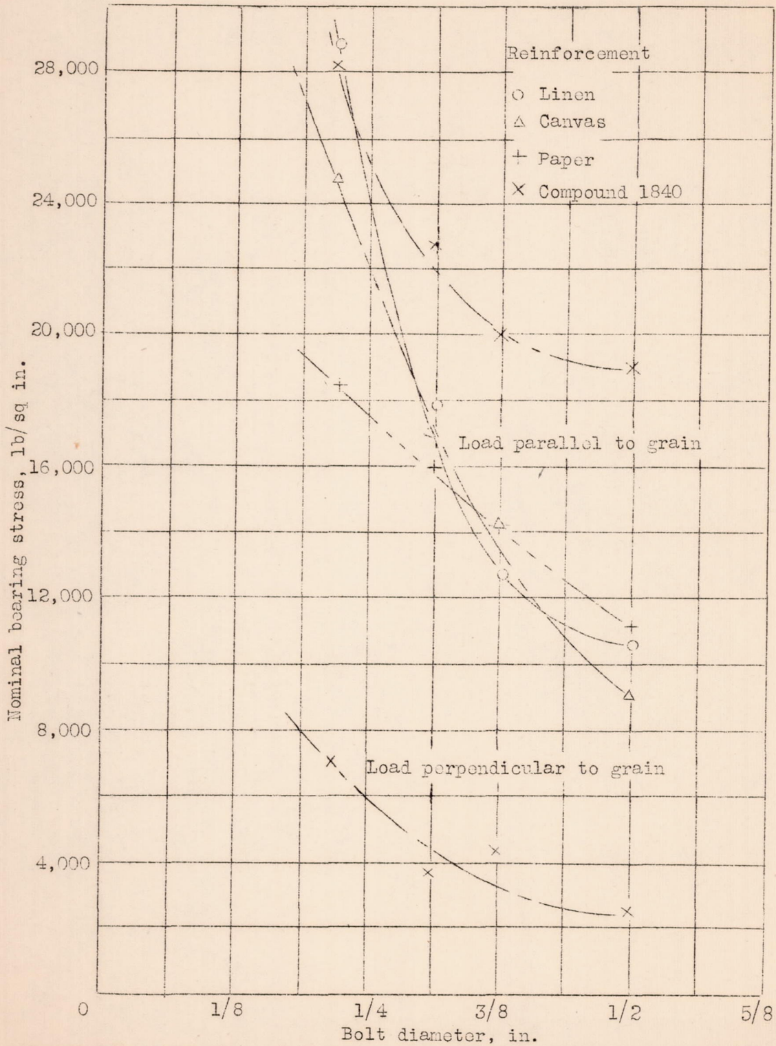
Figure 13.- Variation of bearing stress with bolt diameter in bearing tests for reinforced synthetic resin.
