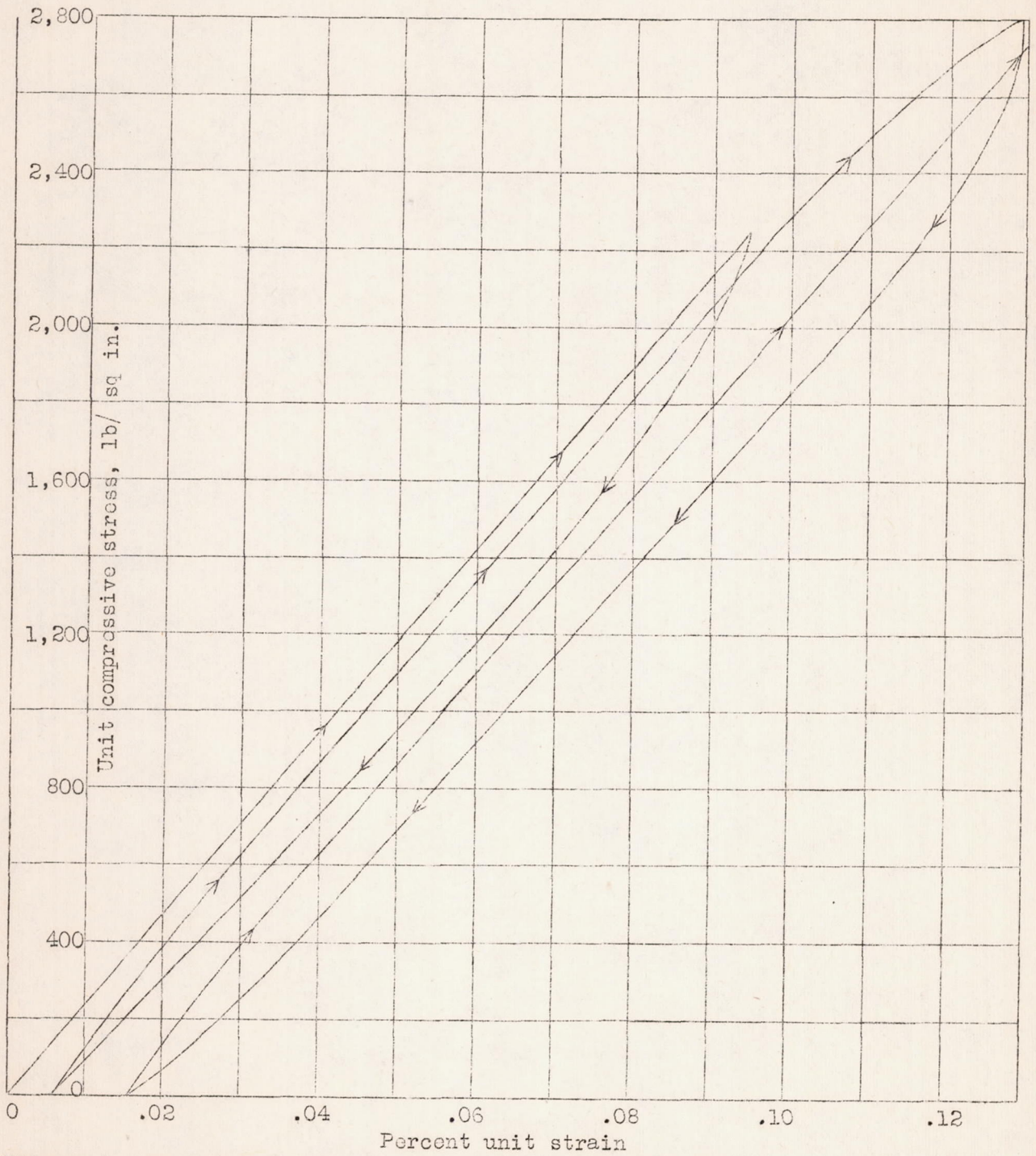
Figure 4.- Repeated loading in compression on a rod of synthetic resin with linen base.
