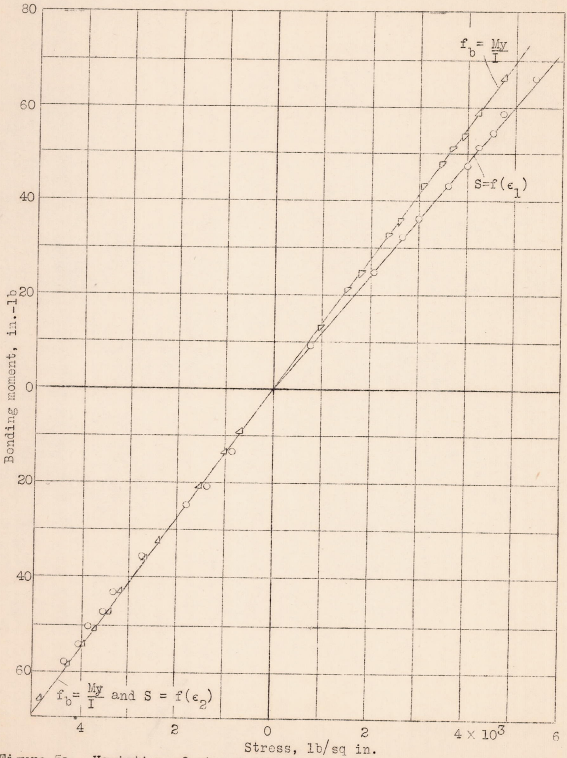
Figure 5a.- Variation of stress with bending moment for synthetic resin, paper base.
