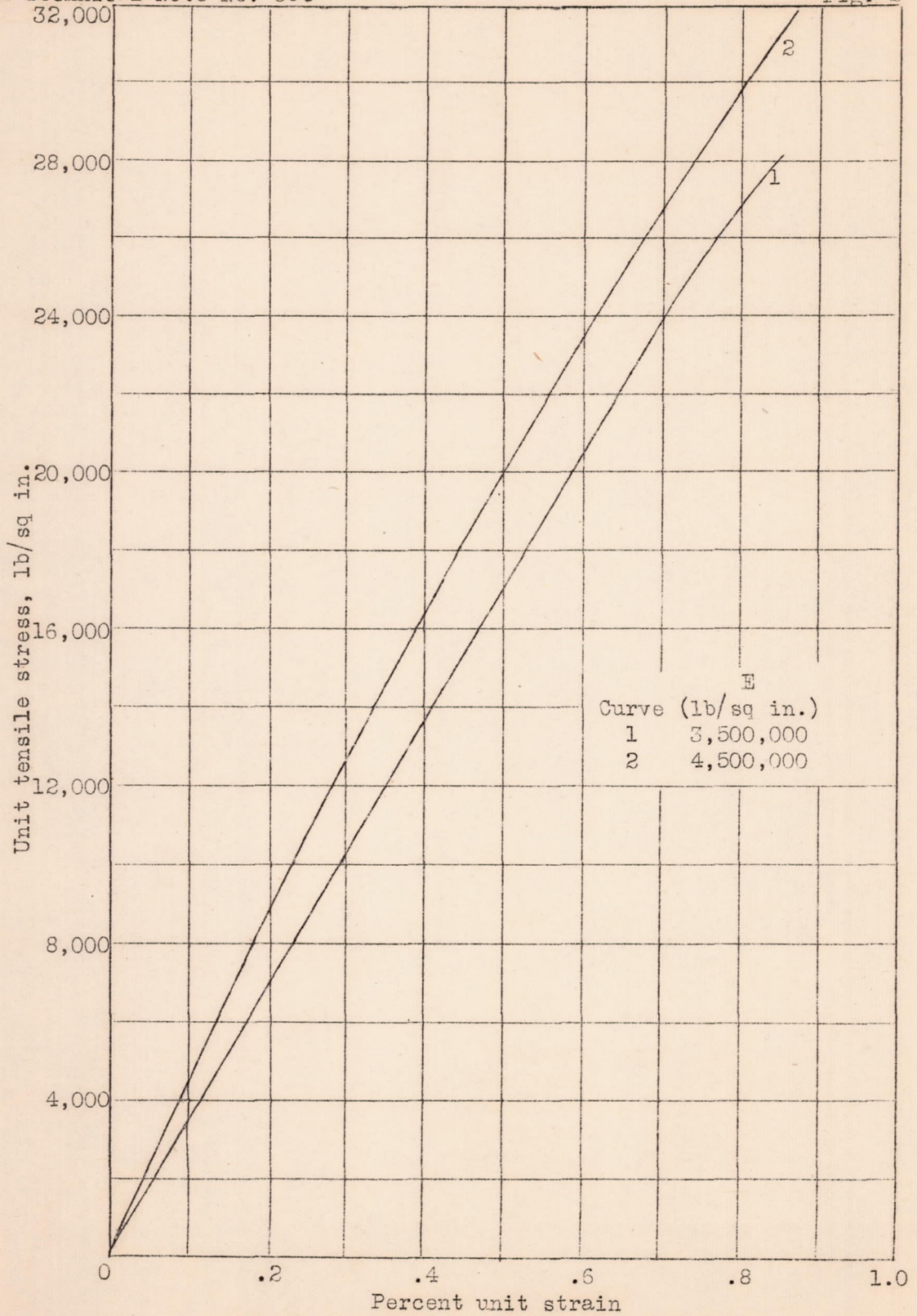
Figure 2.- Compound 1840 in tension.
