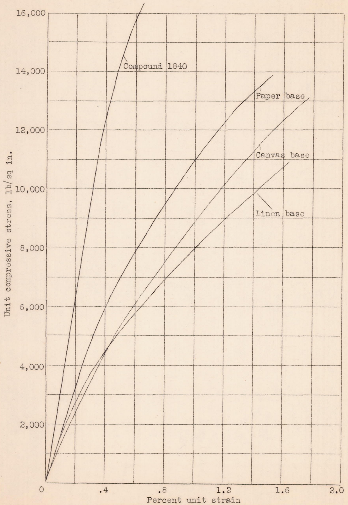
Figure 3.- Properties in compression.
