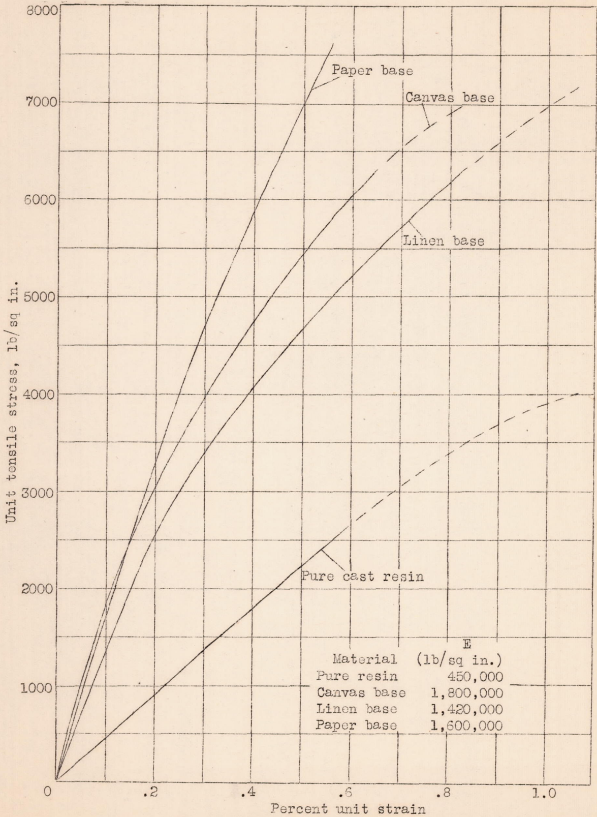
Figure 1.- Synthetic resin in tension.
