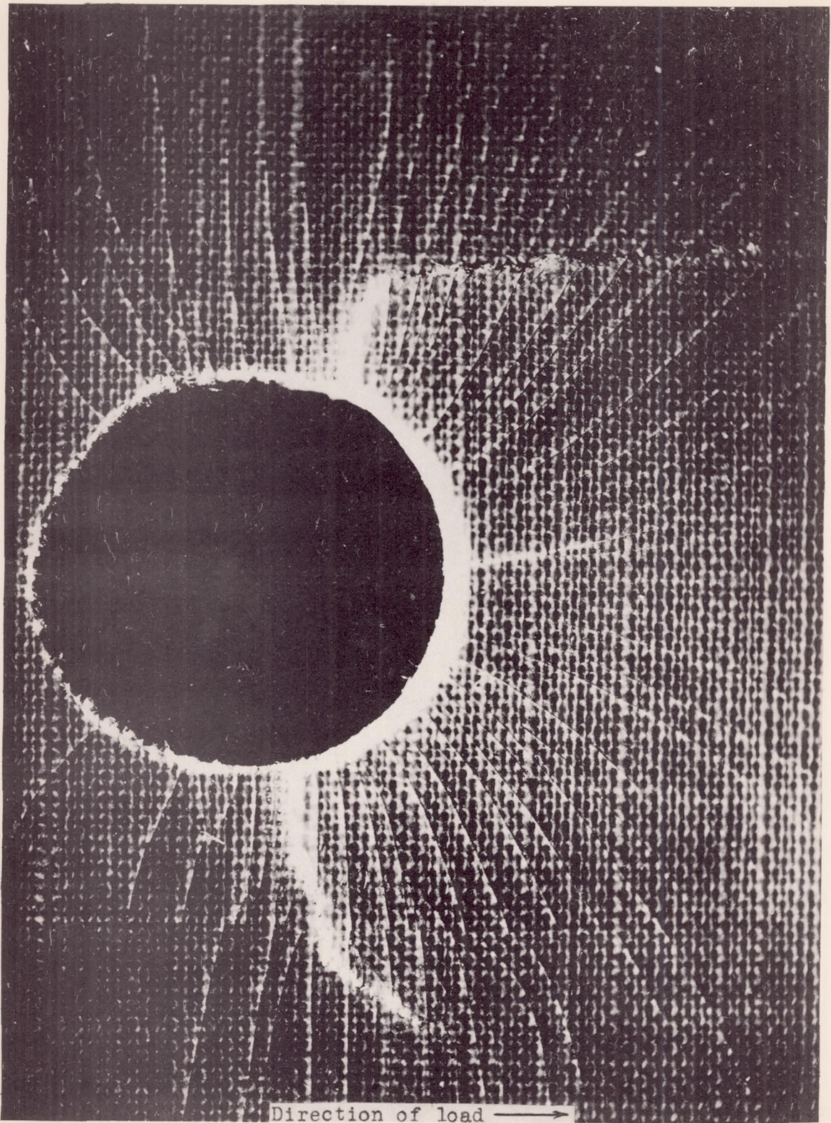
Figure 12. - Photomicrograph of notched specimen of synthetic resin.
