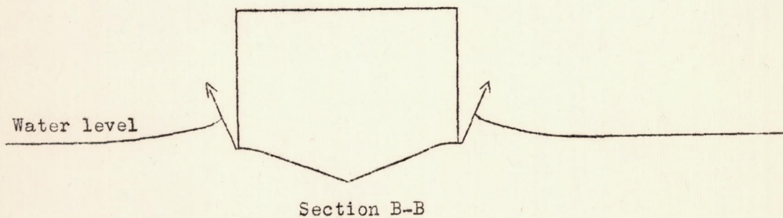
Figure 18.- Diagrams of spray formation at two parts of a typical forebody.
