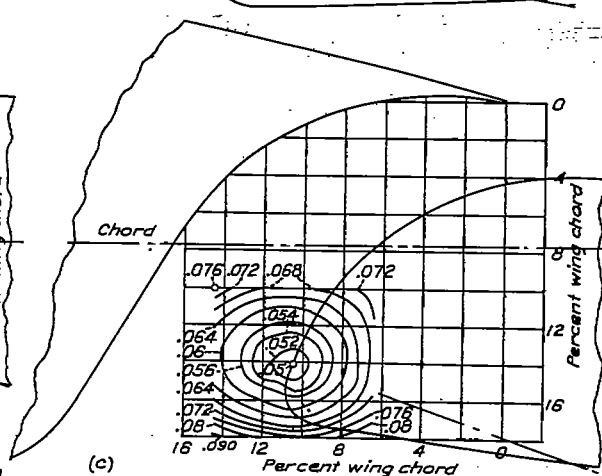
Figure 11.- Contours of flap location for c_{d0} . The 0.40c slotted flap 1-b.
