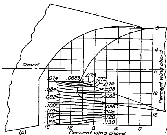
Figure 10.- Contours of flap location for c_{d0} . The 0.40c slotted flap 1-a.
