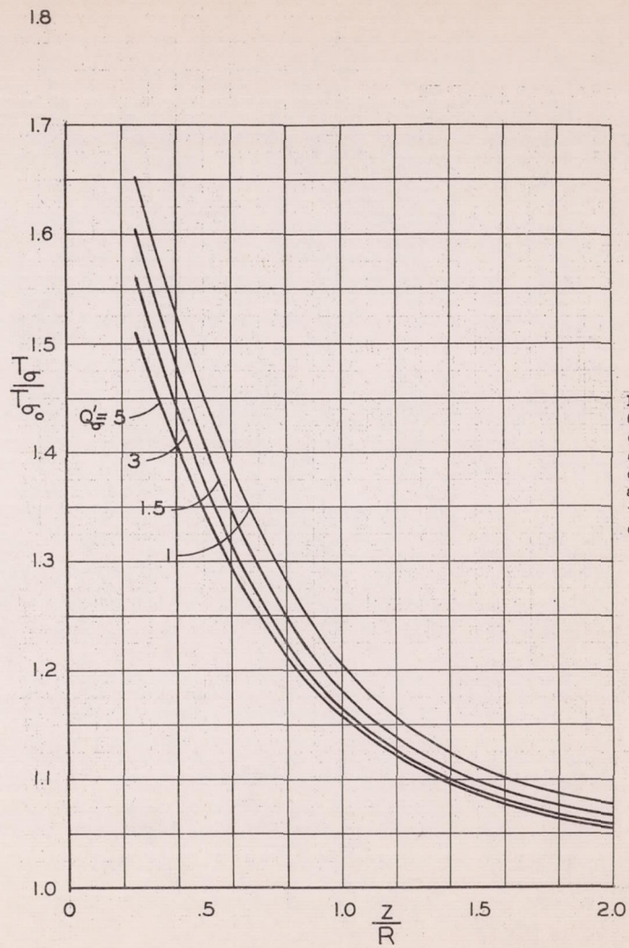
Fig. 12. Ground Effect on the Landing of a Helicopter. ( q_{\sigma}^i = 3 )
