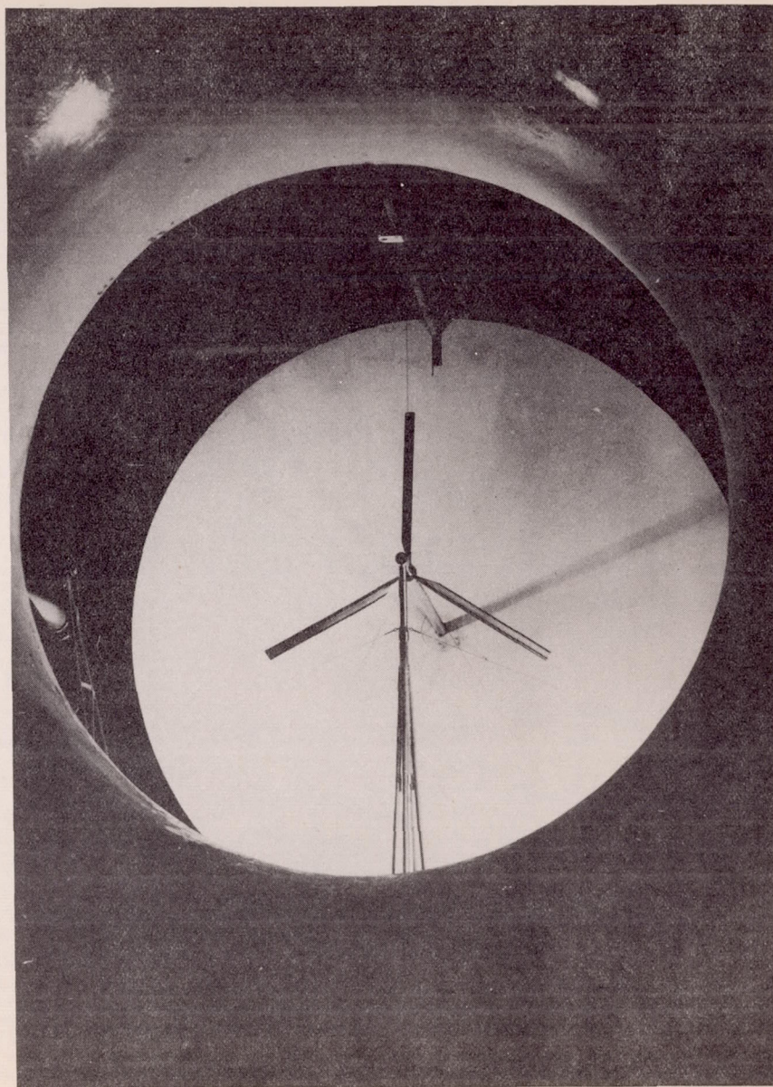
Figure 9.- Three-bladed rotor model and ground plane viewed from tunnel entrance cone.
