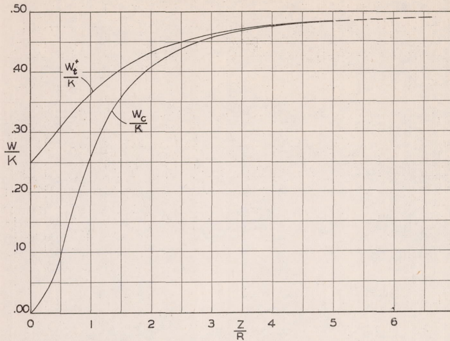
Figure 2.- Induced velocity variation. with Z/R
