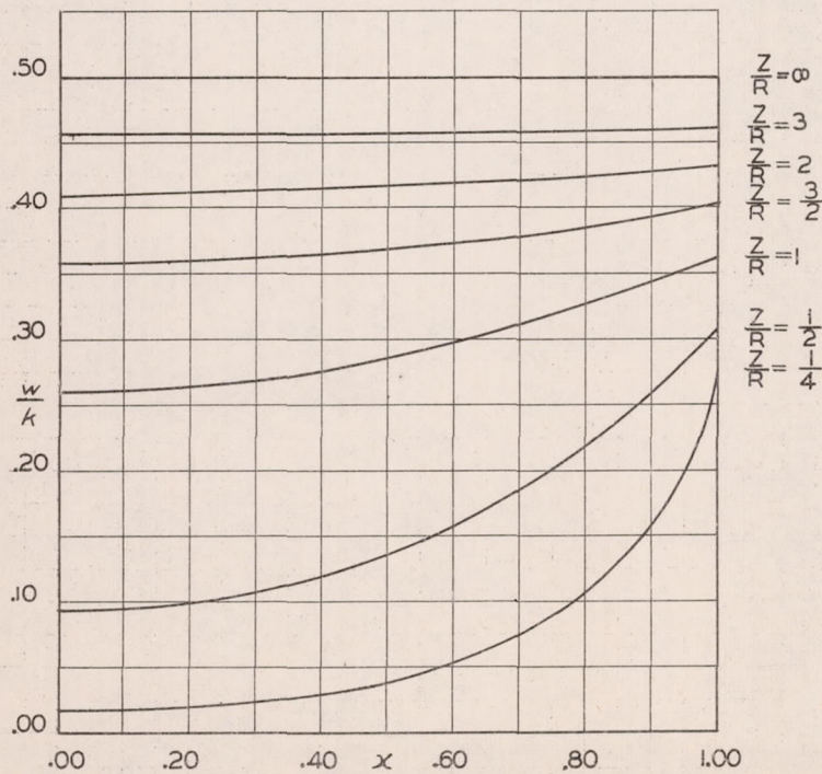
Figure 5.- Induced velocity distribution along rotor blade.
